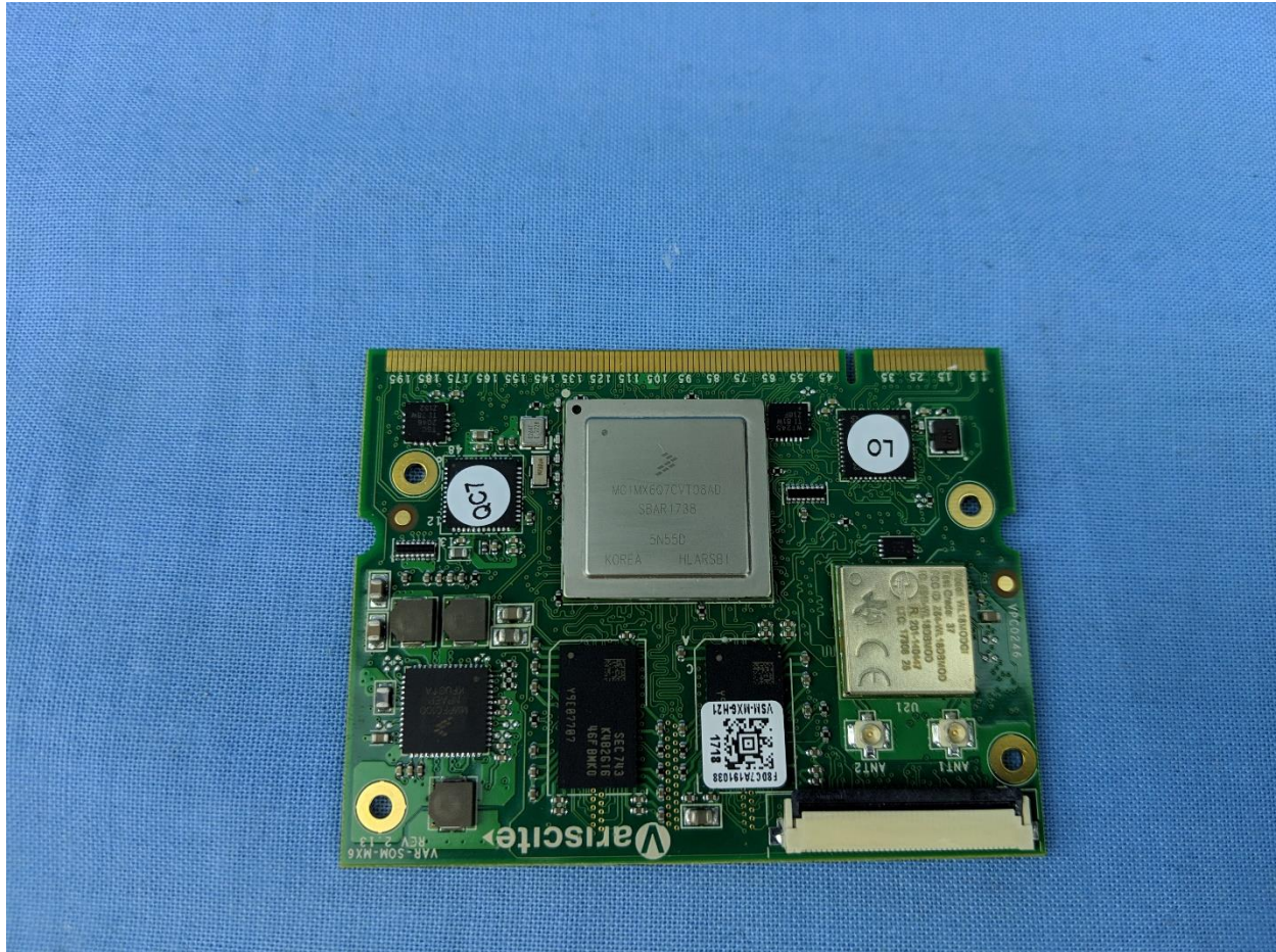
Main Board Top no Heatsink
