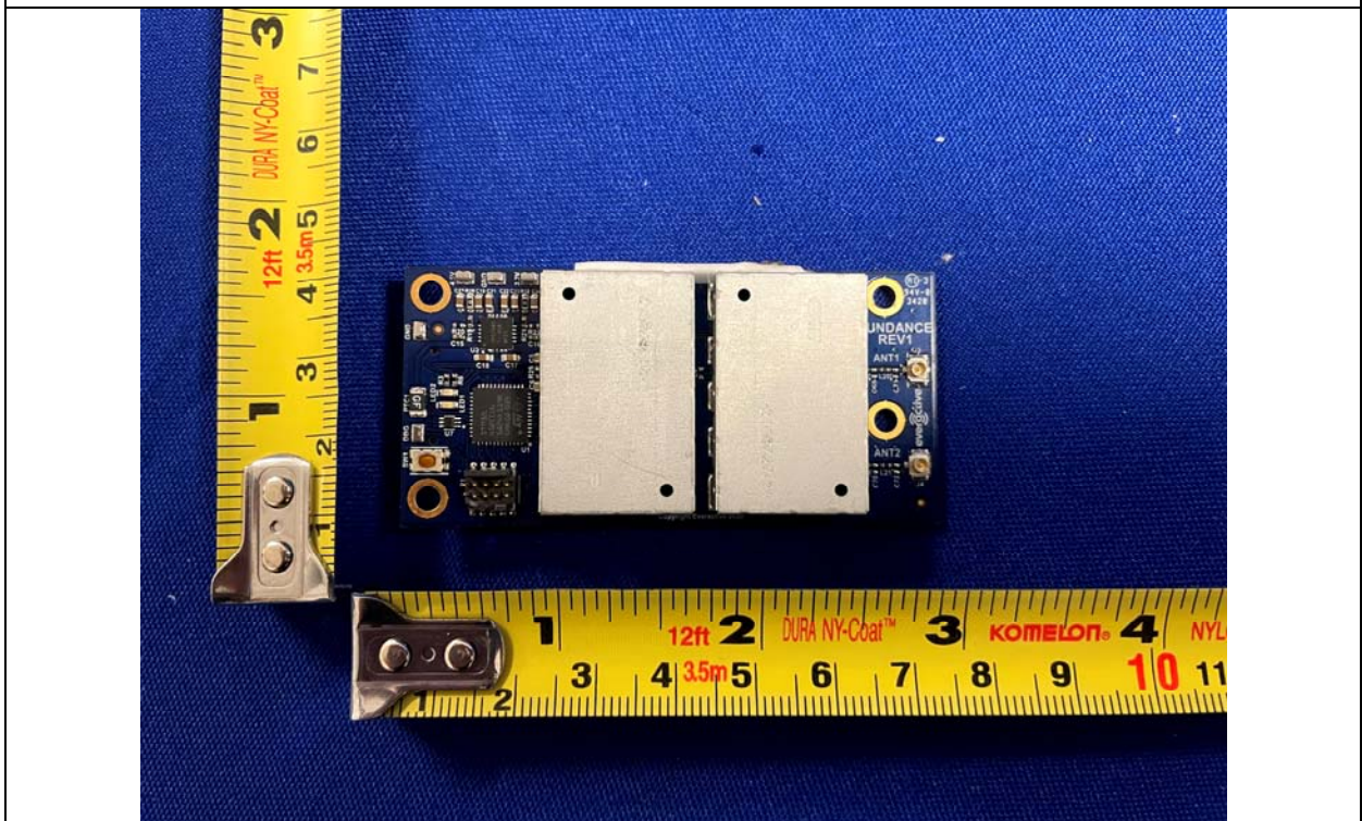
Remove Flexible EMI/ Microwave Absorber View
