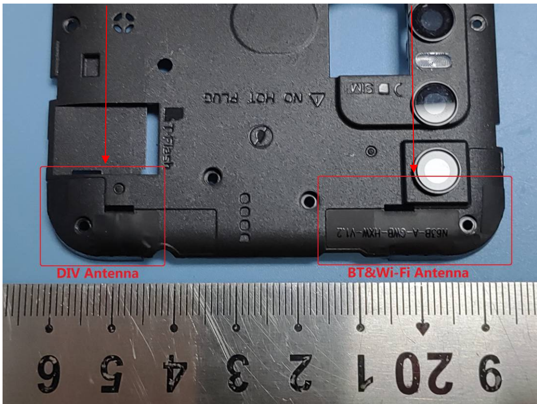
DIV Antenna
