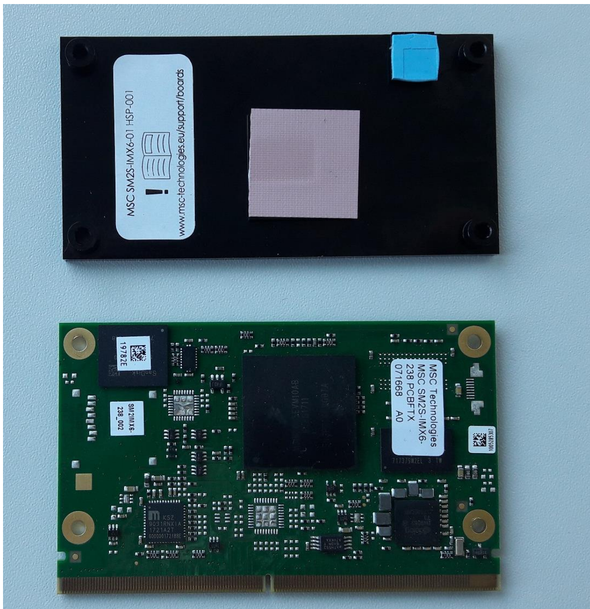
CPU-Modul Top view with heatspreader and thermal pads
