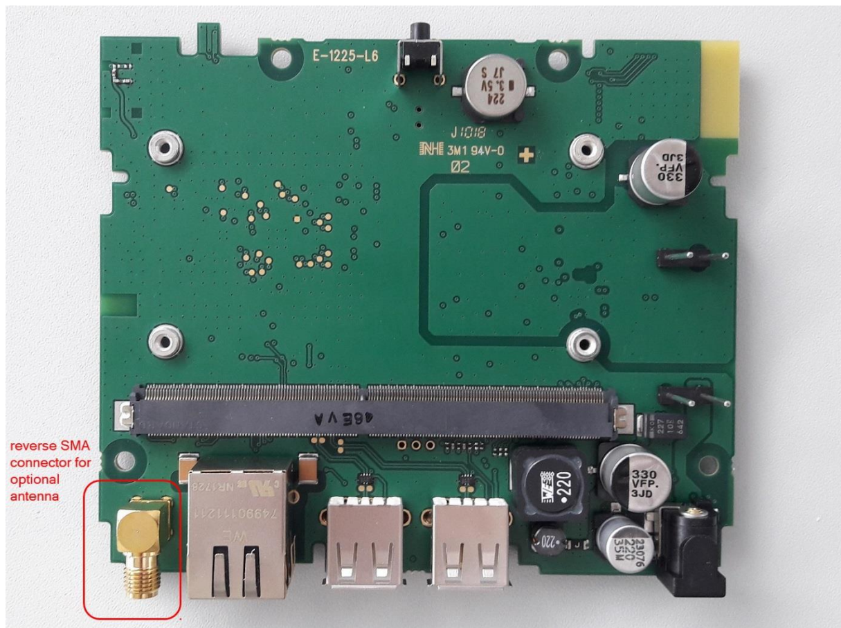
Bottom view without CPU-module and heatsreader
