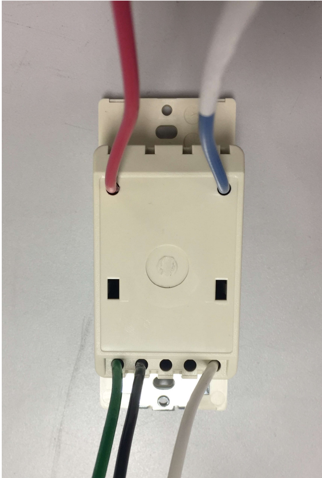
3 wire dimmer – Rear
