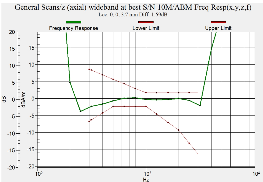
Figure C.6 Frequency Response of LTE B5
