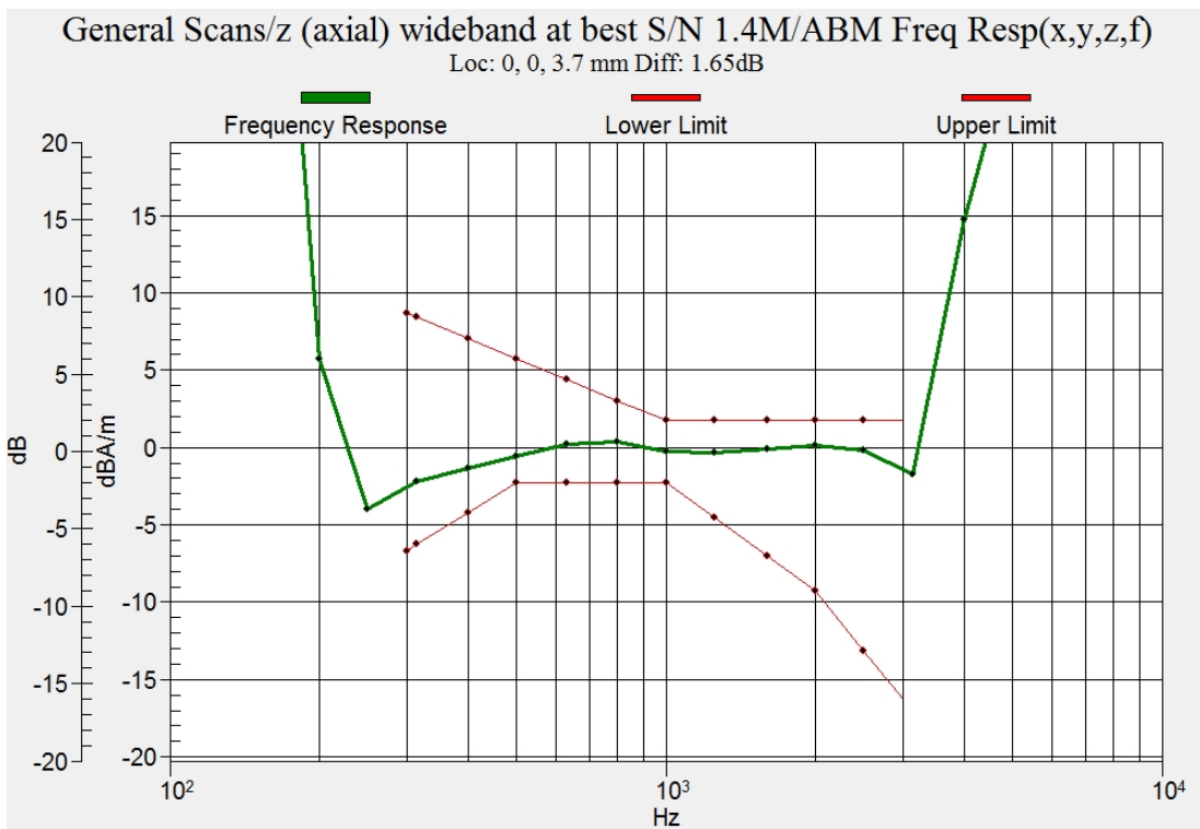
Figure C.4 Frequency Response of LTE B2 1.4M
