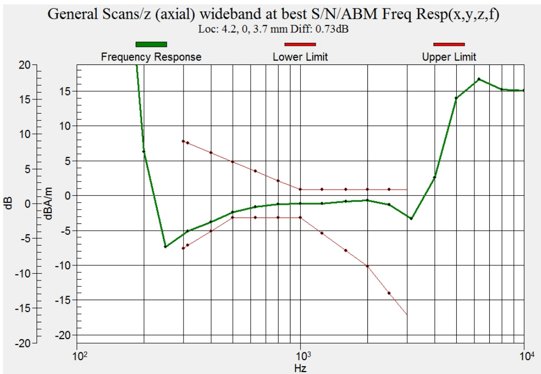
Figure C.2 Frequency Response of WCDMA 1900
