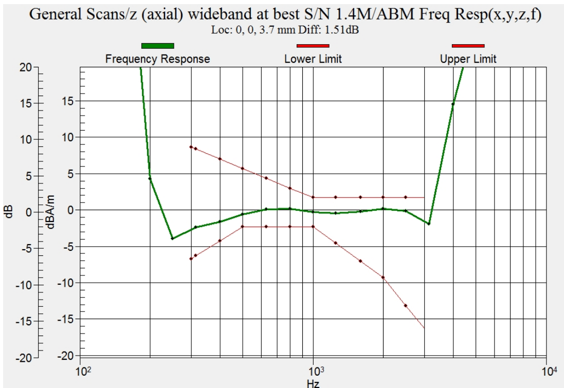
Figure C.12 Frequency Response of LTE B66 1.4M
