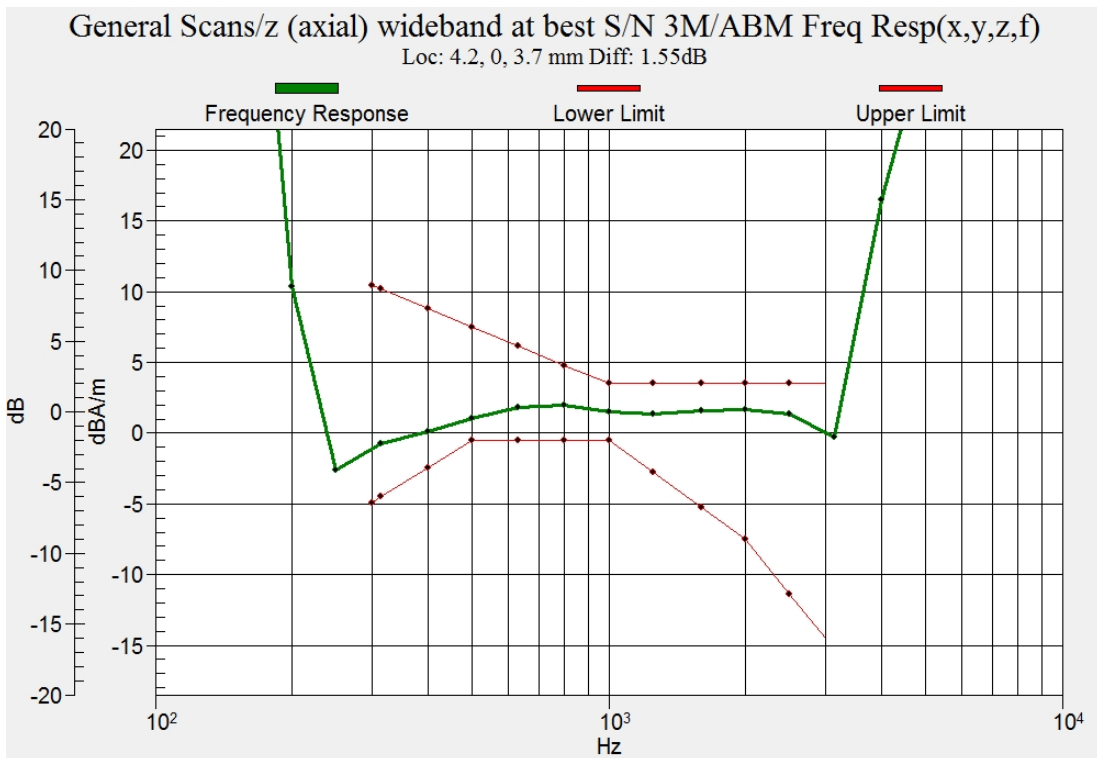
Figure C.8 Frequency Response of LTE B12 3M
