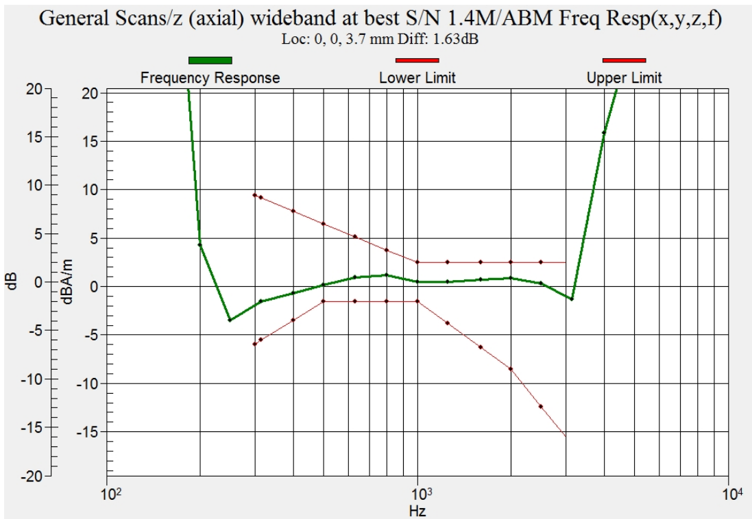
Figure C.7 Frequency Response of LTE B12 1.4M
