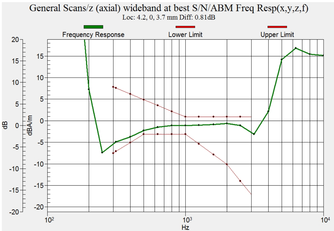
Figure C.3 Frequency Response of WCDMA 1700
