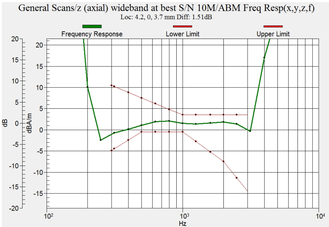
Figure C.11 Frequency Response of LTE B30 10M
