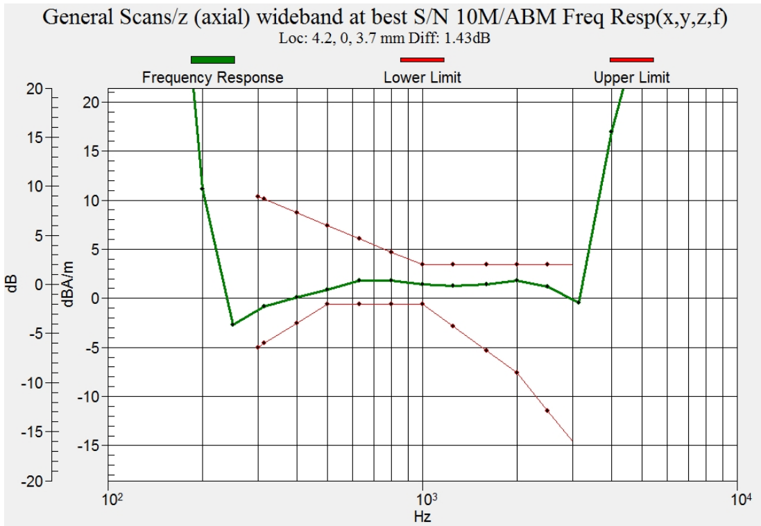
Figure C.9 Frequency Response of LTE B14
