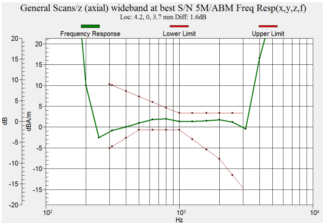
Figure C.10 Frequency Response of LTE B30 5M
