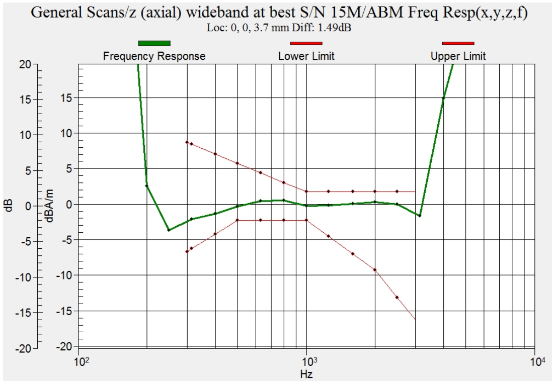
Figure C.13 Frequency Response of LTE B66 15M
