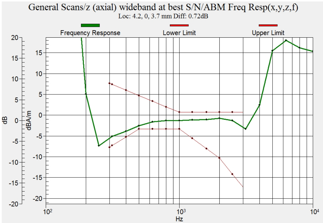
Figure C.1 Frequency Response of WCDMA 850
