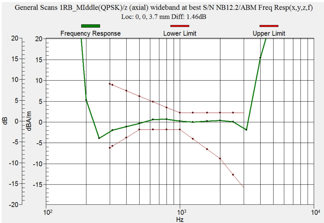
Figure C.5 Frequency Response of LTE B2 20M
