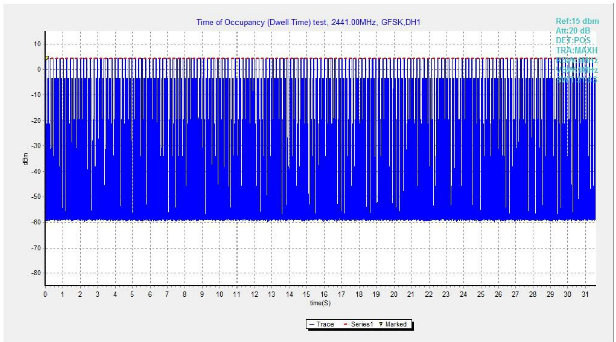
Fig.65. Number of Transmissions Measurement: Channel 39,Packet DH1
