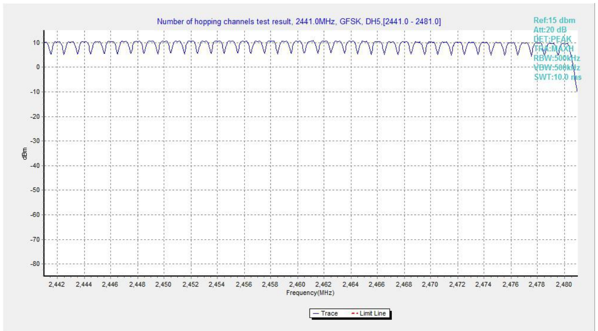
Fig.95. Number of hopping frequencies: GFSK, Channel 40 - 78
