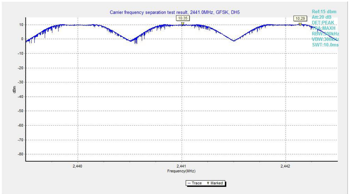
Fig.91. Carrier frequency separation measurement: GFSK, Channel 39
