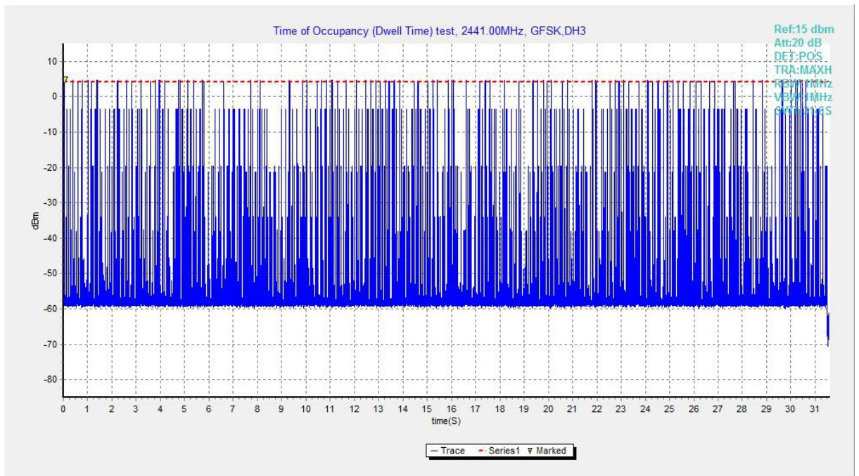
Fig.67. Number of Transmissions Measurement: Channel 39,Packet DH3
