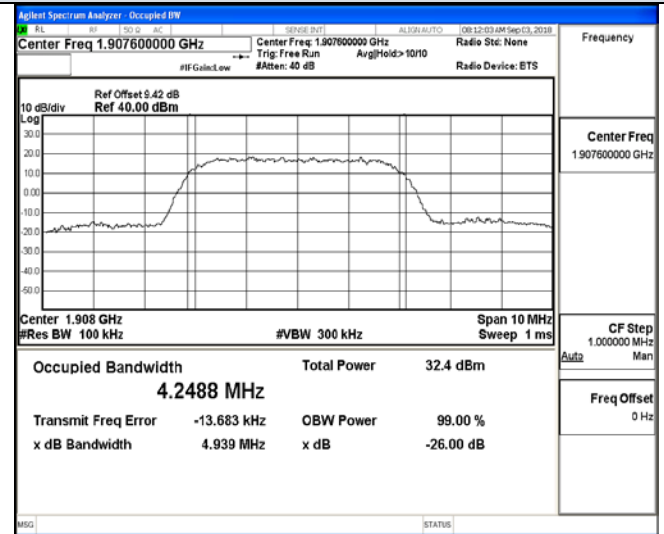
Channel 9538 / 1907.6 MHz
