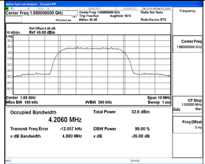
Channel 9400 / 1880.0 MHz
