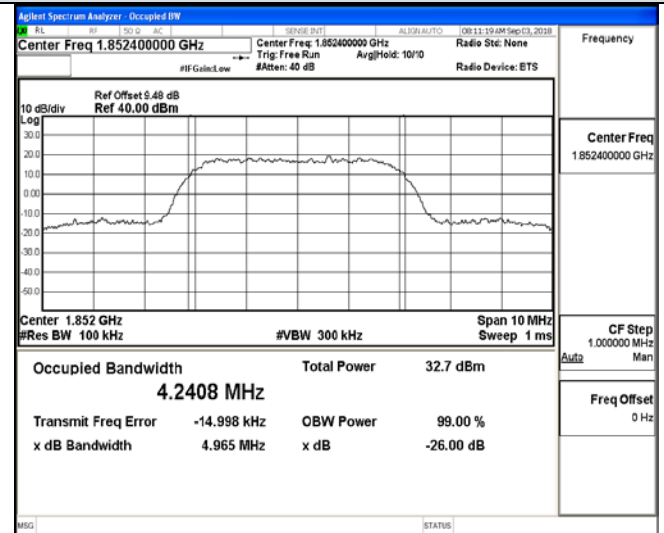
Channel 9262 / 1852.4 MHz
