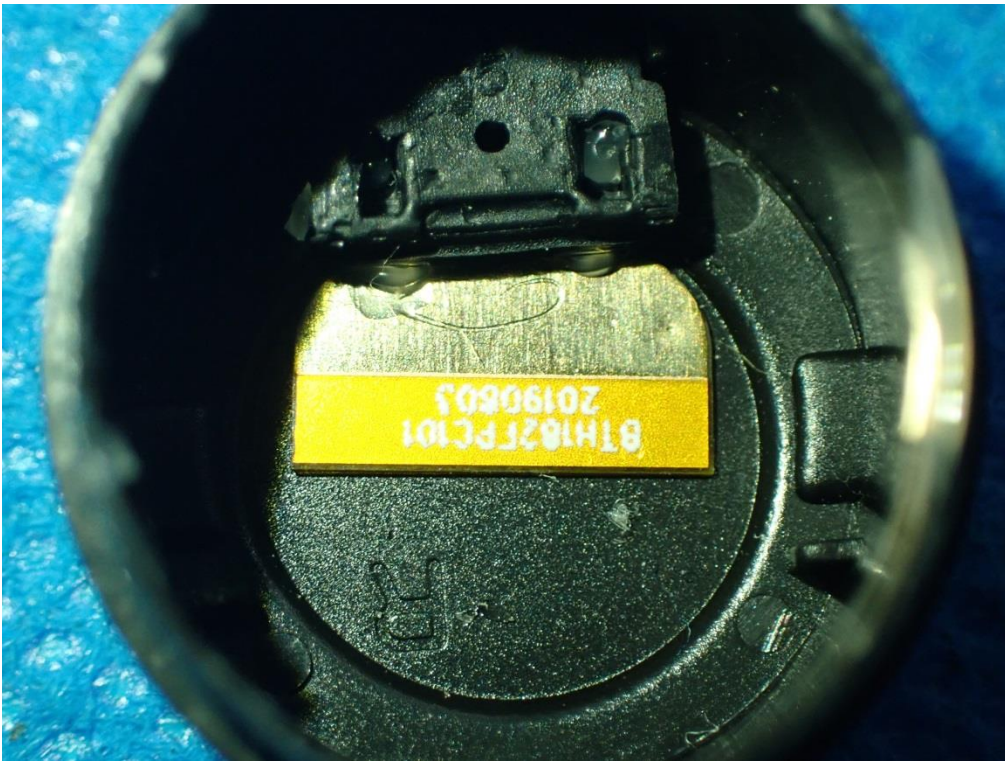
INTERNAL VIEW-9 OF EUT(Right earphone)
