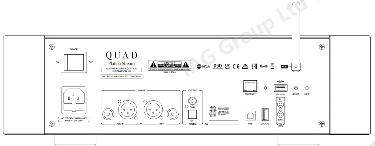
Power Switch Mains Input Analogue outputs Digital outputs Wi-F- Antenna Ethernet USB Storage Reset WPS PC USB USB Update 12V trigger
