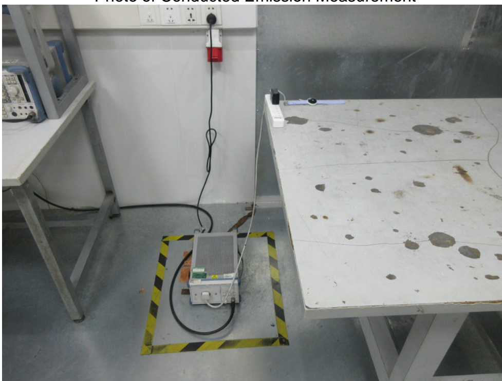
FCC ID: 2A058-B18 Photo of Conducted Emission Measurement
