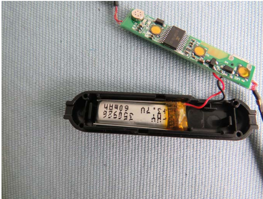
BT Chip
