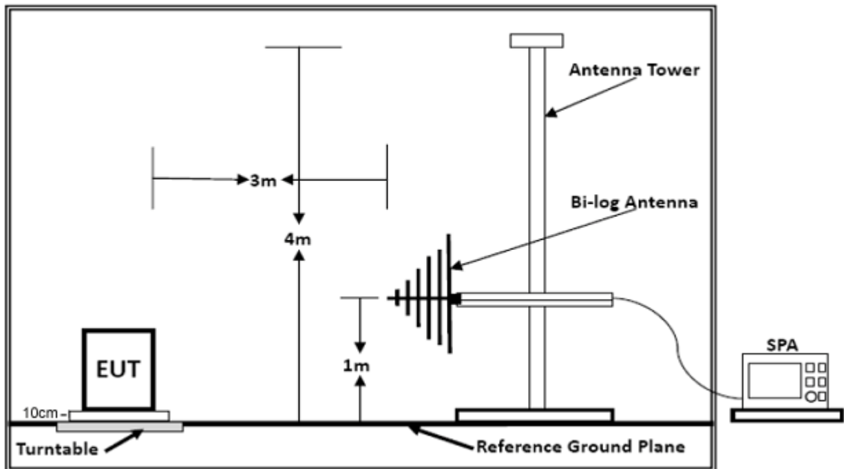
(B) Radiated Emission Test-Up Frequency 30MHz~1GHz
