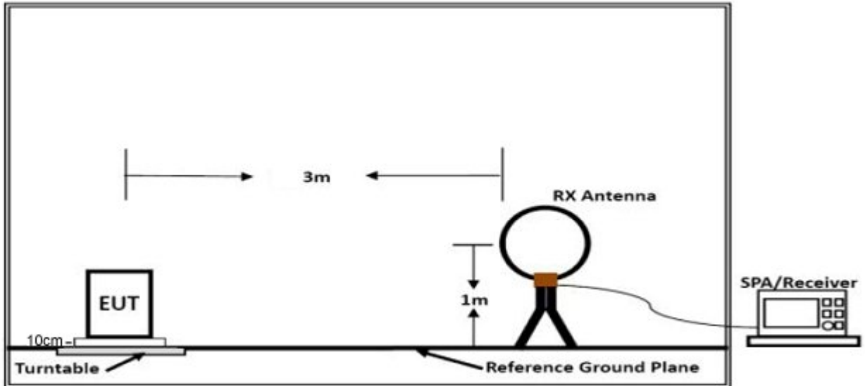
(A) Radiated Emission Test-Up Frequency Below 30MHz
