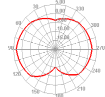
Bluetooth 39 TRP H
