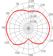
Bluetooth 39 TRP
