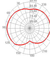
Bluetooth 39 TIS
