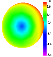
Bluetooth 0 TRP
