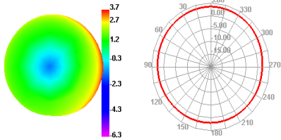
Bluetooth 0 TRP H
