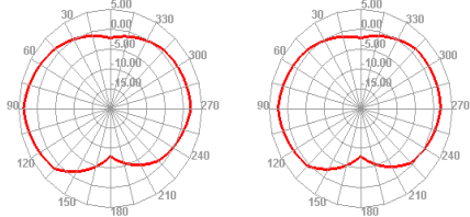
Bluetooth 39 TRP
