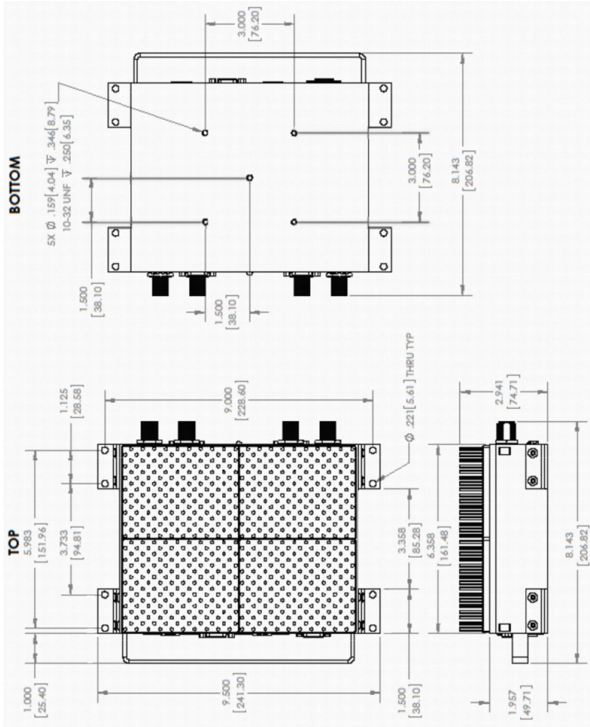
Figure 2 Mounting Dimensions
