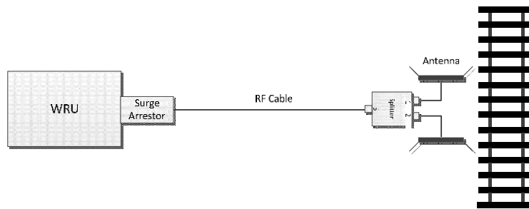
Figure 4 Access Point Radio Installation – Two Antennas
