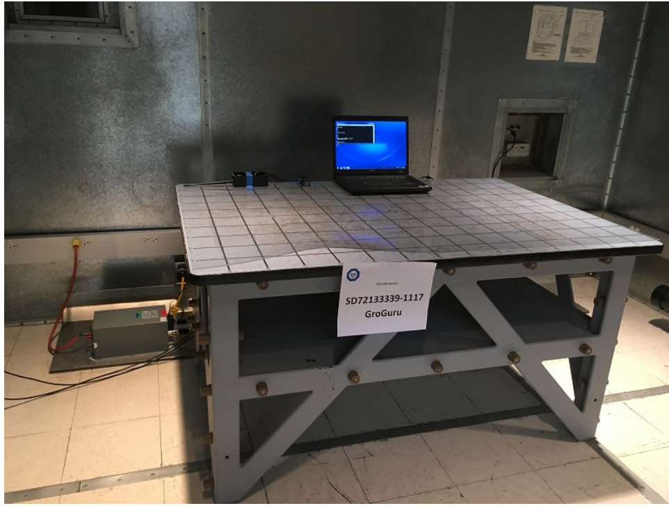
Conducted Emissions Front (Base Unit)
