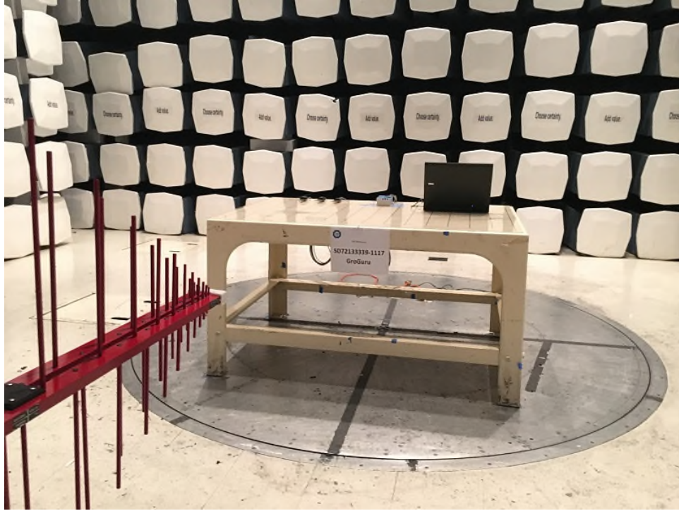
Radiated Emissions Below 1GHz Front (STEM Host)
