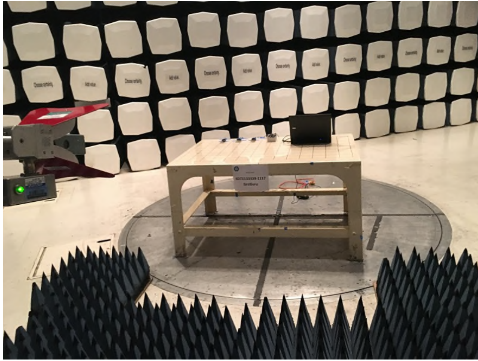
Radiated Emissions Above 1GHz Front (STEM Host)
