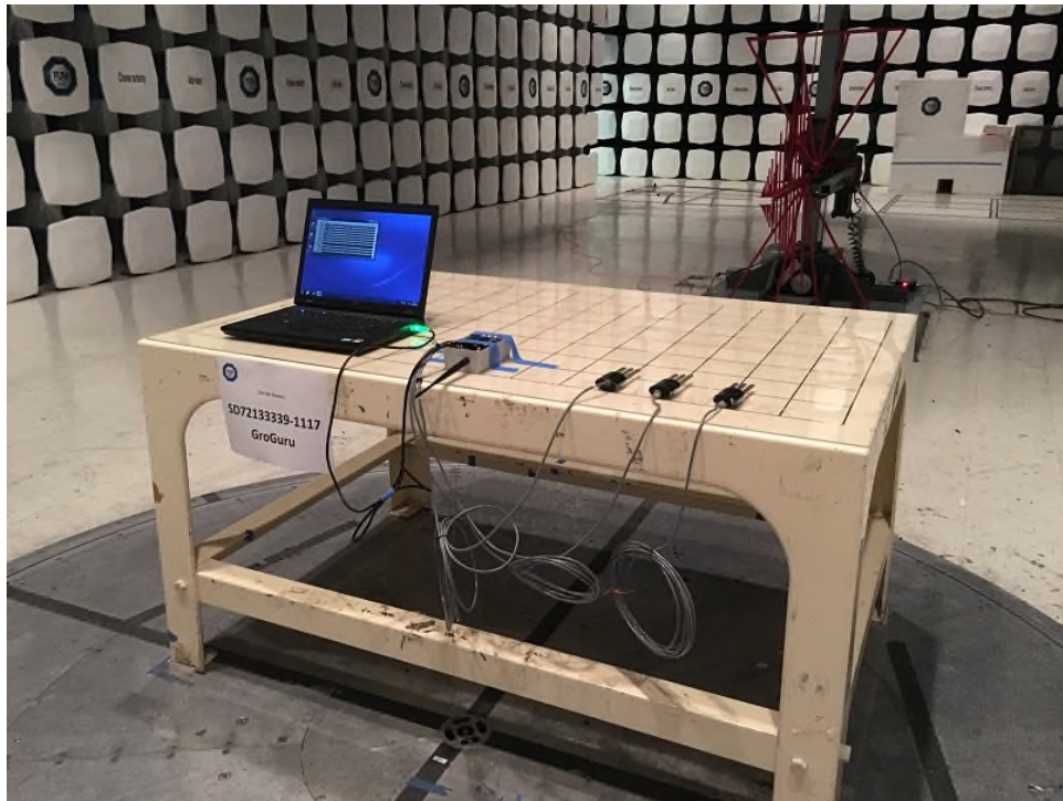
Radiated Emissions Below 1GHz Rear (STEM Host)
