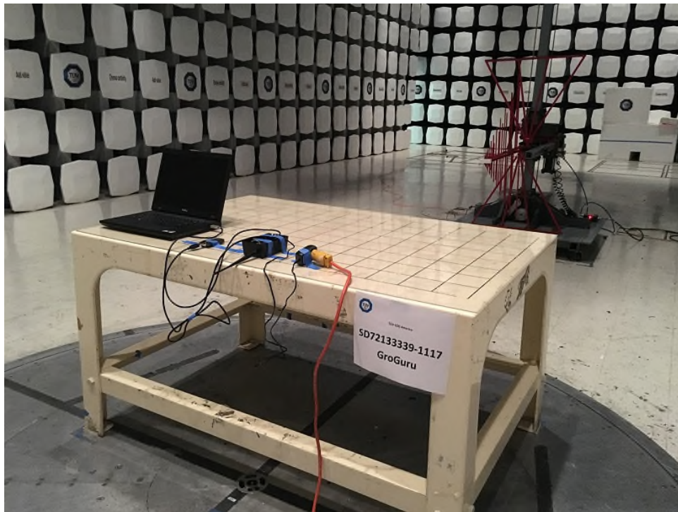
Radiated Emissions Below 1GHz Rear (BASE Host)
