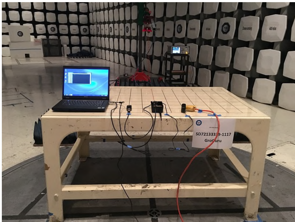
Radiated Emissions Above 1GHz Front (BASE Host)
