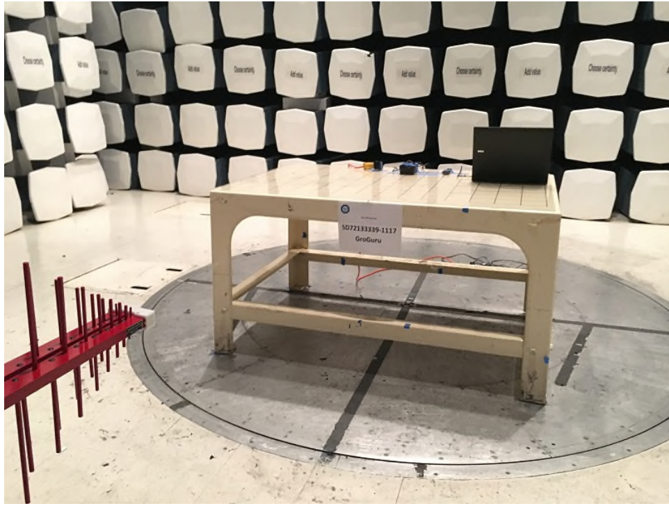
Radiated Emissions Below 1GHz Front (BASE Host)
