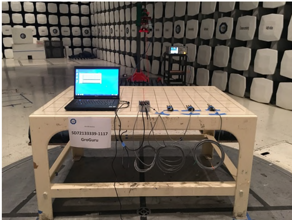
Radiated Emissions Above 1GHz Rear (STEM Host)
