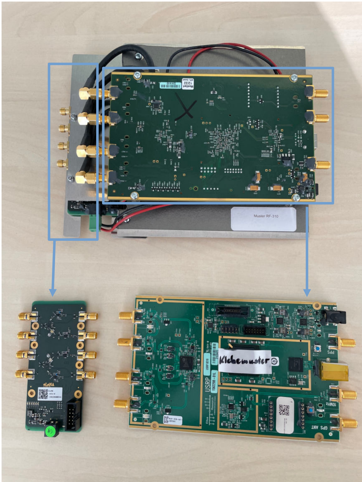
RF Modul with eLeNA board and the Ettus (NI) USRP B210 broadband receiver
