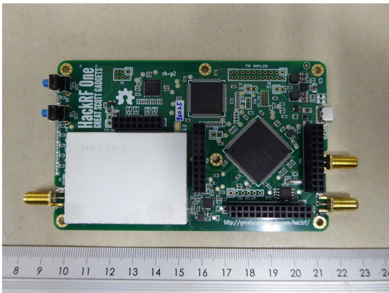
162281_EUT24: detail view
