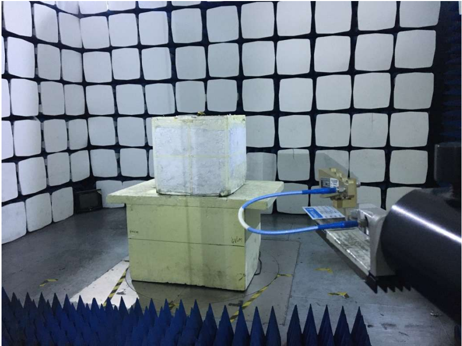
Radiated Emission Test Setup (Above 18 GHz) from 1.5M-Height Turntable Test Table
