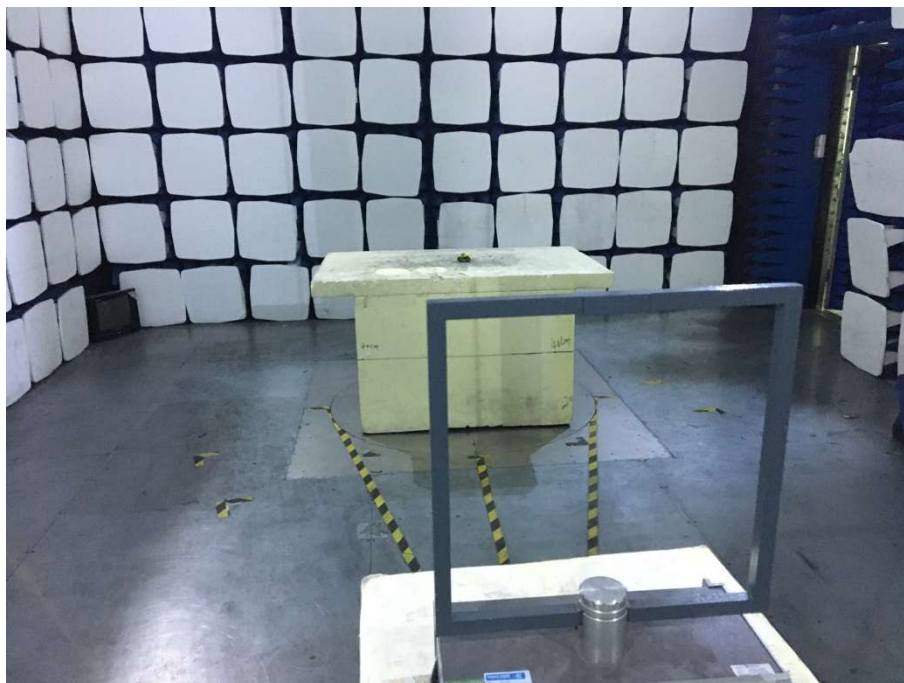
Radiated Emission Test Setup (Below 30 MHz) from 0.8M-Height Turntable Test Table
