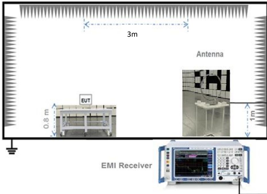
For Radiated Emission Test (Below 30 MHz)
