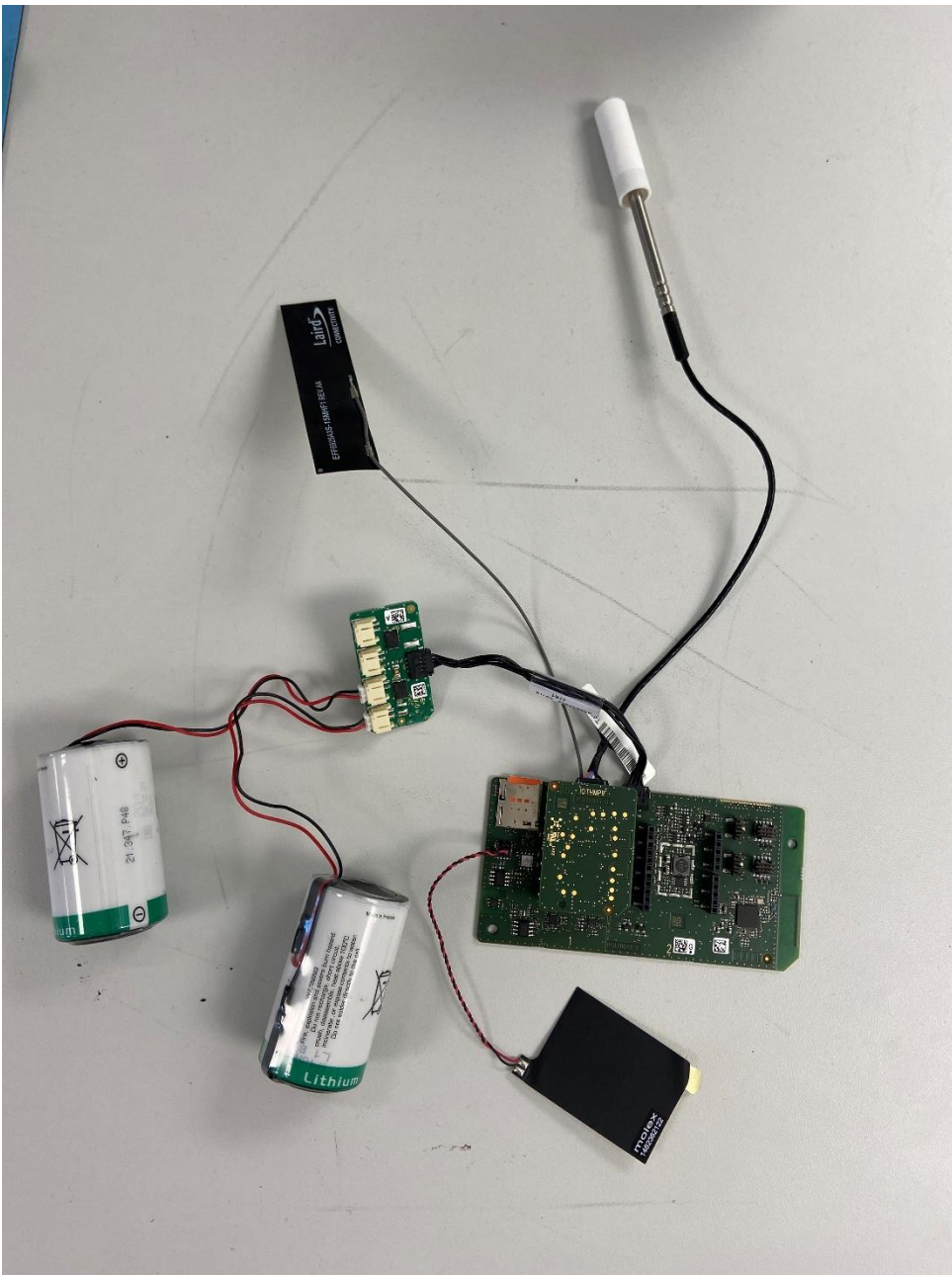
Photo 8. FMP102 Electronics
