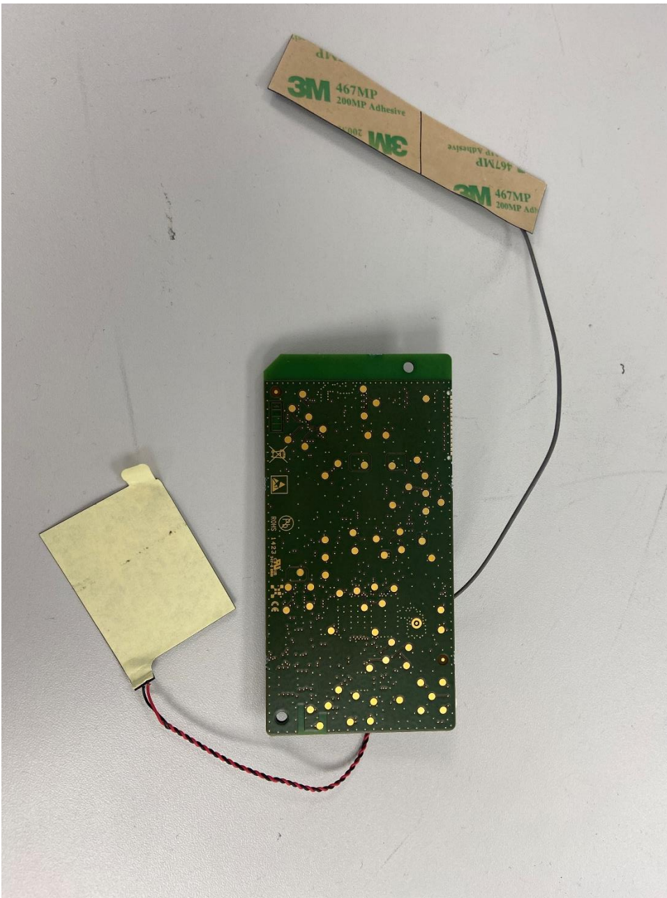
Photo 10. IOTMAINCB and Antennas, Back View
