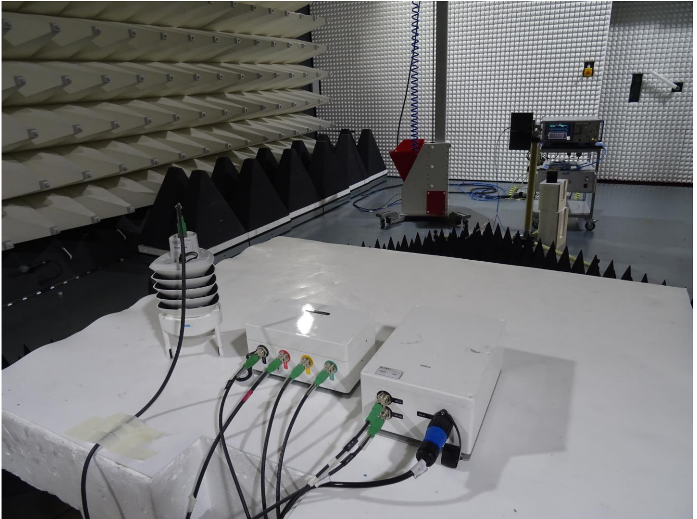
Photograph Radiated emission. High Range.
