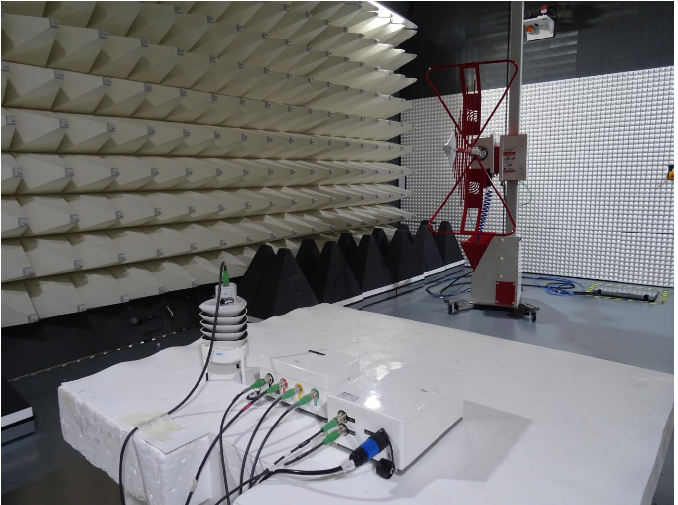
Photograph Radiated emission. Low Range.
