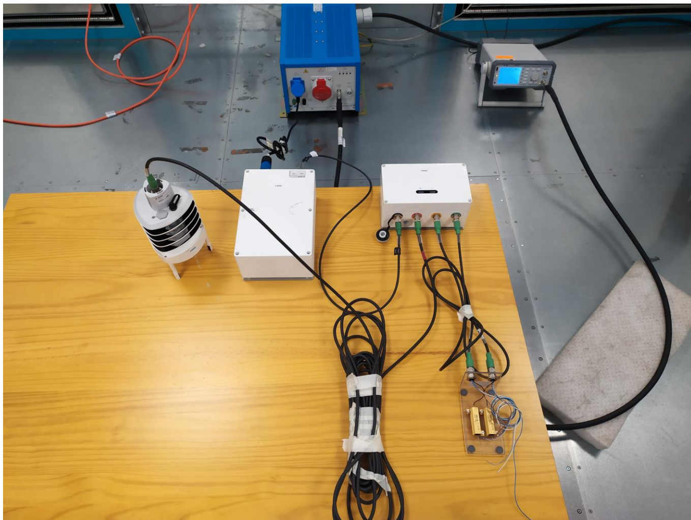
Photograph Conducted Emission
