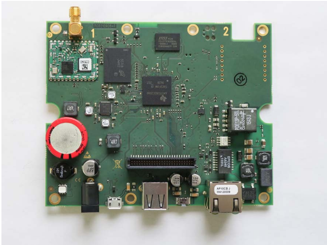
PCB radio module shield off
