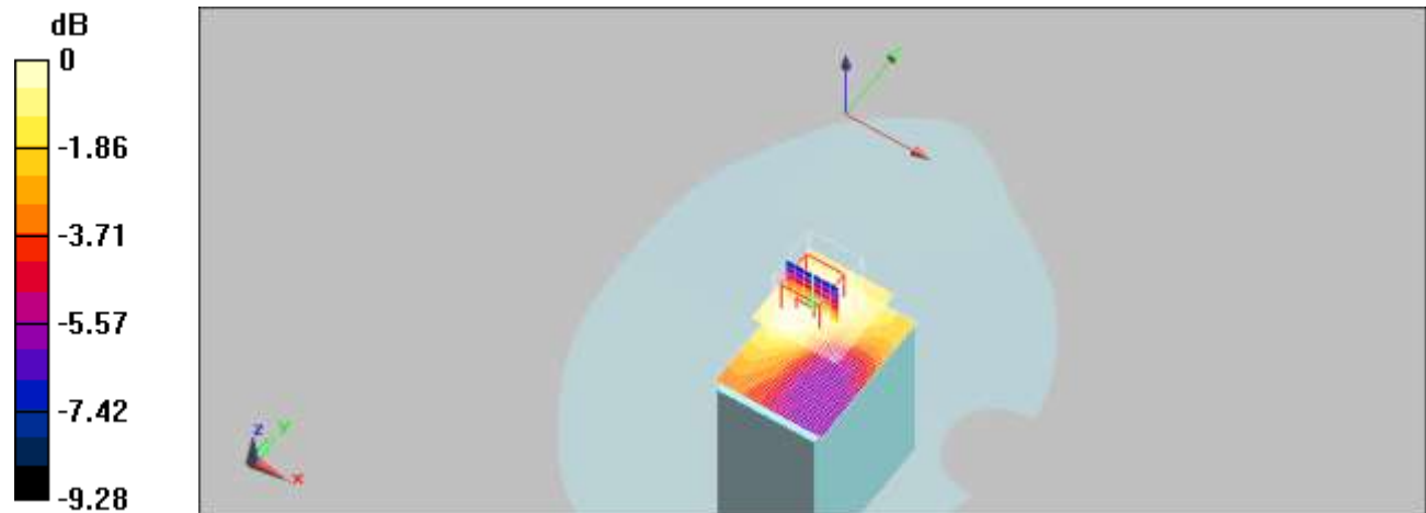
0 dB = 0.024mW/g
