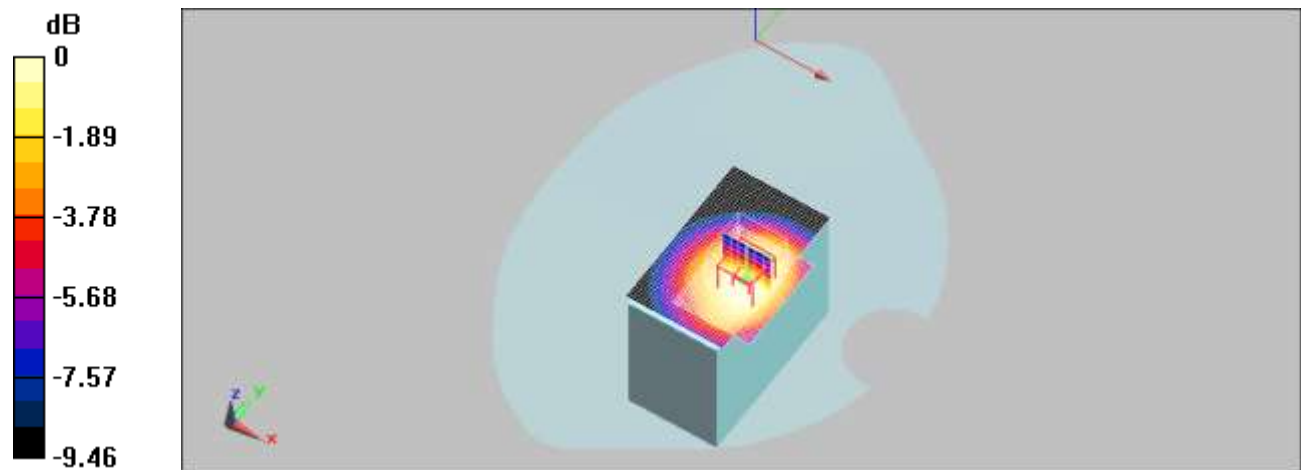
0 dB = 0.155mW/g
