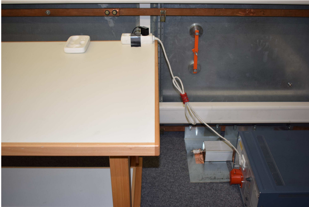
Picture 9: AC power line conducted emission – Standby (front view)
