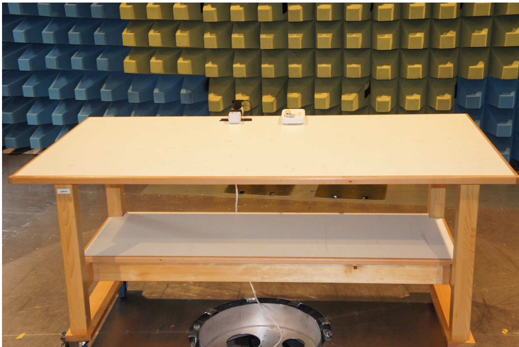
Picture 8: SAC, radiated emission test 30 MHz – 1 GHz – Charging (rear view)
