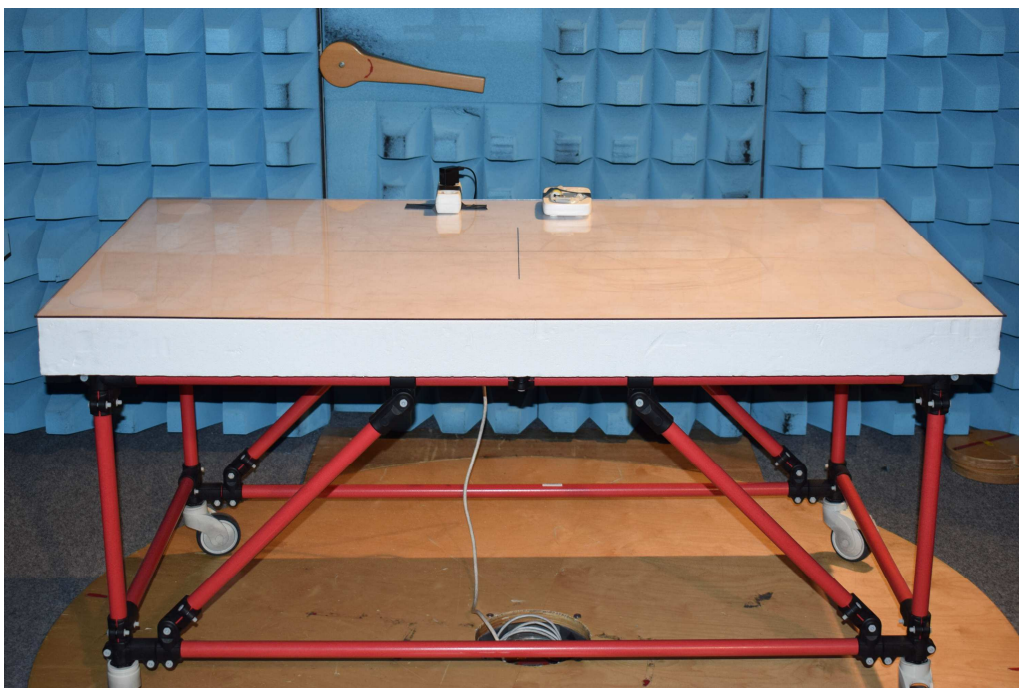
Picture 4: CDC, radiated emission test 9 kHz -30 MHz - Charging (rear view)
