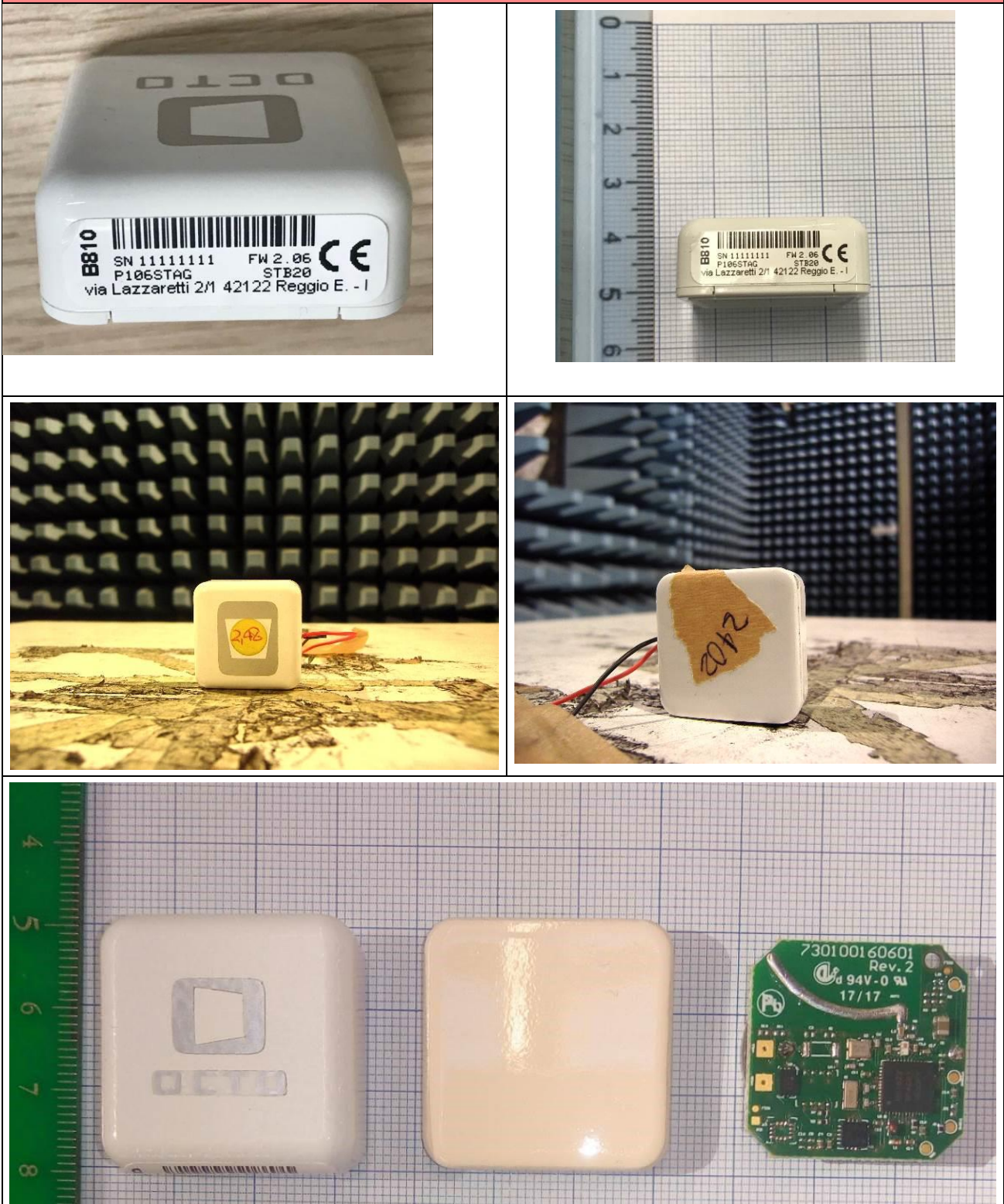
PHOTO N°1 – EUT IDENTIFICATION
