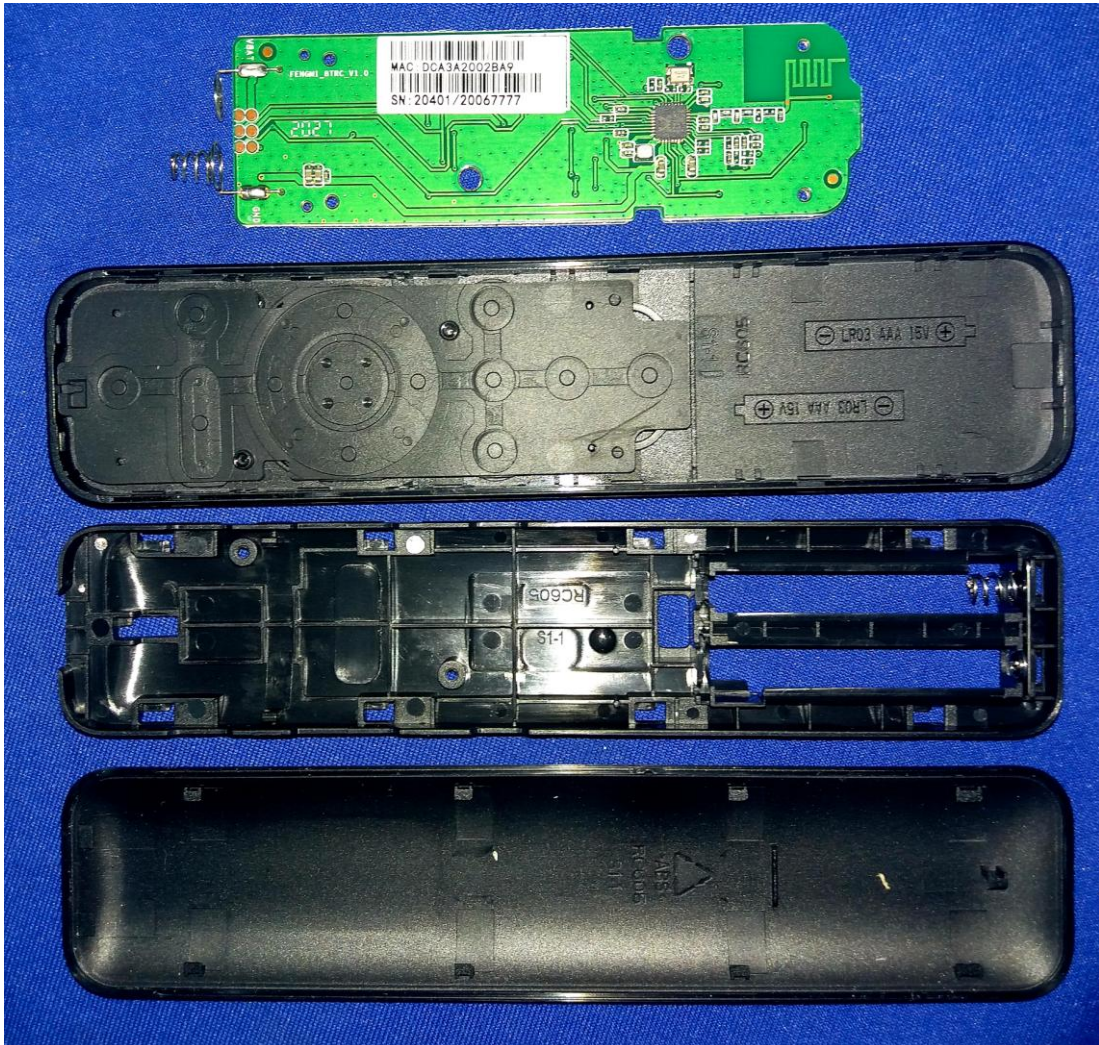
Figure 6 Inside of the EUT
