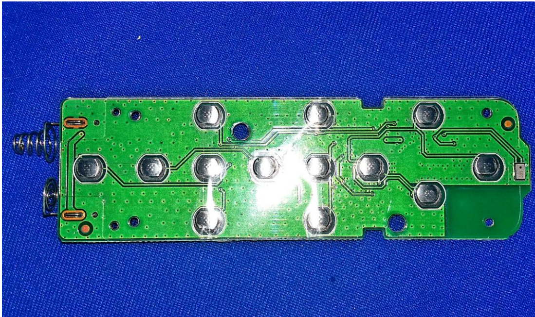
Figure 8 Inside of the EUT
