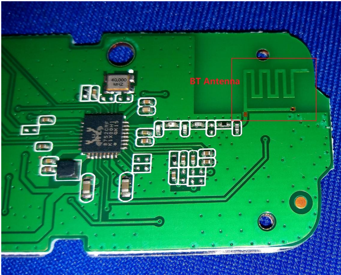
Figure 9 Inside of the EUT
