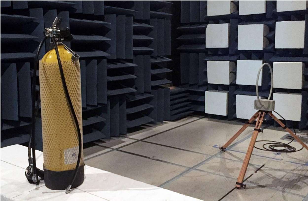
Radiated Emissions, 10kHz to 30MHz with Loop Antenna.
