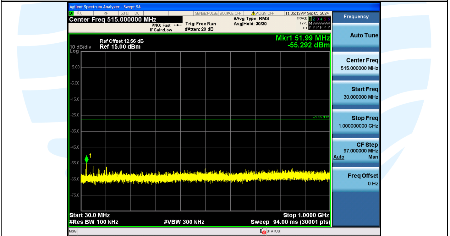
3DH5-Ant1-2402-30~1000-PASS
