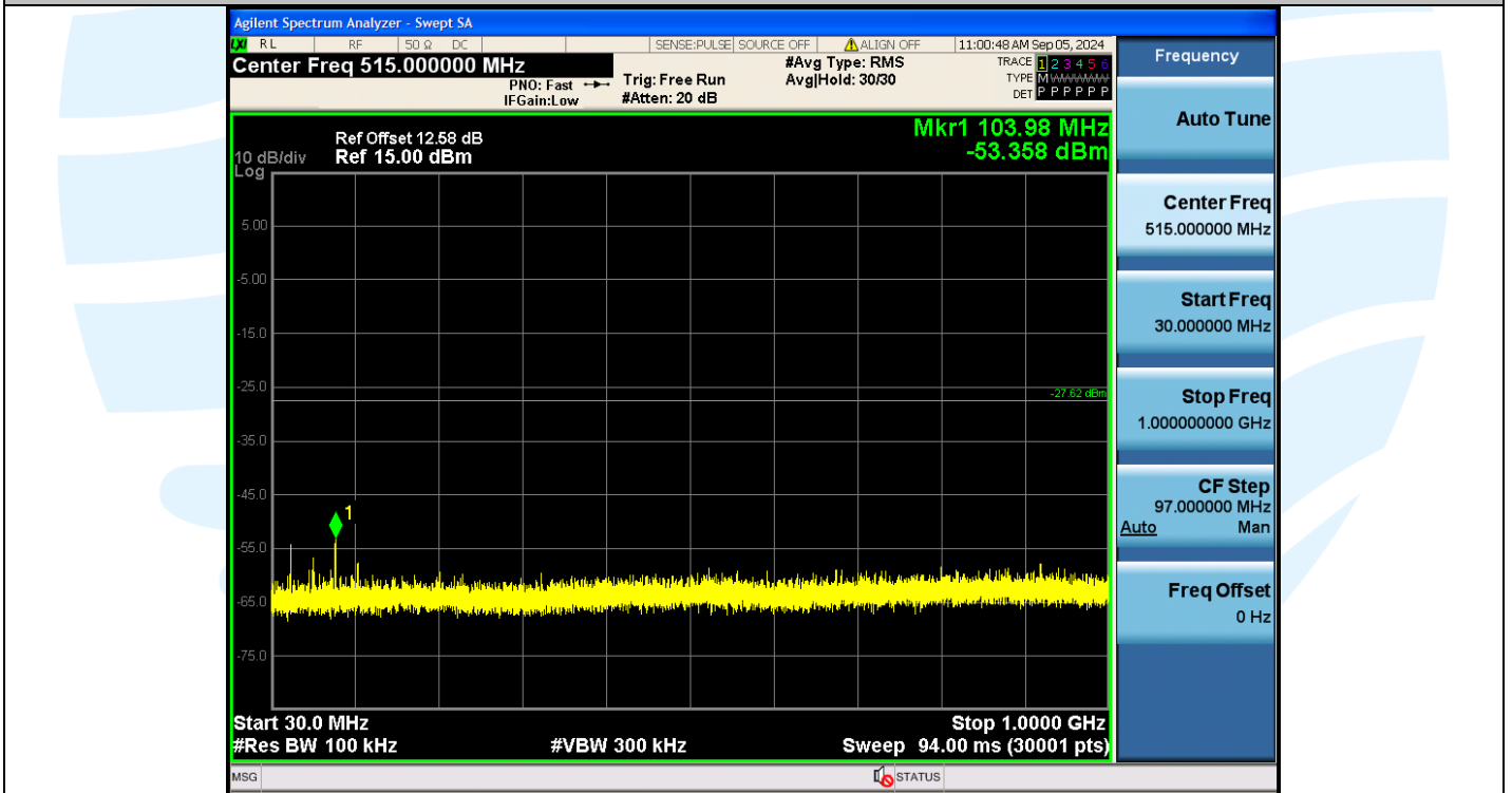
2DH5-Ant1-2441-30~1000-PASS
