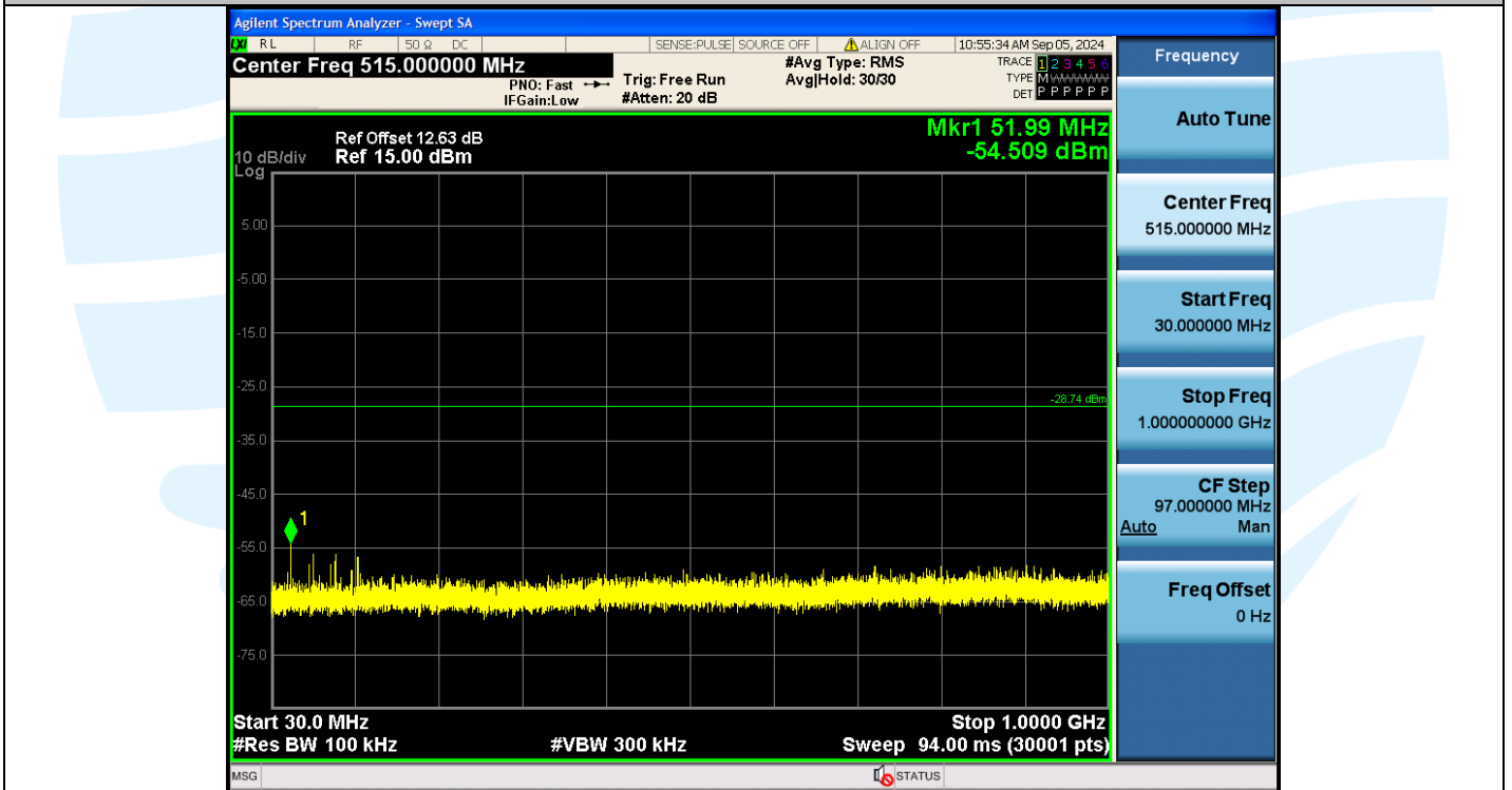
DH5-Ant1-2480-30~1000-PASS
