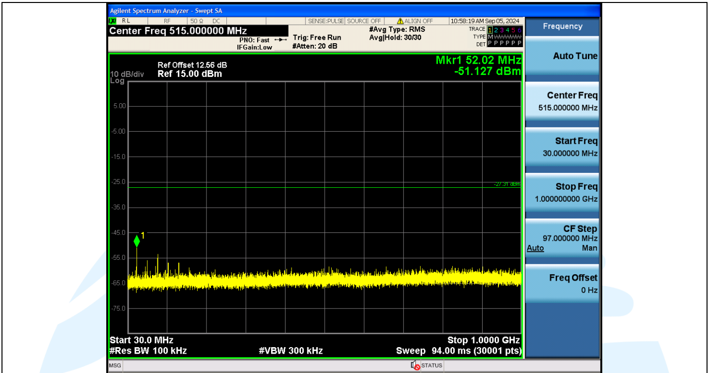
2DH5-Ant1-2402-30~1000-PASS
