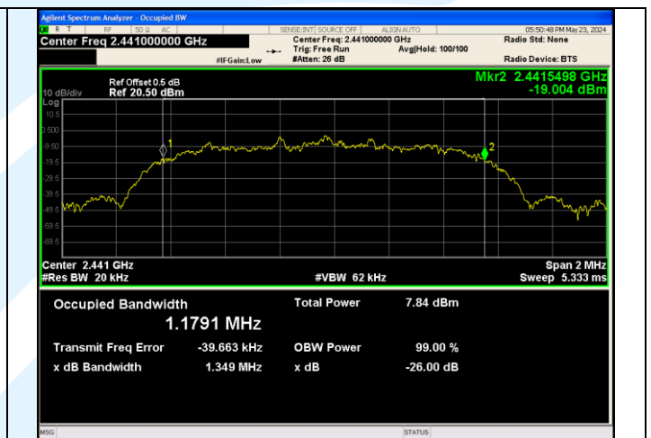
8DPSK_3-DH5_Channel 39
