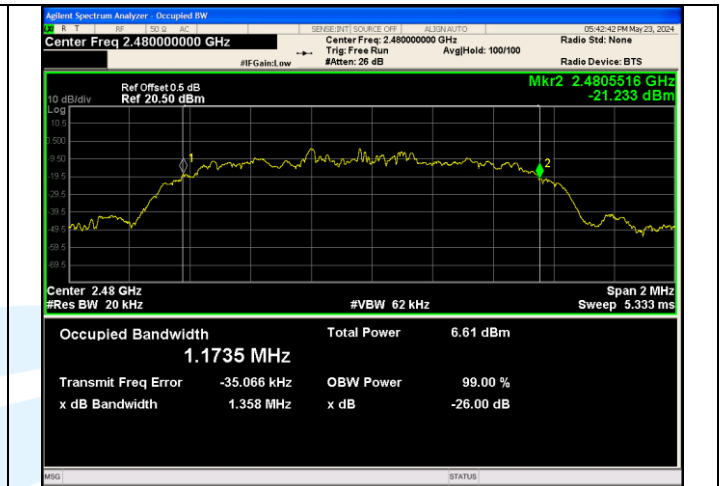
\pi/4 DQPSK_2-DH5_Channel 78
