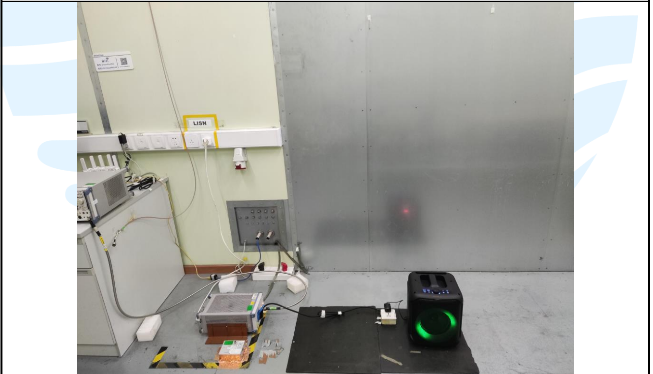
Conducted Emission Test Setup
