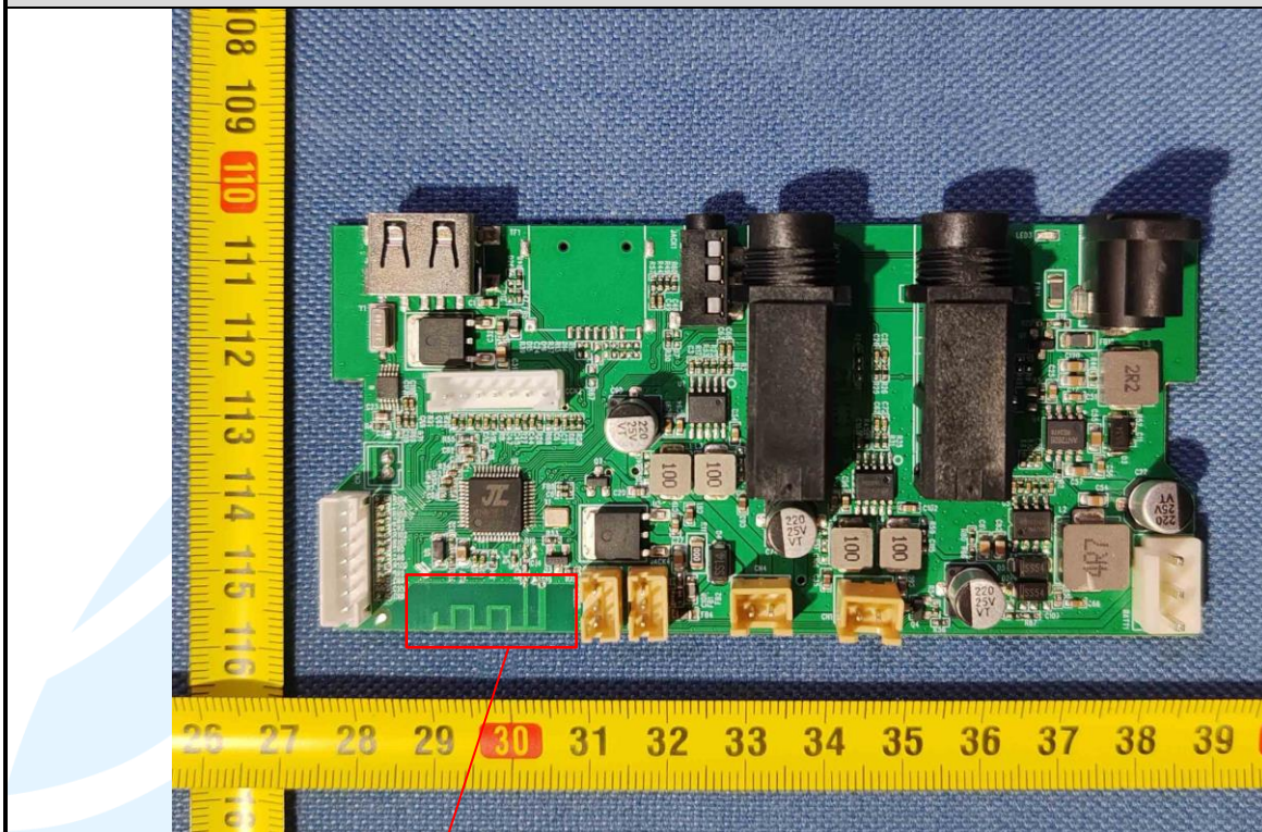
BT Antenna
