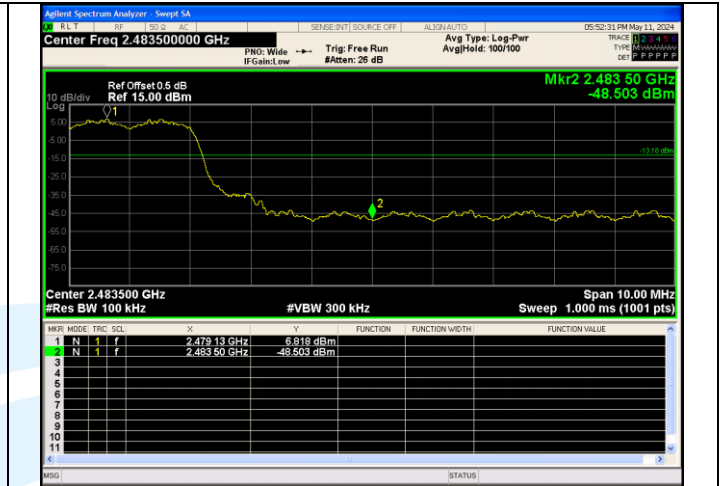
Out Of Band Emission(Right) π/4DQPSK 2-DH5 Channel Hopping
