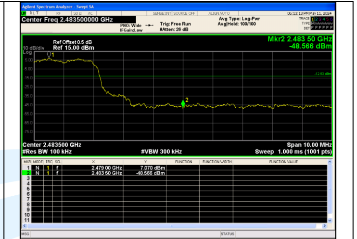
Out Of Band Emission(Right) 8DPSK 3-DH5 Channel Hopping
