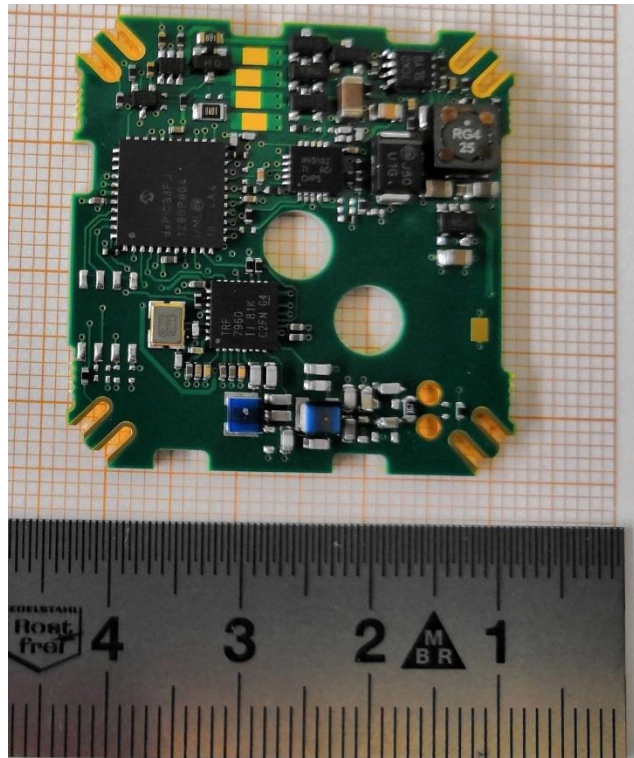
PCB mainboard – top view
