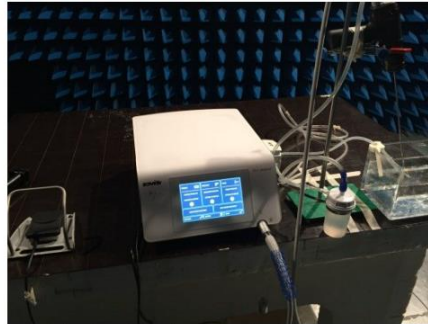
Test setup in anechoic chamber
