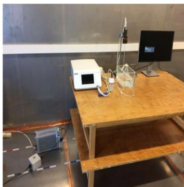
Test setup
