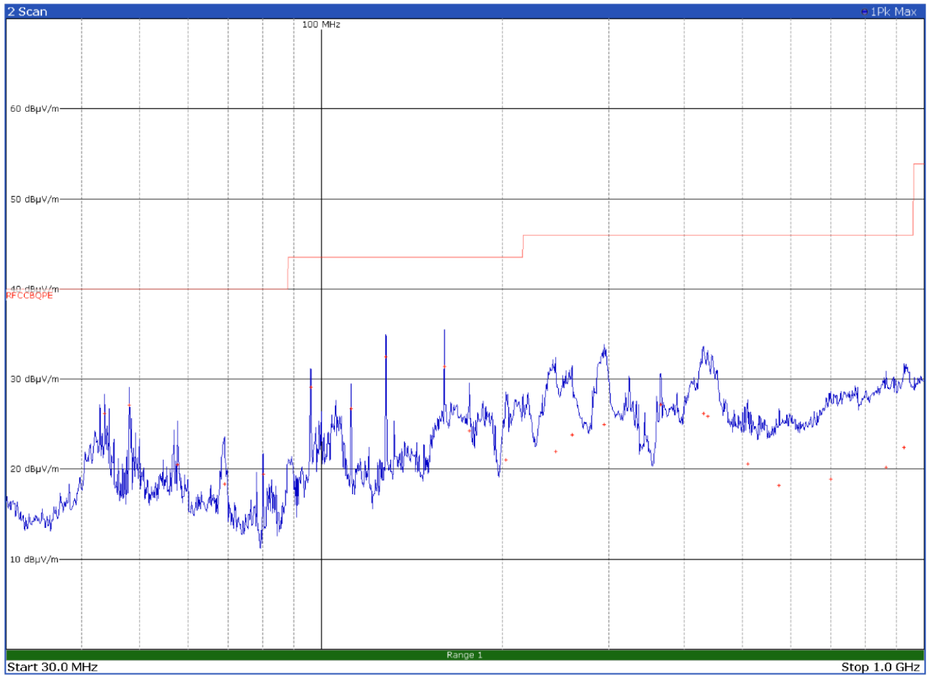
Figure 8.3-2: Radiated emissions with antenna in horizontal polarization
