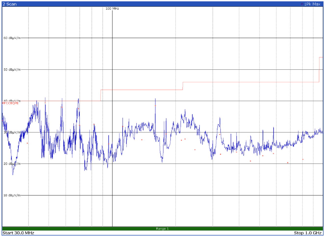
Figure 8.3-3: Radiated emissions with antenna in vertical polarization
