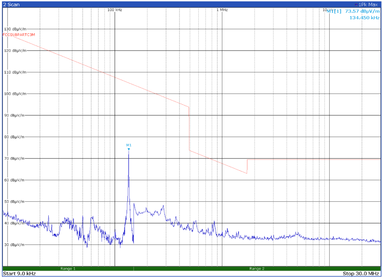
Figure 8.3-1: Radiated emissions with antenna loop
