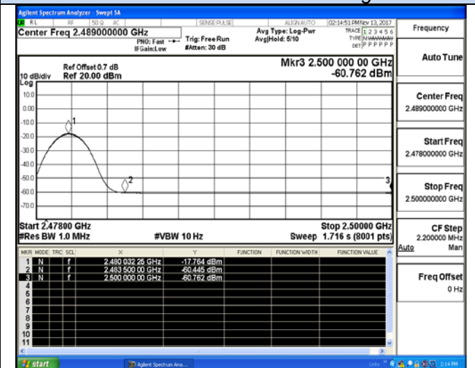
Channel 78 / 2480 MHz – Average
