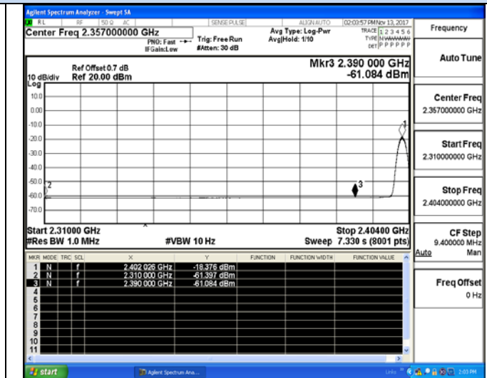
Channel 0 / 2402 MHz –Average
