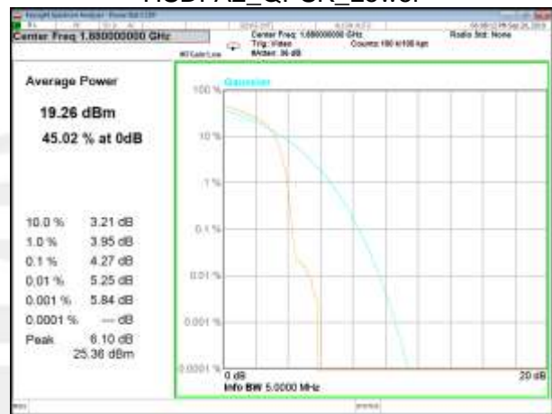
HSDPA2_QPSK_Middle
