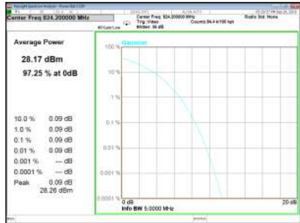
GPRS850_QPSK_Lower
