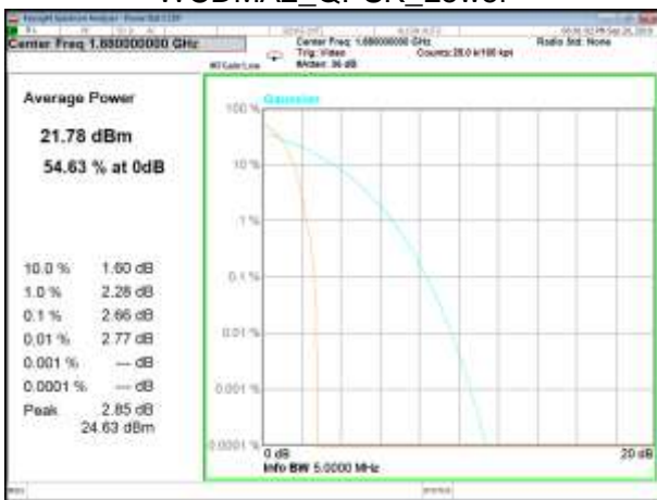
WCDMA2_QPSK_Middle
