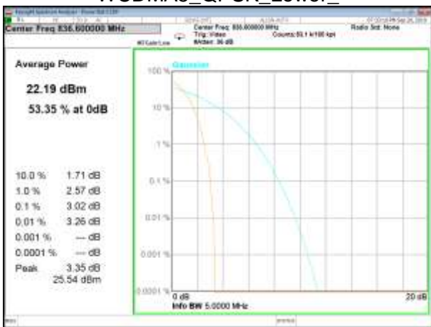
WCDMA5_QPSK_Middle_
