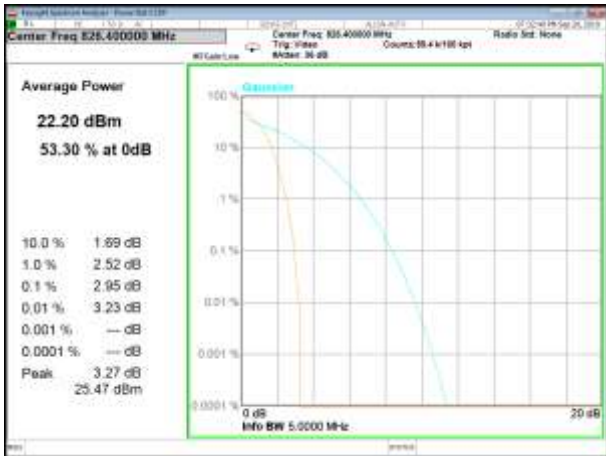
WCDMA5_QPSK_Lower_
