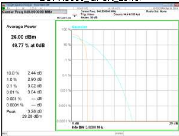
EGPRS850_QPSK_Higher
