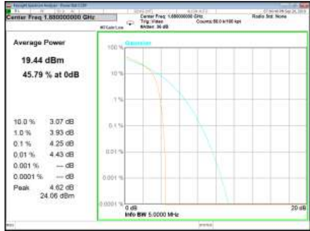
HSUPA2_QPSK_Middle
