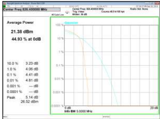
HSDPA5_QPSK_Lower_
