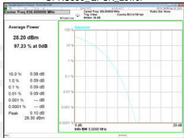
GPRS850_QPSK_Middle
