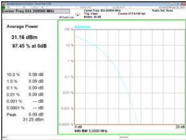
GSM850_QPSK_Lower
