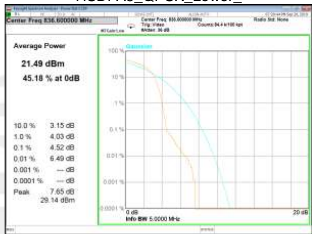
HSDPA5_QPSK_Middle_
