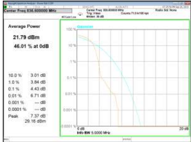
HSUPA5_QPSK_Middle_
