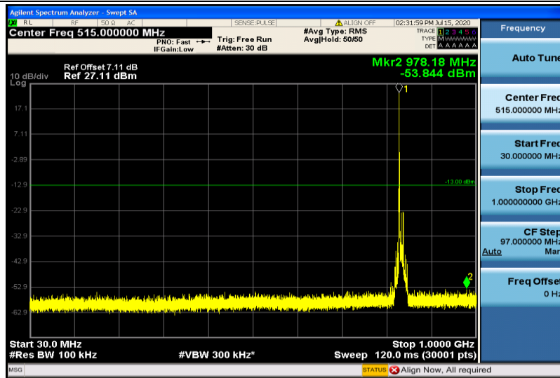
Band26-10MHz-16QAM-26915-1RB#0-30~1000MHz
