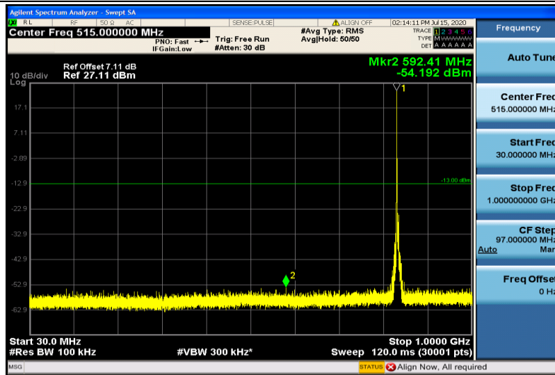
Band26-5MHz-QPSK-26915-1RB#0-30~1000MHz
