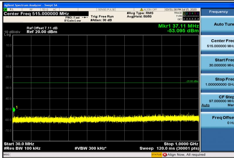
Band41-15MHz-16QAM-40740-1RB#0-30~1000MHz
