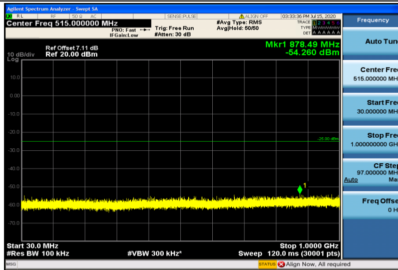
Band41-10MHz-16QAM-40740-1RB#0-30~1000MHz
