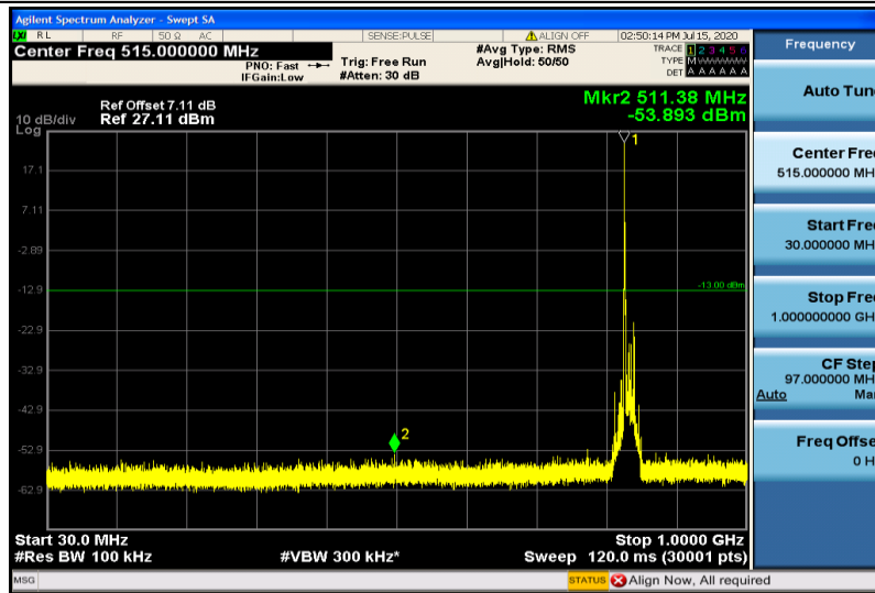
Band26-15MHz-QPSK-26915-1RB#0-30~1000MHz
