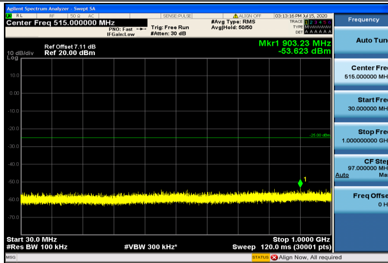
Band41-5MHz-16QAM-40740-1RB#0-30~1000MHz
