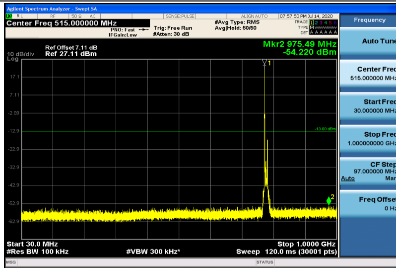
Band13-10MHz-QPSK-23230-1RB#0-30~1000MHz
