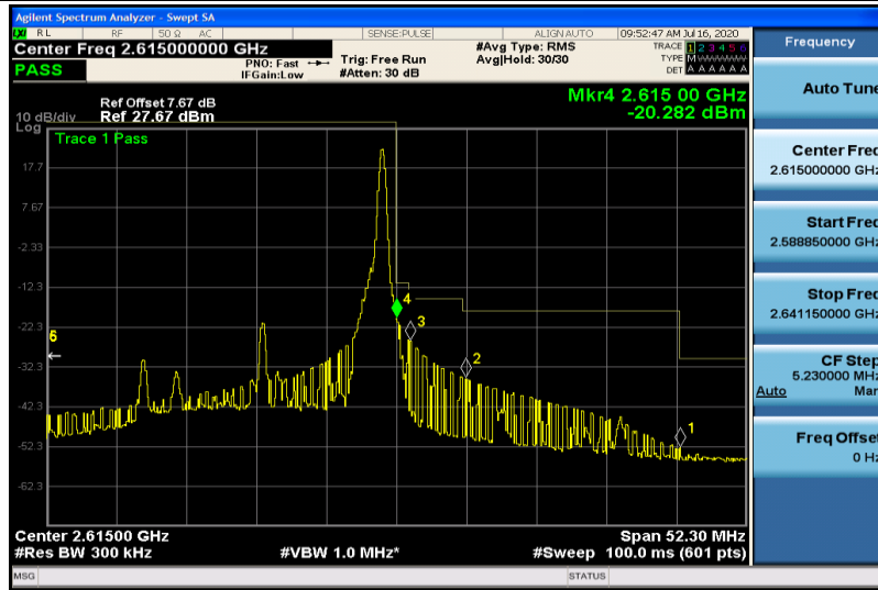
Band41-20MHz-16QAM-40740-1RB#99
