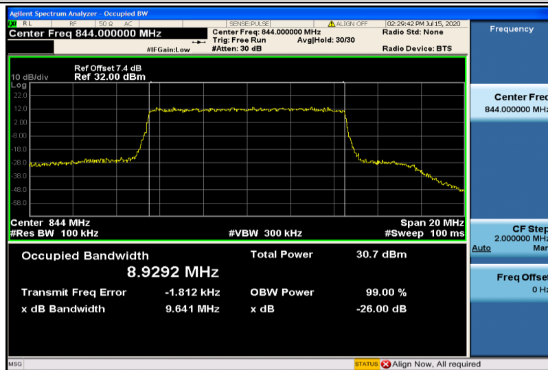
Band26-10MHz-QPSK-26990-50RB#0-8.9292
