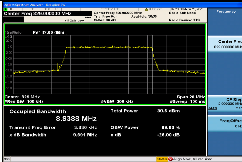
Band26-10MHz-QPSK-26840-50RB#0-8.9388
