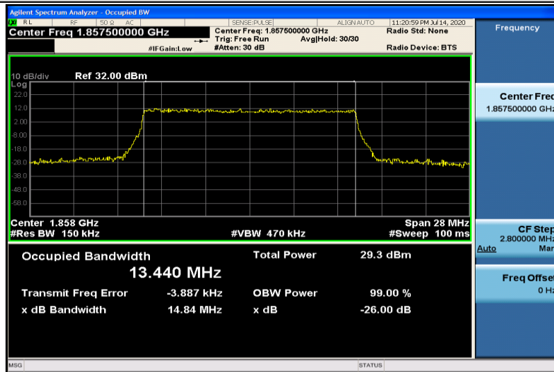
Band25-15MHz-16QAM-26115-75RB#0-13.440
