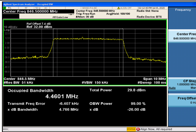
Band26-5MHz-16QAM-27015-25RB#0-4.4601
