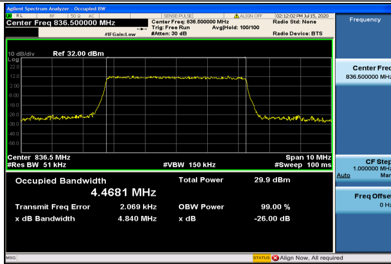
Band26-5MHz-16QAM-26915-25RB#0-4.4681
