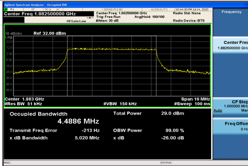
Band25-5MHz-16QAM-26365-25RB#0-4.4886
