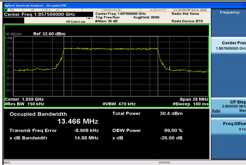
Band25-15MHz-QPSK-26115-75RB#0-13.466
