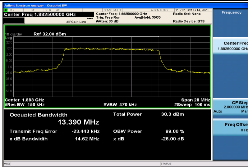
Band25-15MHz-QPSK-26365-75RB#0-13.390
