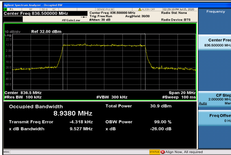
Band26-10MHz-QPSK-26915-50RB#0-8.9380
