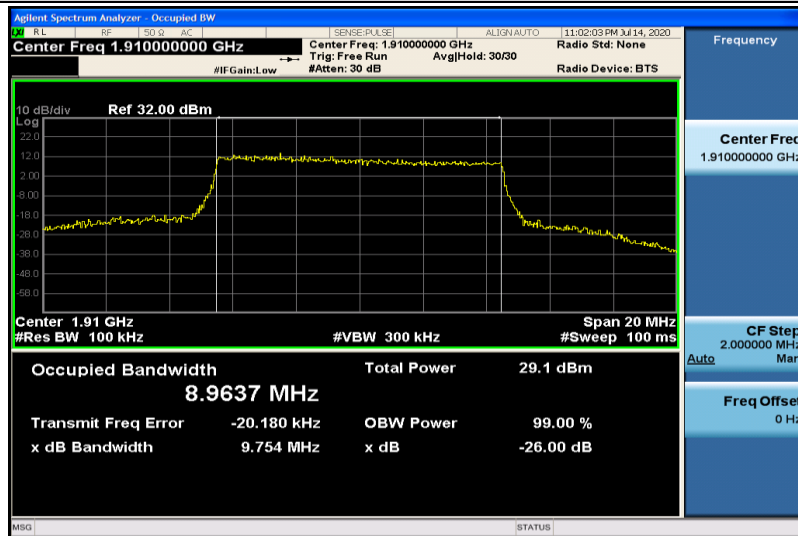
Band25-10MHz-16QAM-26640-50RB#0-8.9637
