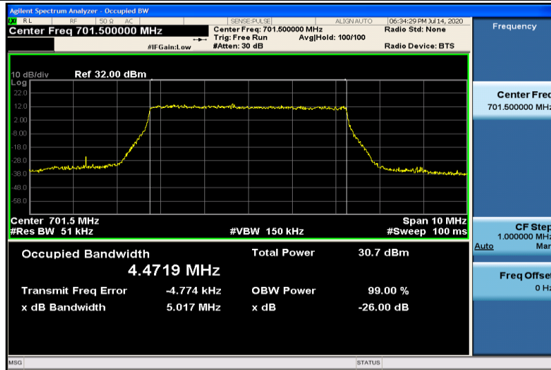
Band12-5MHz-QPSK-23035-25RB#0-4.4719
