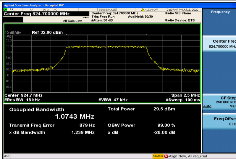
Band26-1.4MHz-QPSK-26797-6RB#0-1.0743
