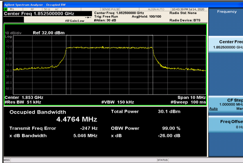
Band25-5MHz-QPSK-26065-25RB#0-4.4764
