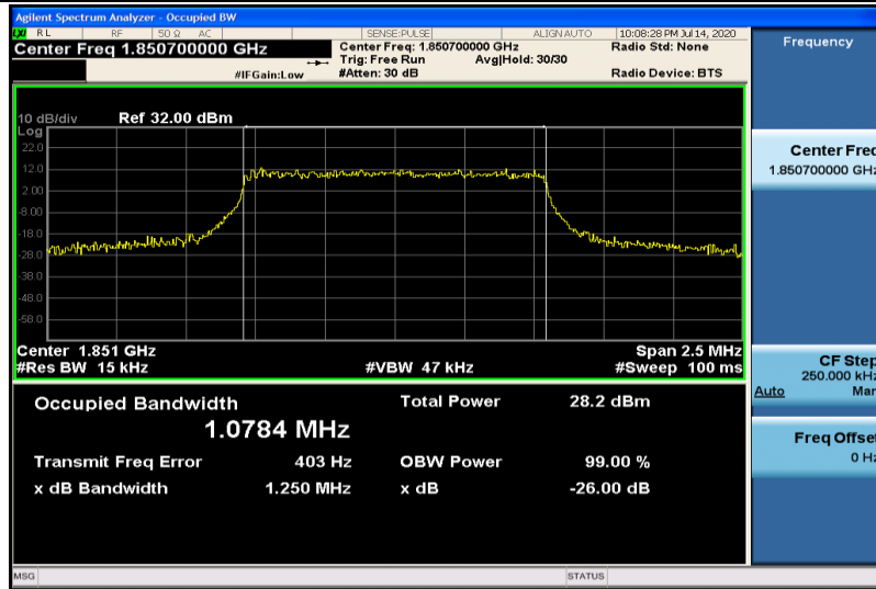
Band25-1.4MHz-16QAM-26047-6RB#0-1.0784
