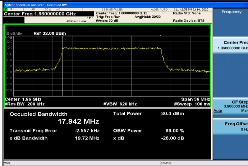
Band25-20MHz-QPSK-26140-100RB#0-17.942
