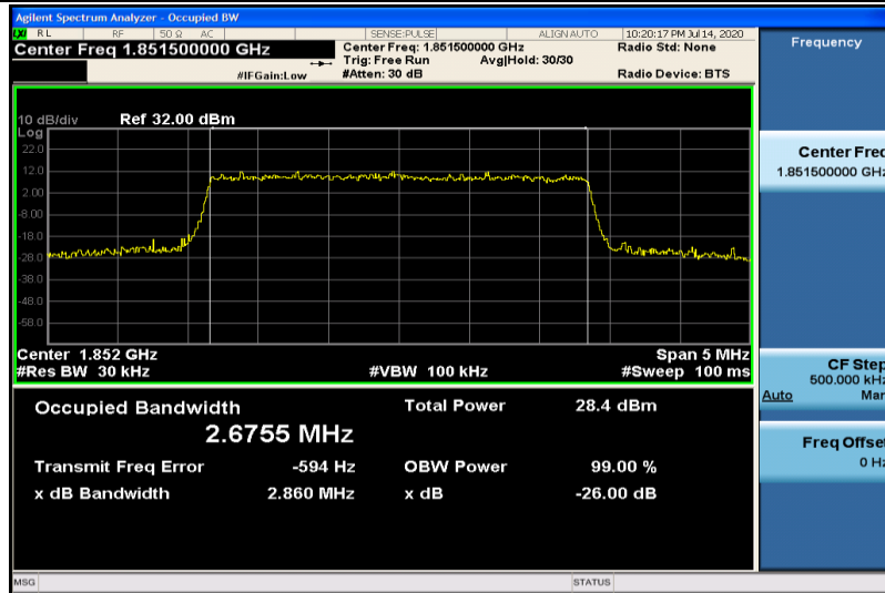
Band25-3MHz-16QAM-26055-15RB#0-2.6755
