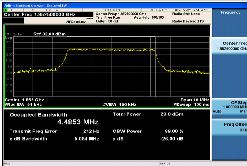
Band25-5MHz-16QAM-26065-25RB#0-4.4853
