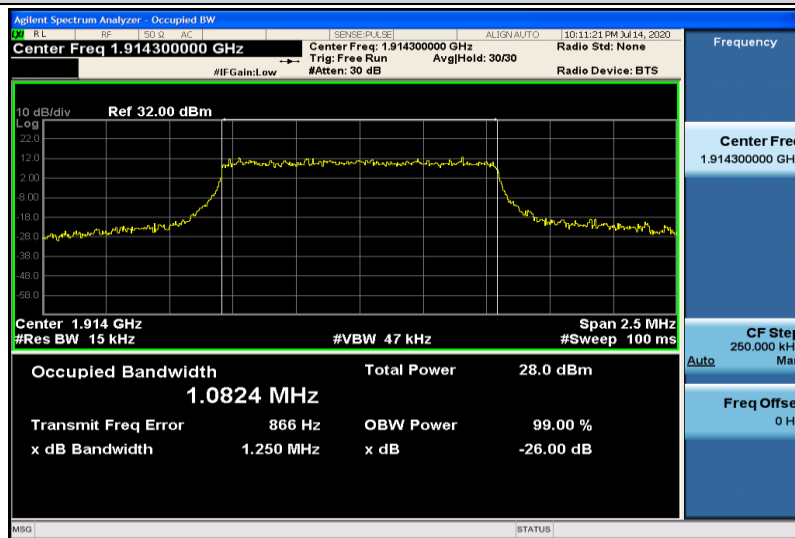
Band25-1.4MHz-16QAM-26683-6RB#0-1.0824
