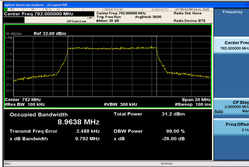
Band13-10MHz-QPSK-23230-50RB#0-8.9638
