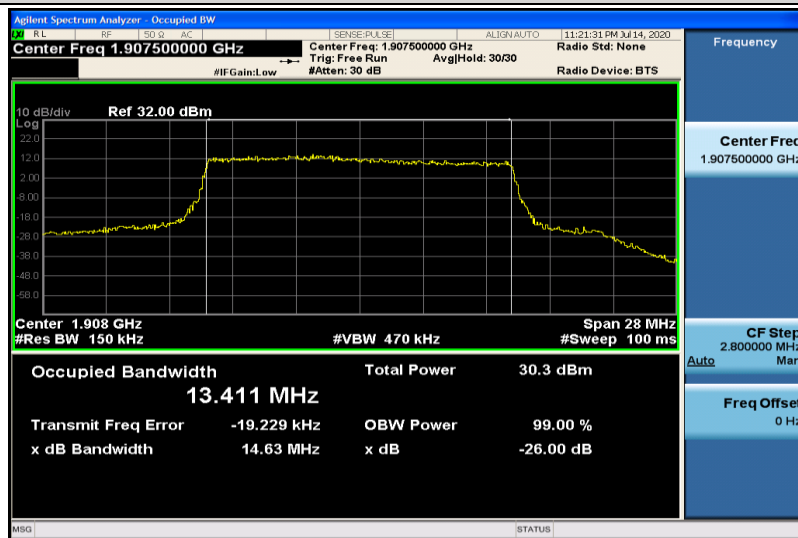
Band25-15MHz-QPSK-26615-75RB#0-13.411
