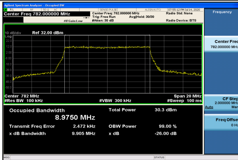
Band13-10MHz-16QAM-23230-50RB#0-8.9750
