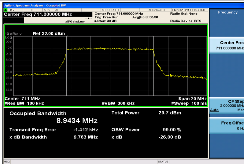
Band12-10MHz-16QAM-23130-50RB#0-8.9434
