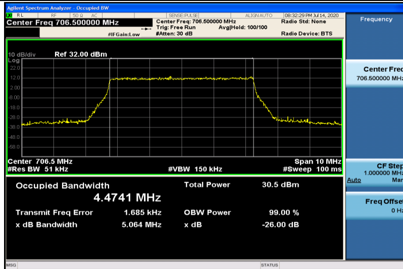
Band17-5MHz-QPSK-23755-25RB#0-4.4741
