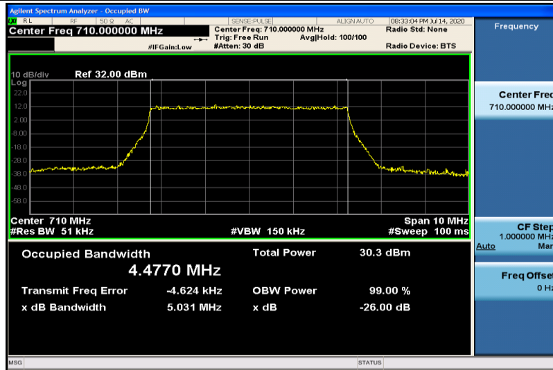
Band17-5MHz-QPSK-23790-25RB#0-4.4770
