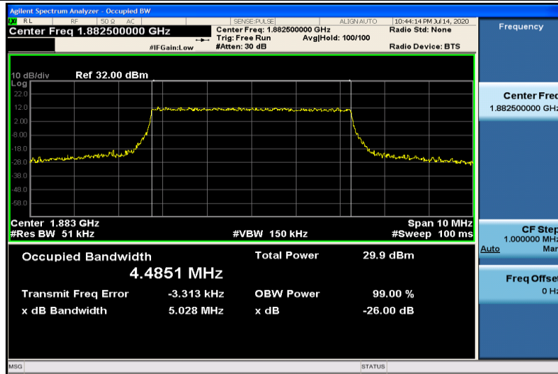
Band25-5MHz-QPSK-26365-25RB#0-4.4851
