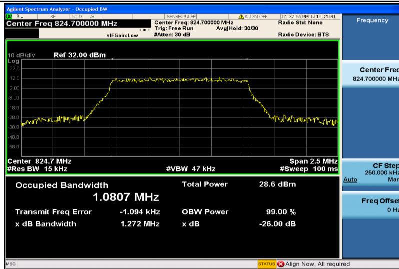
Band26-1.4MHz-16QAM-26797-6RB#0-1.0807
