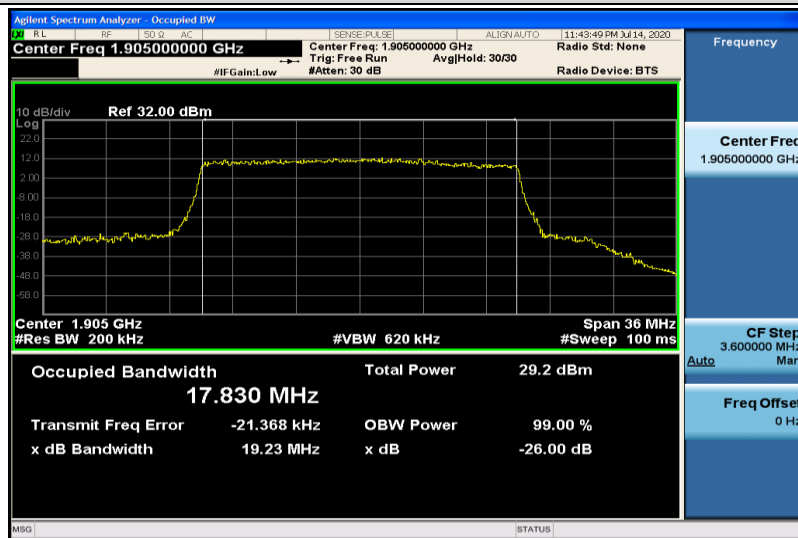
Band25-20MHz-16QAM-26590-100RB#0-17.830
