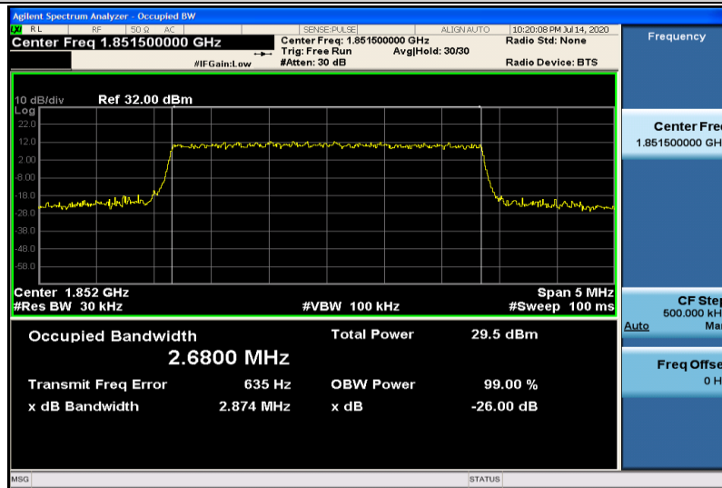
Band25-3MHz-QPSK-26055-15RB#0-2.6800
