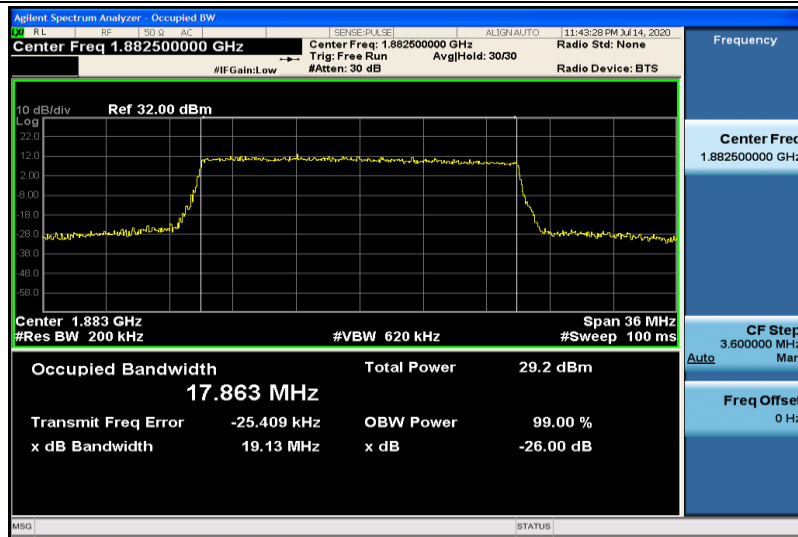
Band25-20MHz-16QAM-26365-100RB#0-17.863
