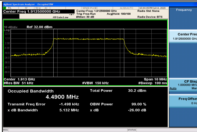
Band25-5MHz-QPSK-26665-25RB#0-4.4900
