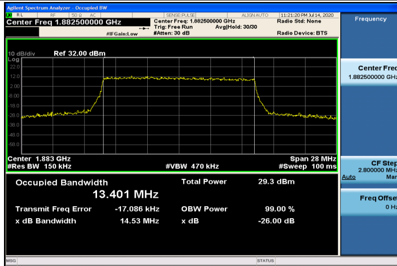
Band25-15MHz-16QAM-26365-75RB#0-13.401
