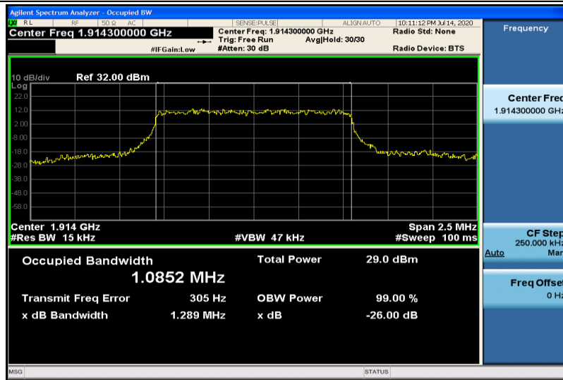
Band25-1.4MHz-QPSK-26683-6RB#0-1.0852
