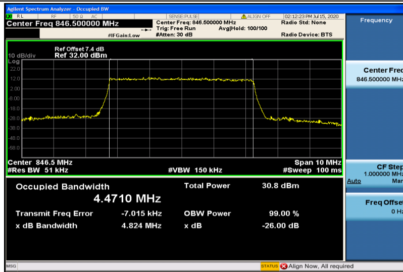
Band26-5MHz-QPSK-27015-25RB#0-4.4710
