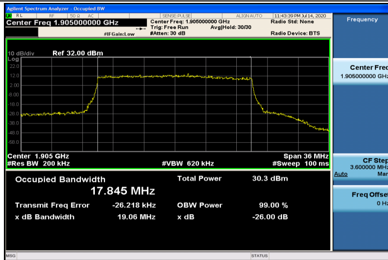
Band25-20MHz-QPSK-26590-100RB#0-17.845
