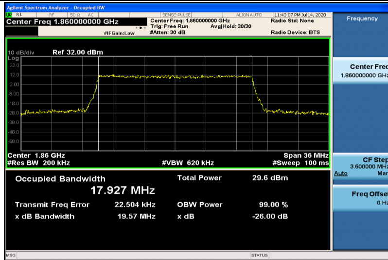
Band25-20MHz-16QAM-26140-100RB#0-17.927
