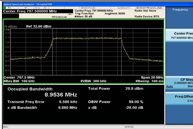
Band12-10MHz-16QAM-23095-50RB#0-8.9536
