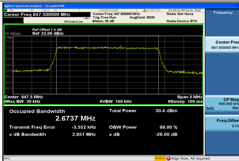
Band26-3MHz-QPSK-27025-15RB#0-2.6737
