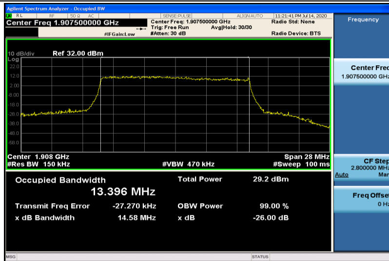
Band25-15MHz-16QAM-26615-75RB#0-13.396
