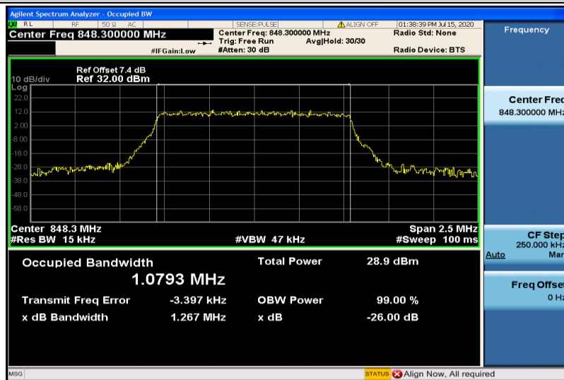
Band26-1.4MHz-16QAM-27033-6RB#0-1.0793
