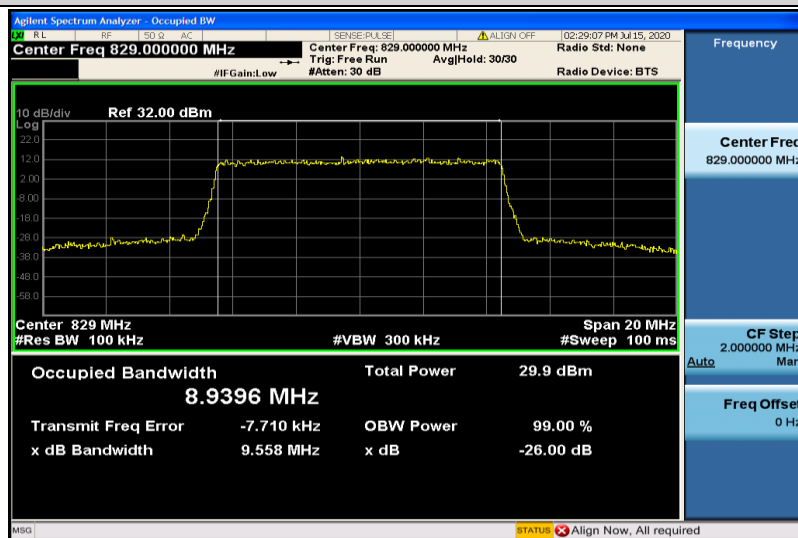
Band26-10MHz-16QAM-26840-50RB#0-8.9396
