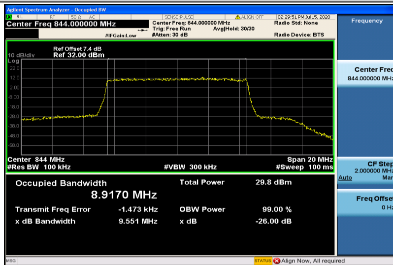
Band26-10MHz-16QAM-26990-50RB#0-8.9170
