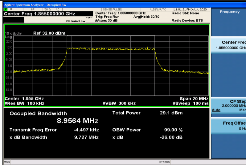
Band25-10MHz-16QAM-26090-50RB#0-8.9564
