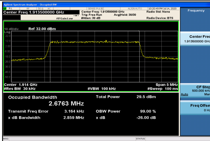
Band25-3MHz-QPSK-26675-15RB#0-2.6763
