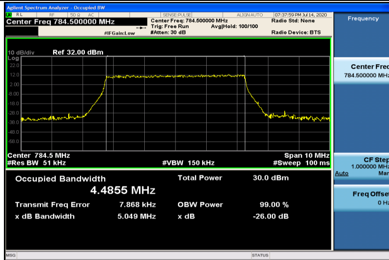
Band13-5MHz-16QAM-23255-25RB#0-4.4855
