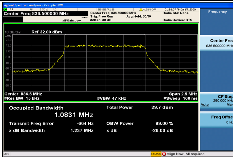
Band26-1.4MHz-QPSK-26915-6RB#0-1.0831
