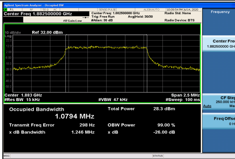
Band25-1.4MHz-16QAM-26365-6RB#0-1.0794
