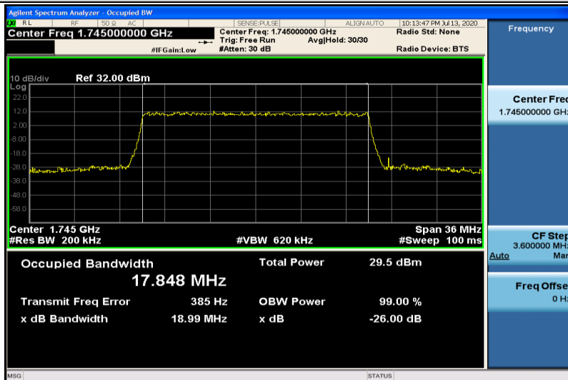
Band4-20MHz-QPSK-20300-100RB#0-17.848
