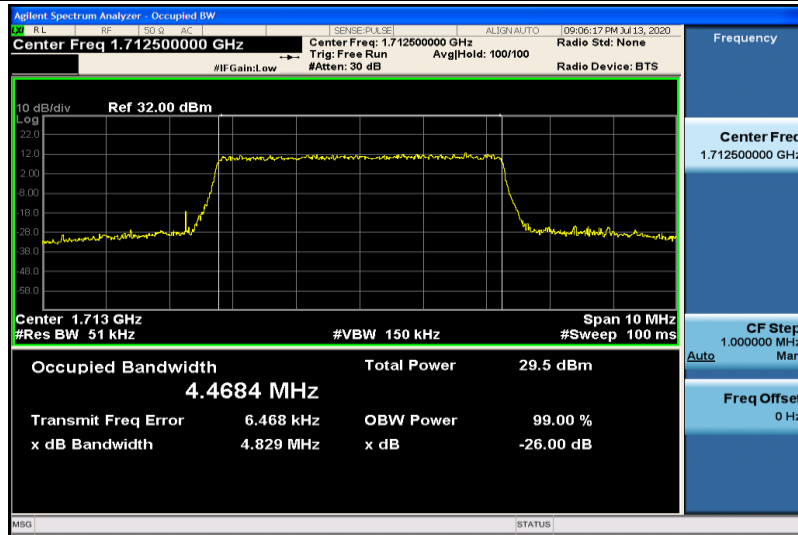
Band4-5MHz-16QAM-19975-25RB#0-4.4684
