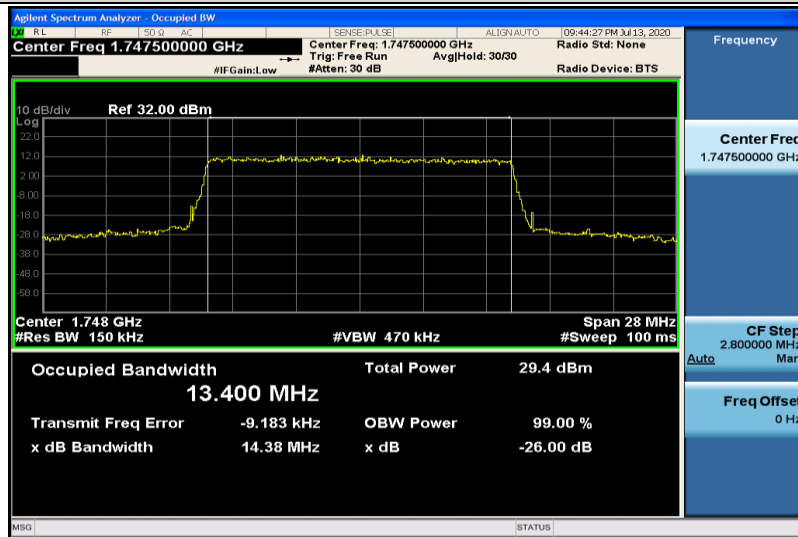
Band4-15MHz-QPSK-20325-75RB#0-13.400
