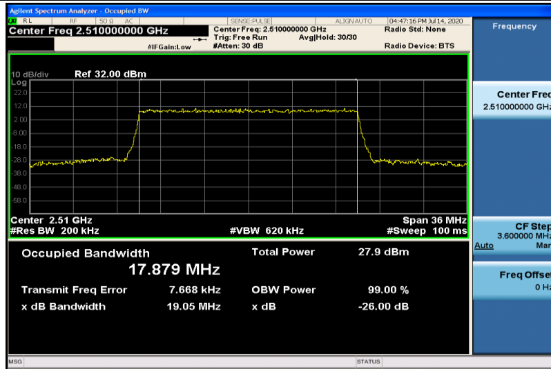
Band7-20MHz-16QAM-20850-100RB#0-17.879
