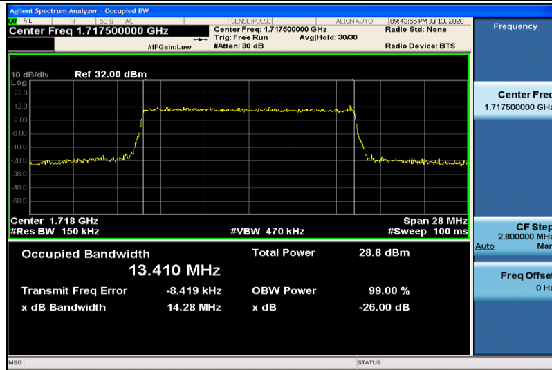
Band4-15MHz-16QAM-20025-75RB#0-13.410
