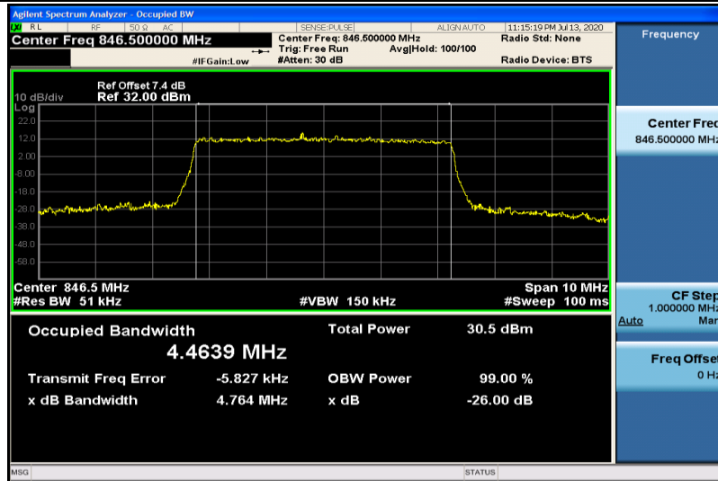
Band5-5MHz-16QAM-20625-25RB#0-4.4639
