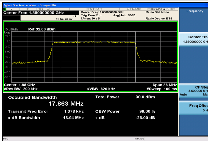
Band2-20MHz-16QAM-18900-100RB#0-17.863
