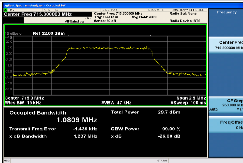
Band12-1.4MHz-QPSK-23173-6RB#0-1.0809
