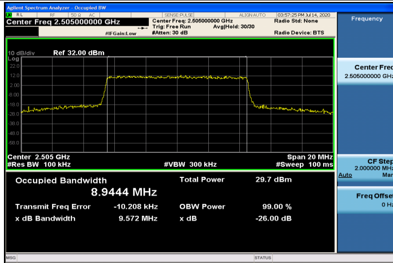
Band7-10MHz-16QAM-20800-50RB#0-8.9444
