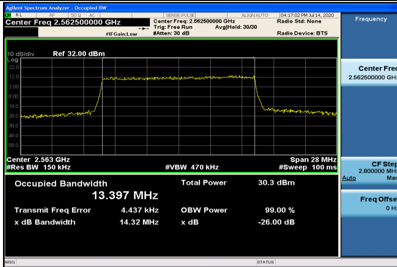
Band7-15MHz-16QAM-21375-75RB#0-13.397
