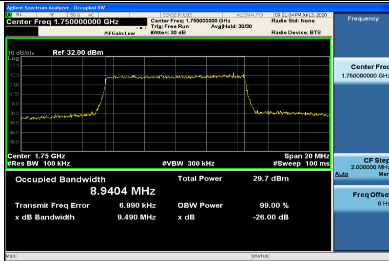
Band4-10MHz-16QAM-20350-50RB#0-8.9404
