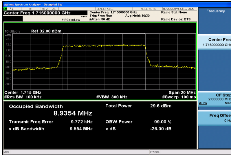
Band4-10MHz-16QAM-20000-50RB#0-8.9354
