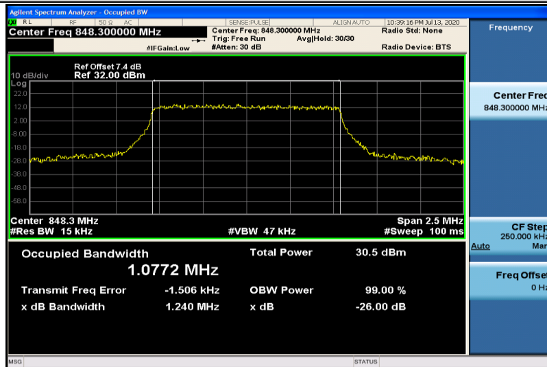
Band5-1.4MHz-QPSK-20643-6RB#0-1.0772
