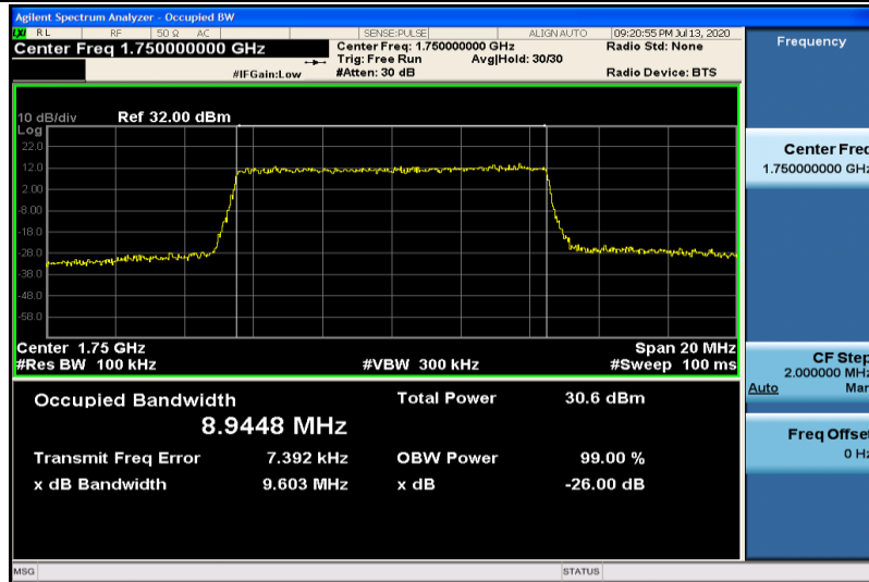
Band4-10MHz-QPSK-20350-50RB#0-8.9448
