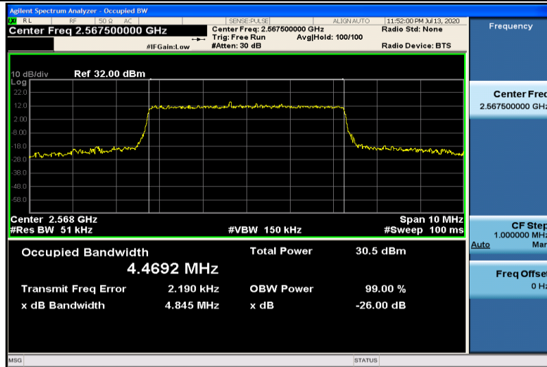
Band7-5MHz-16QAM-21425-25RB#0-4.4692
