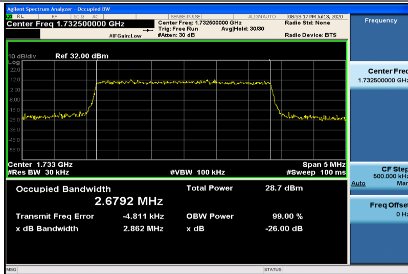
Band4-3MHz-16QAM-20175-15RB#0-2.6792
