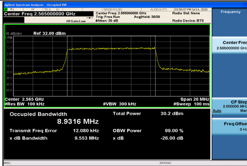
Band7-10MHz-16QAM-21400-50RB#0-8.9316
