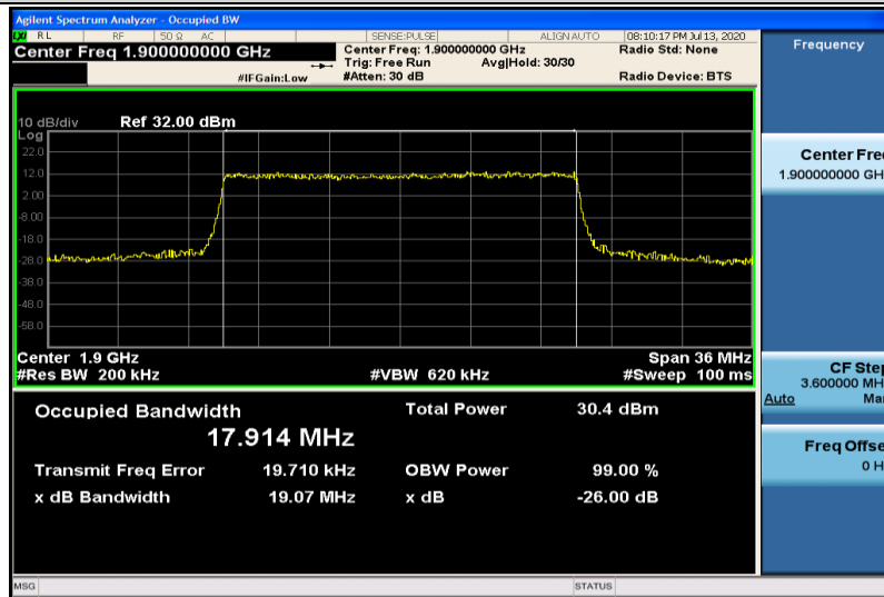
Band2-20MHz-16QAM-19100-100RB#0-17.914
