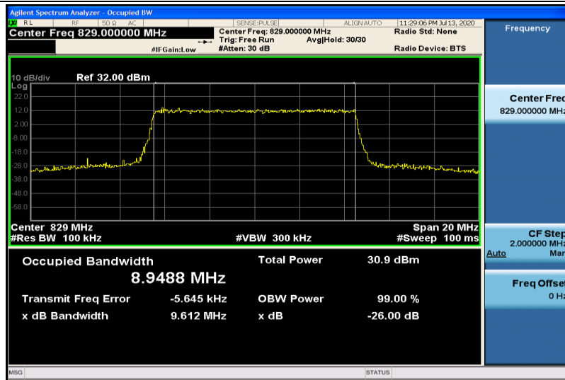
Band5-10MHz-QPSK-20450-50RB#0-8.9488
