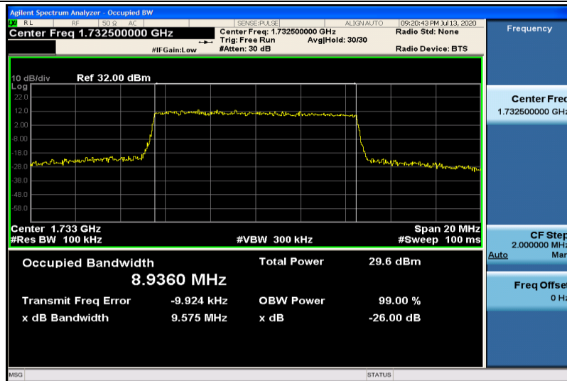
Band4-10MHz-16QAM-20175-50RB#0-8.9360
