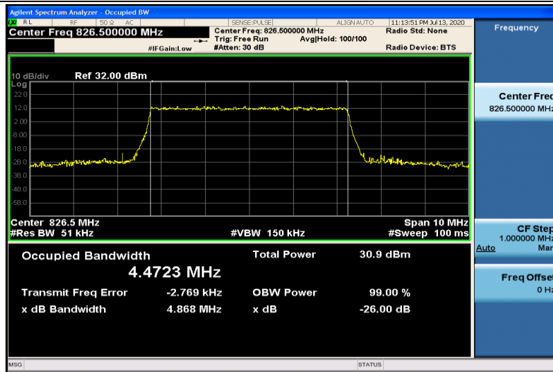
Band5-5MHz-QPSK-20425-25RB#0-4.4723
