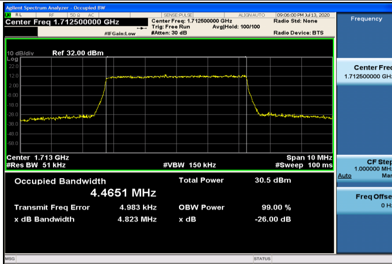
Band4-5MHz-QPSK-19975-25RB#0-4.4651
