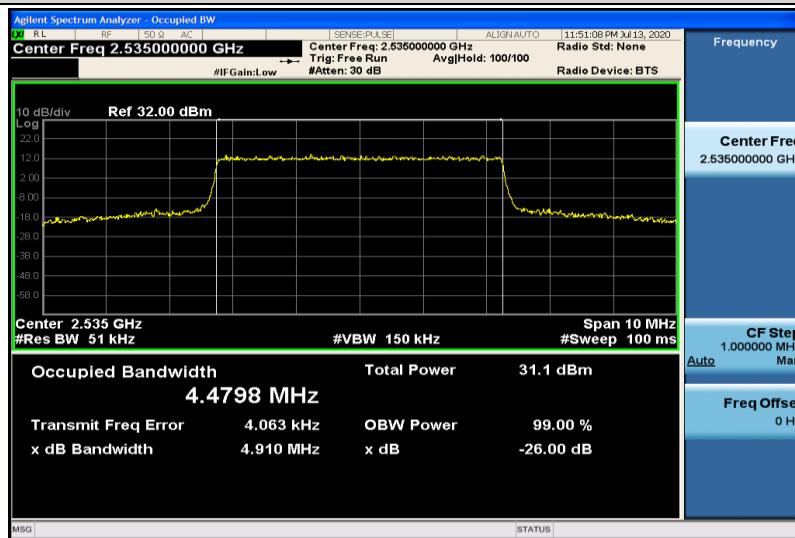
Band7-5MHz-QPSK-21100-25RB#0-4.4798
