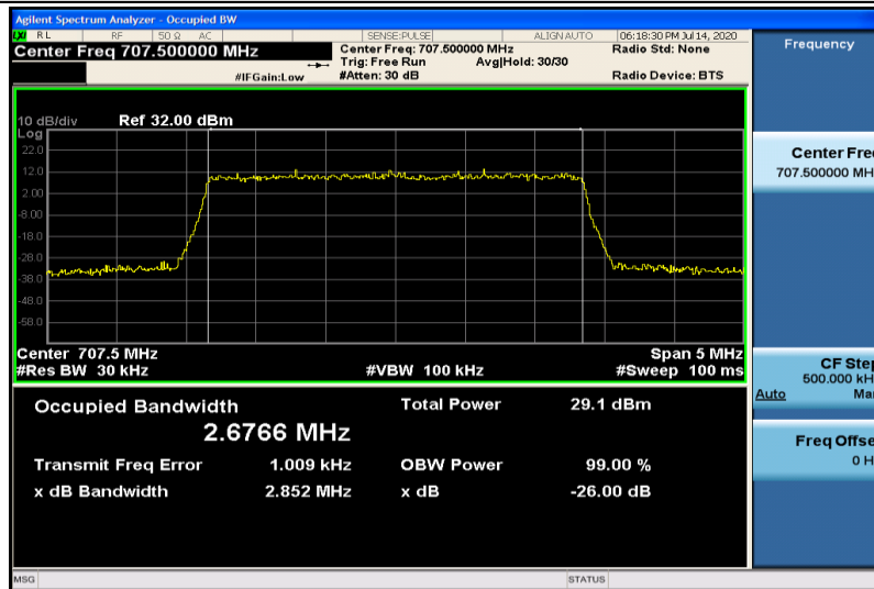
Band12-3MHz-16QAM-23095-15RB#0-2.6766
