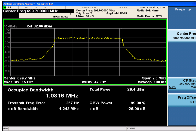
Band12-1.4MHz-QPSK-23017-6RB#0-1.0816
