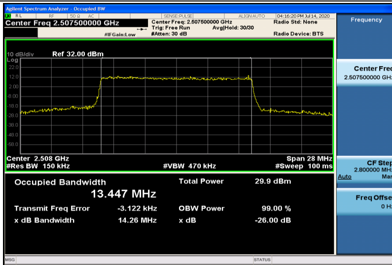
Band7-15MHz-16QAM-20825-75RB#0-13.447
