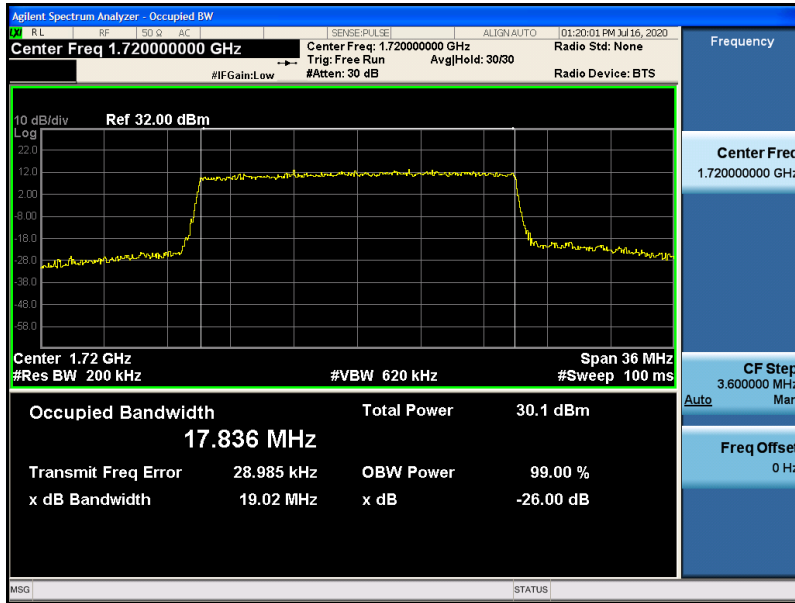
Band4-20MHz-QPSK-20050-100RB#0-17.835
