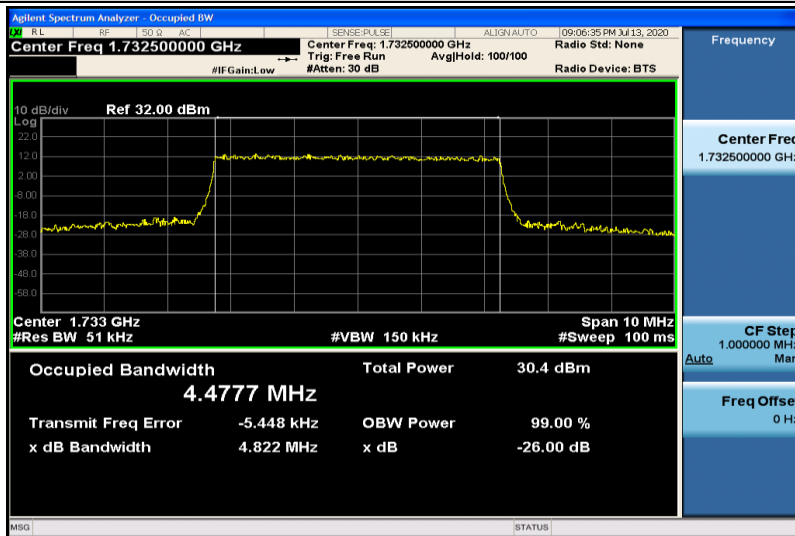
Band4-5MHz-QPSK-17325-25RB#0-4.4777
