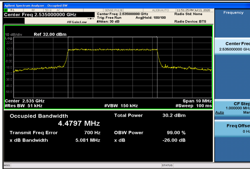
Band7-5MHz-16QAM-21100-25RB#0-4.4797
