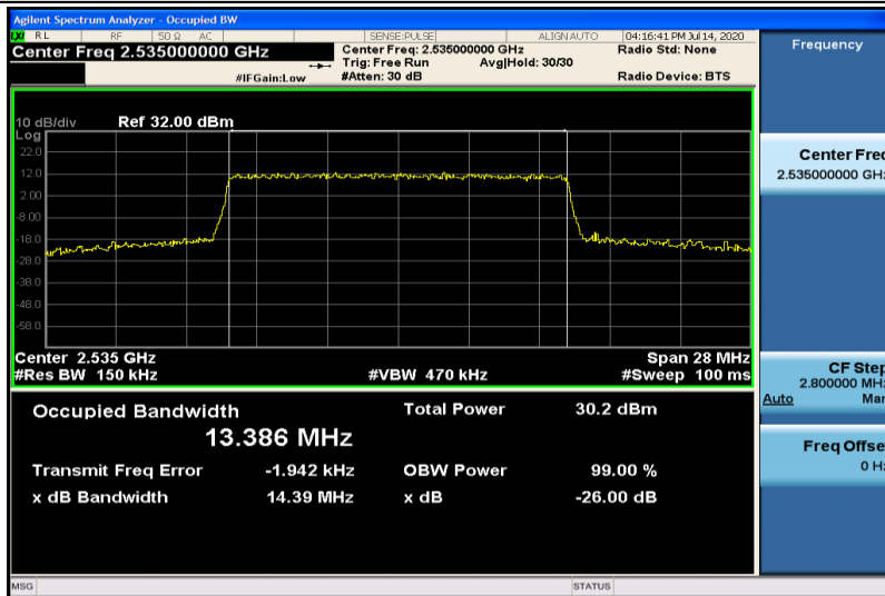
Band7-15MHz-16QAM-21100-75RB#0-13.386
