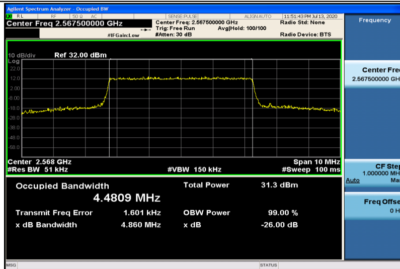
Band7-5MHz-QPSK-21425-25RB#0-4.4809
