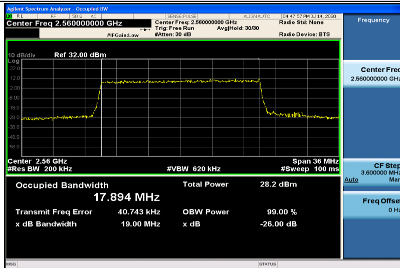
Band7-20MHz-16QAM-21350-100RB#0-17.894
