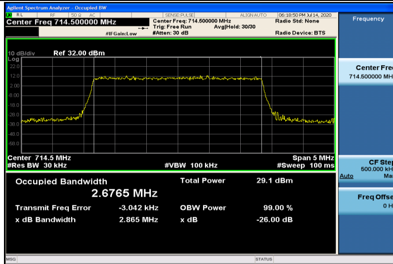
Band12-3MHz-16QAM-23165-15RB#0-2.6765
