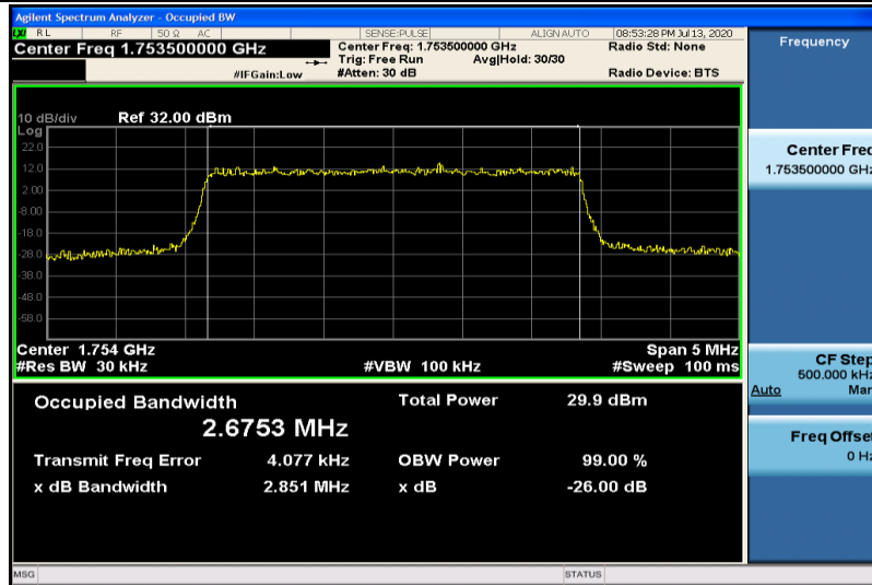
Band4-3MHz-QPSK-20385-15RB#0-2.6753
