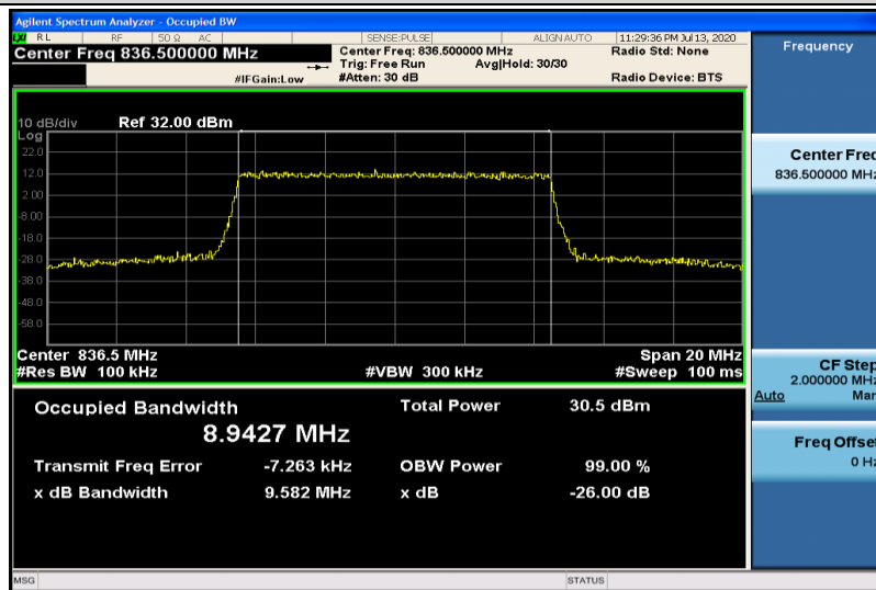
Band5-10MHz-16QAM-20525-50RB#0-8.9427
