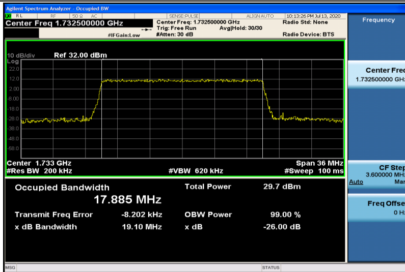
Band4-20MHz-QPSK-20175-100RB#0-17.885
