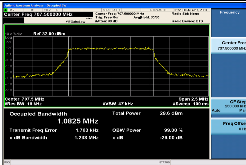
Band12-1.4MHz-QPSK-23095-6RB#0-1.0825
