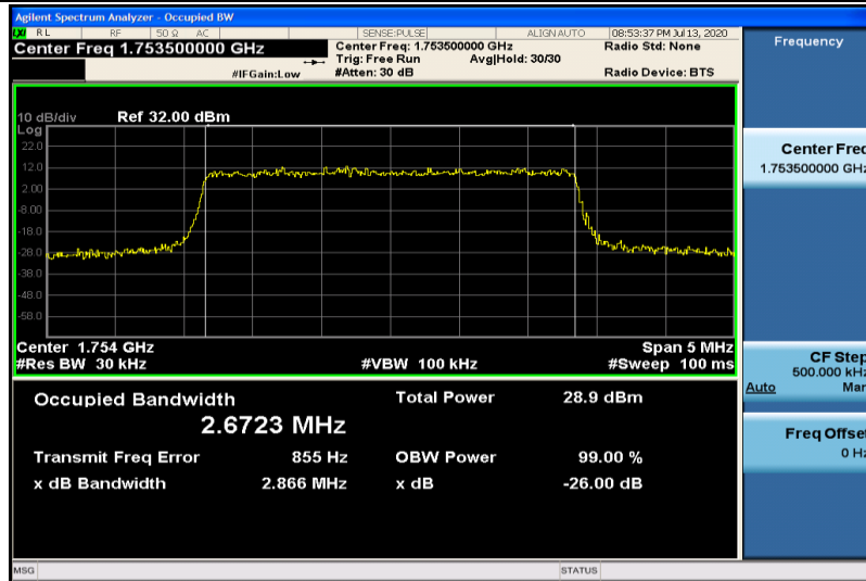
Band4-3MHz-16QAM-20385-15RB#0-2.6723
