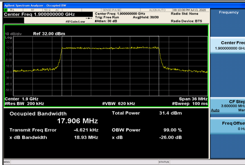
Band2-20MHz-QPSK-19100-100RB#0-17.906
