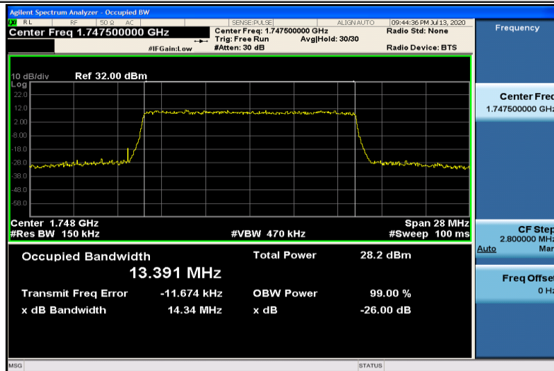
Band4-15MHz-16QAM-20325-75RB#0-13.391
