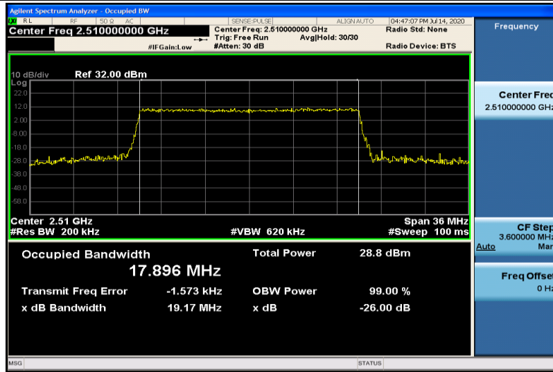
Band7-20MHz-QPSK-20850-100RB#0-17.896
