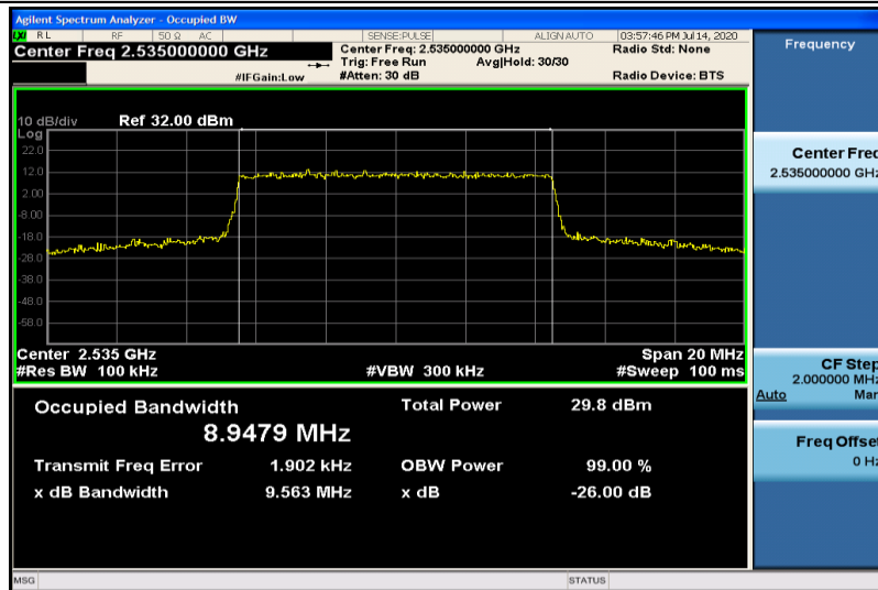
Band7-10MHz-16QAM-21100-50RB#0-8.9479
