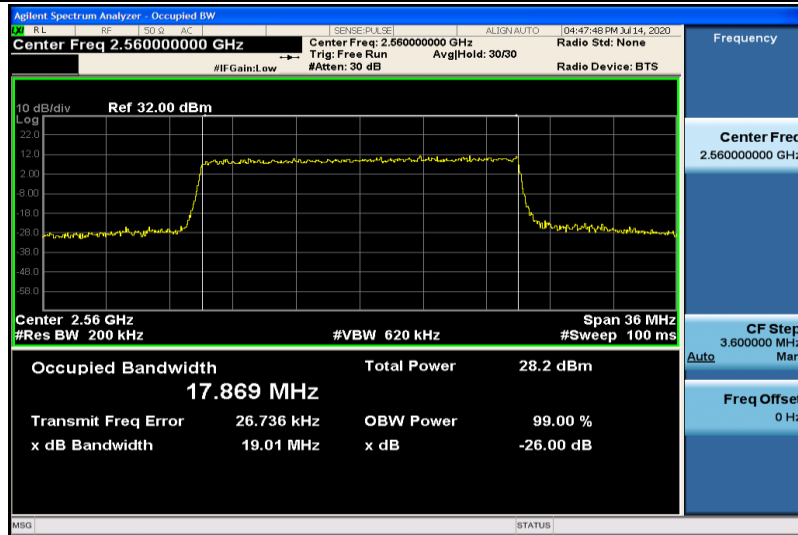
Band7-20MHz-QPSK-21350-100RB#0-17.869
