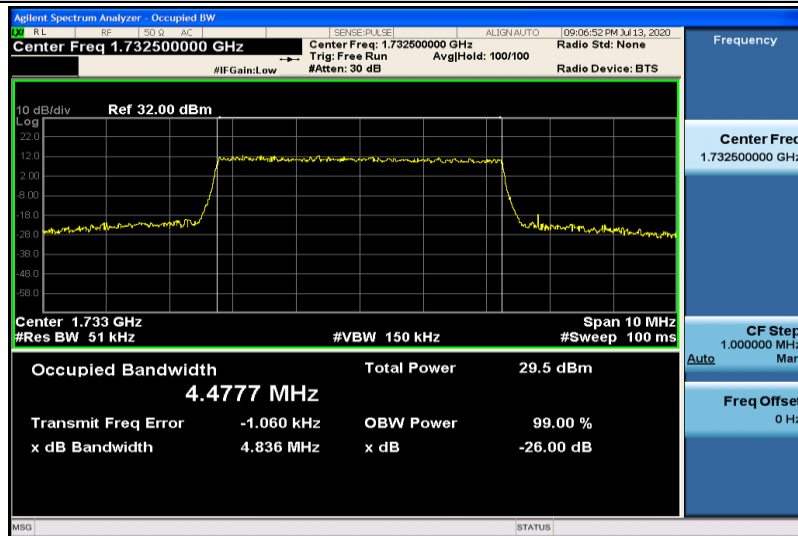
Band4-5MHz-16QAM-20175-25RB#0-4.4777
