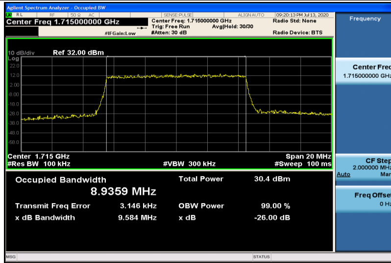
Band4-10MHz-QPSK-20000-50RB#0-8.9359
