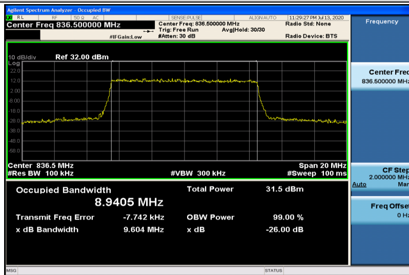
Band5-10MHz-QPSK-20525-50RB#0-8.9405
