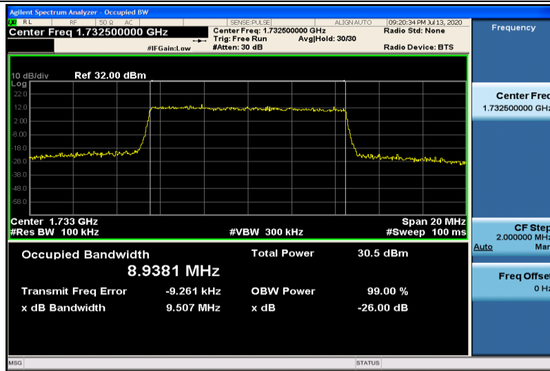
Band4-10MHz-QPSK-20175-50RB#0-8.9381
