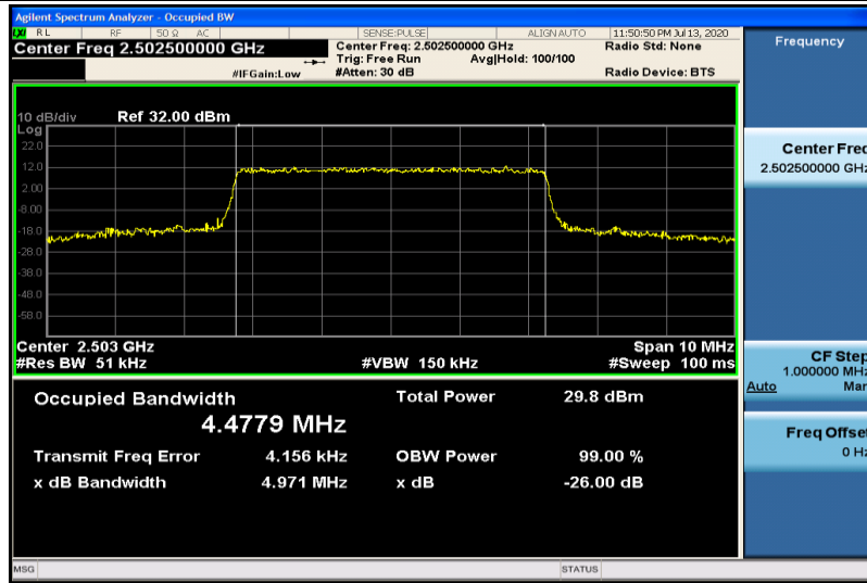
Band7-5MHz-16QAM-20775-25RB#0-4.4779
