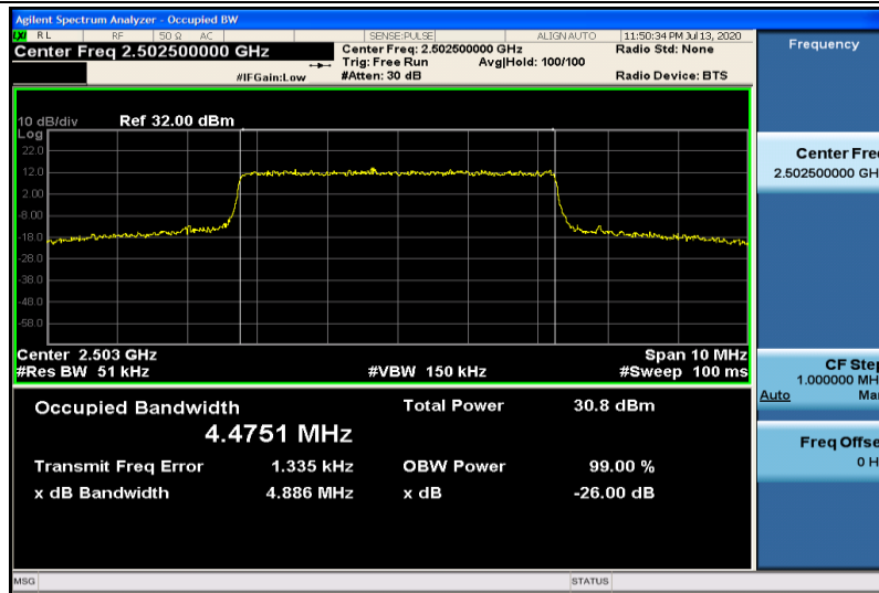
Band7-5MHz-QPSK-20775-25RB#0-4.4751
