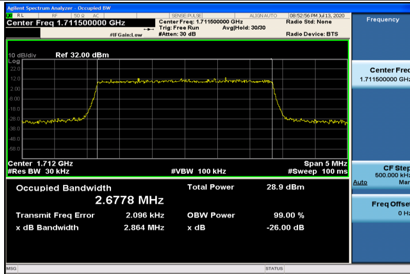
Band4-3MHz-16QAM-19965-15RB#0-2.6778
