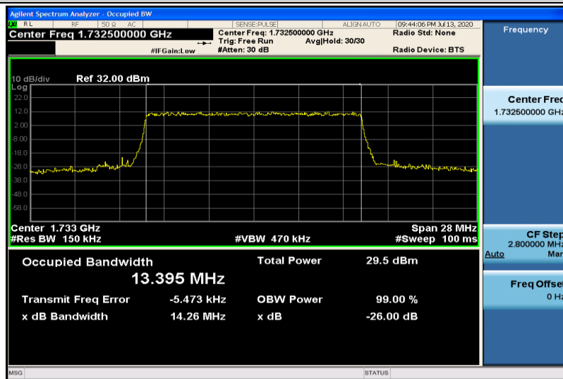
Band4-15MHz-QPSK-20175-75RB#0-13.395
