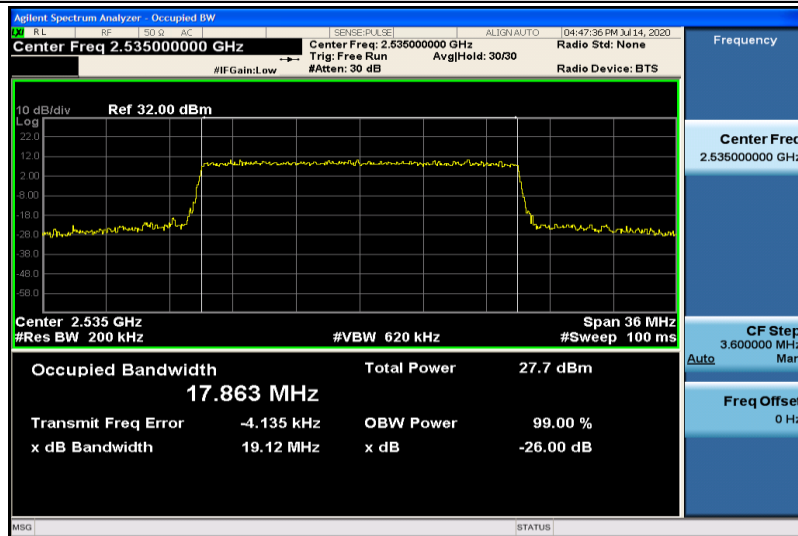
Band7-20MHz-16QAM-21100-100RB#0-17.863
