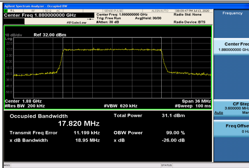
Band2-20MHz-QPSK-18900-100RB#0-17.820
