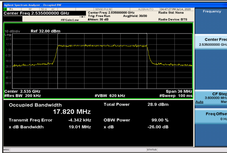
Band7-20MHz-QPSK-21100-100RB#0-17.820
