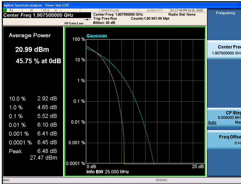
Band25-15MHz-16QAM-26615-75RB#0
