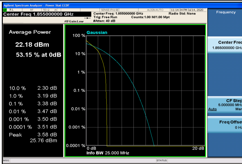
Band25-10MHz-QPSK-26090-1RB#0
