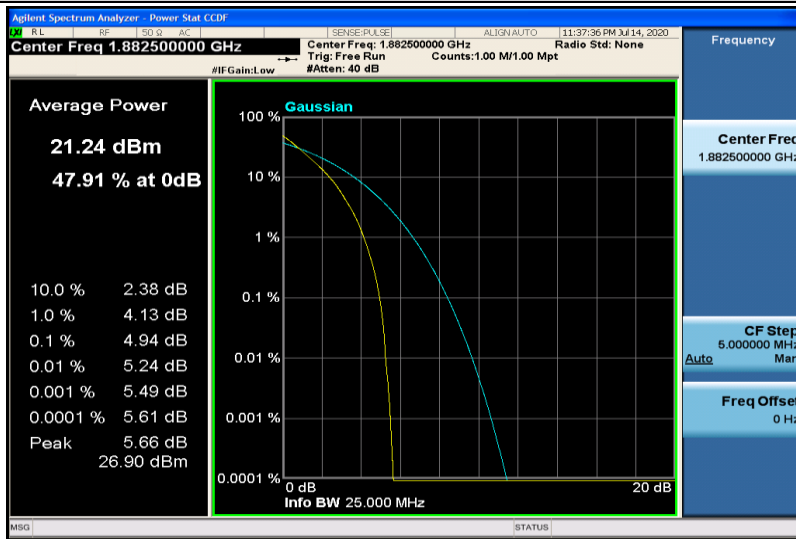
Band25-15MHz-QPSK-26365-75RB#0
