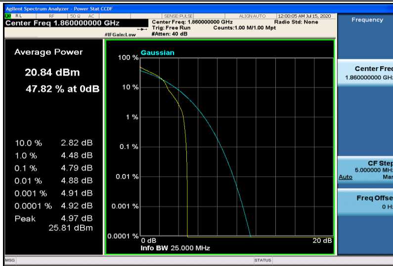
Band25-20MHz-16QAM-26140-1RB#0
