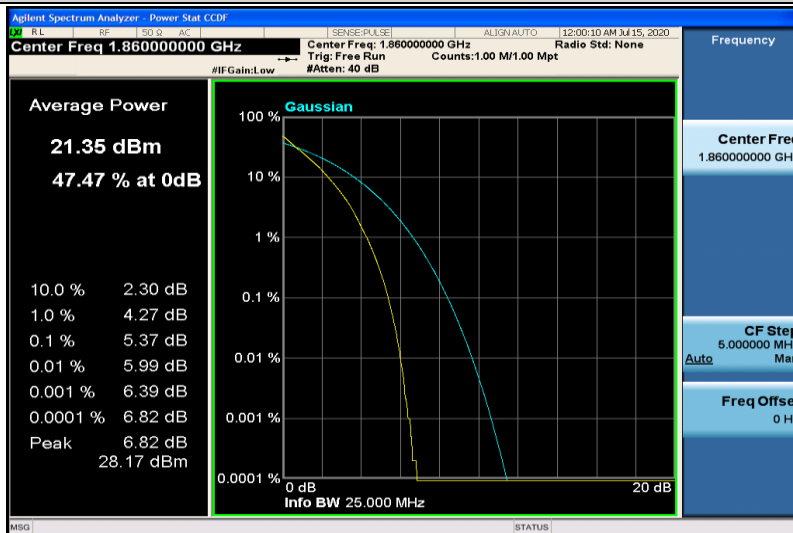
Band25-20MHz-QPSK-26140-100RB#0
