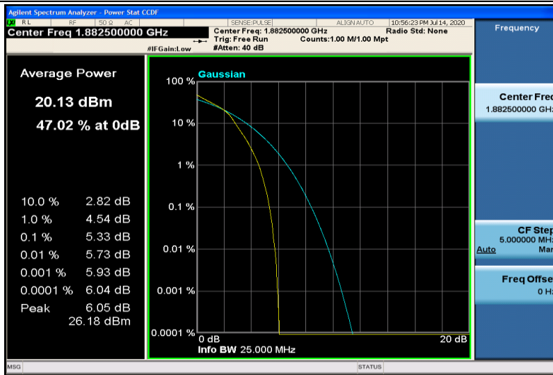
Band25-5MHz-16QAM-26365-25RB#0
