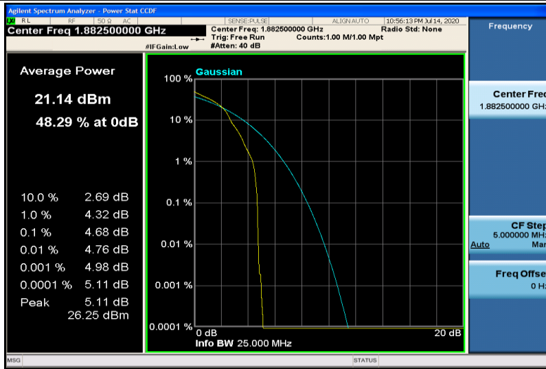
Band25-5MHz-16QAM-26365-1RB#0
