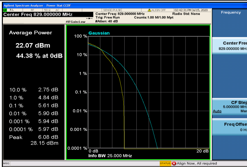
Band26-10MHz-16QAM-26840-1RB#0
