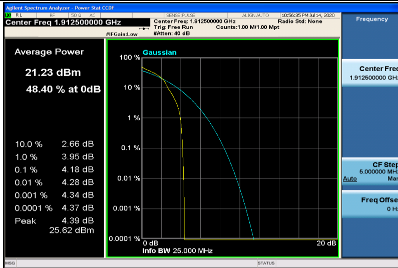
Band25-5MHz-16QAM-26665-1RB#0
