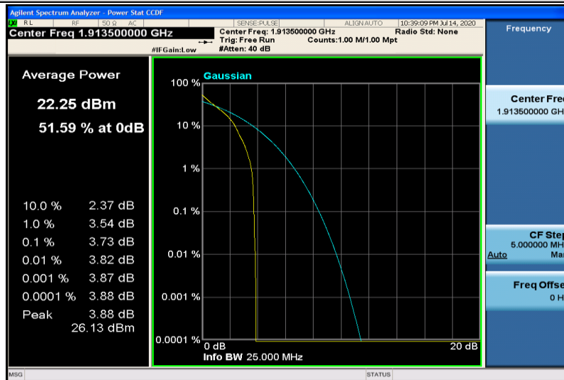
Band25-3MHz-QPSK-26675-1RB#0
