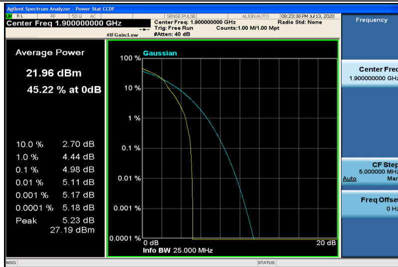
Band2-20MHz-16QAM-19100-1R1B#0
