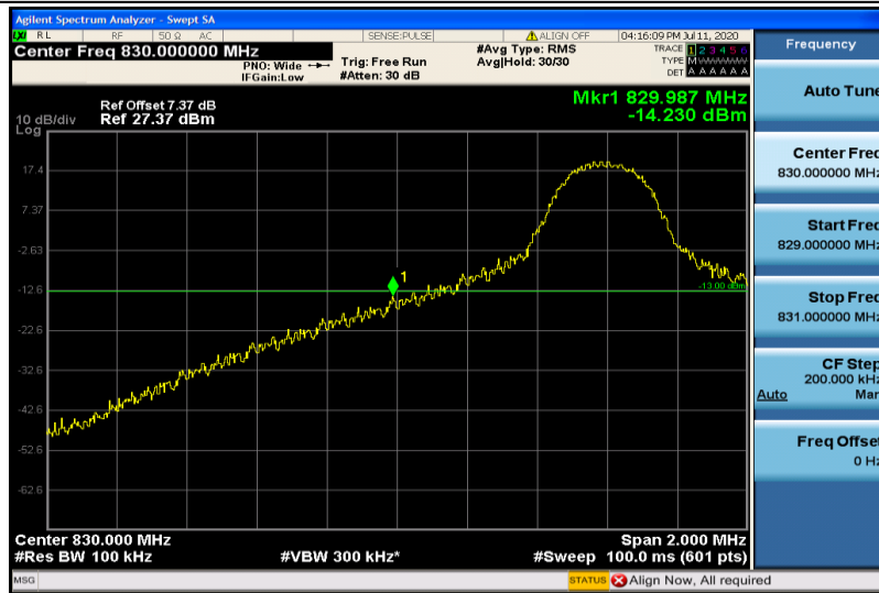
Band19-10MHz-16QAM-24050-1RB#0
