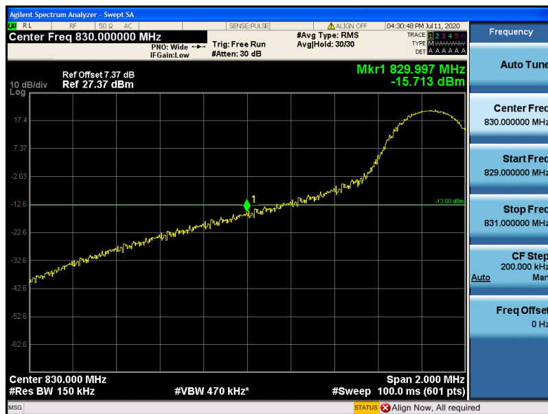
Band19-15MHz-QPSK-24075-1RB#0
