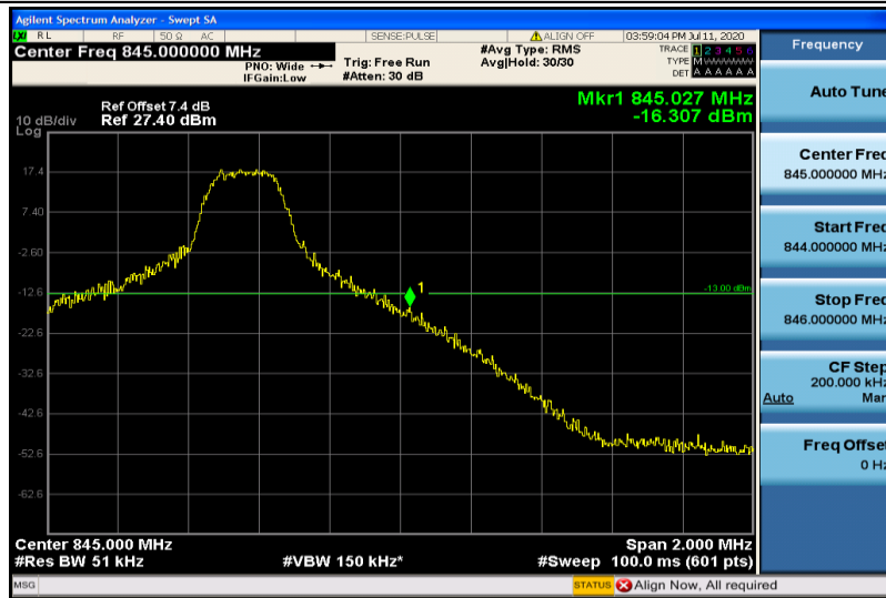
Band19-5MHz-16QAM-24125-1RB#24
