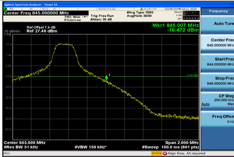
Band19-5MHz-QPSK-24125-1RB#24
