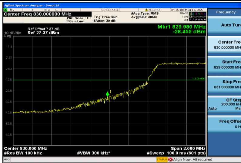
Band19-10MHz-QPSK-24050-50RB#0
