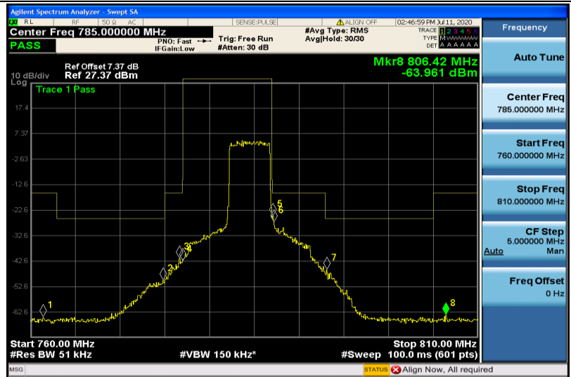
Band13-5MHz-QPSK-23255-25RB#0
