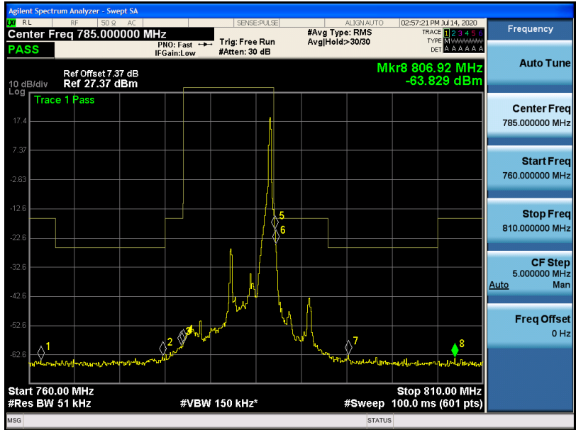
Band13-5MHz-QPSK-23255-1RB#24
