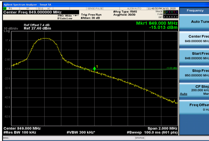
Band5-10MHz-QPSK-20600-1RB#49
