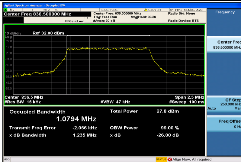
Band5-1.4MHz-QPSK-20525-6RB#0-1.0794
