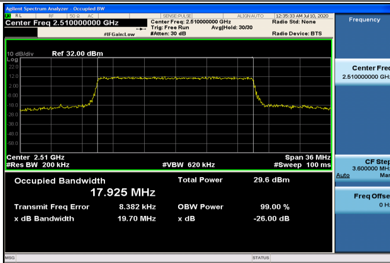
Band7-20MHz-QPSK-20850-100RB#0-17.925
