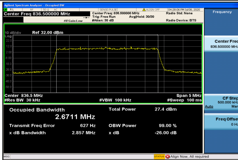
Band5-3MHz-16QAM-20525-15RB#0-2.6711
