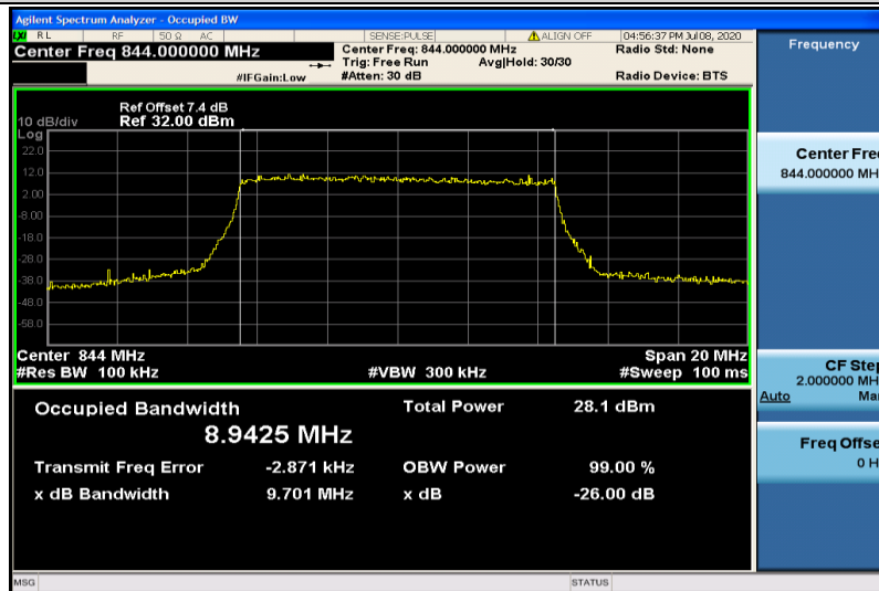
Band5-10MHz-16QAM-20600-50RB#0-8.9425
