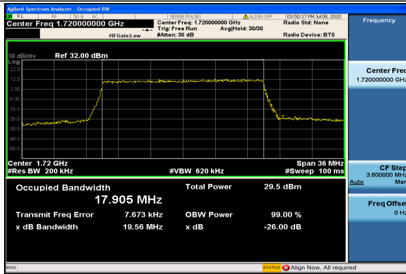
Band4-20MHz-QPSK-20050-100RB#0-17.905
