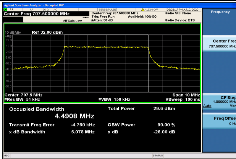
Band12-5MHz-QPSK-23095-25RB#0-4.4908
