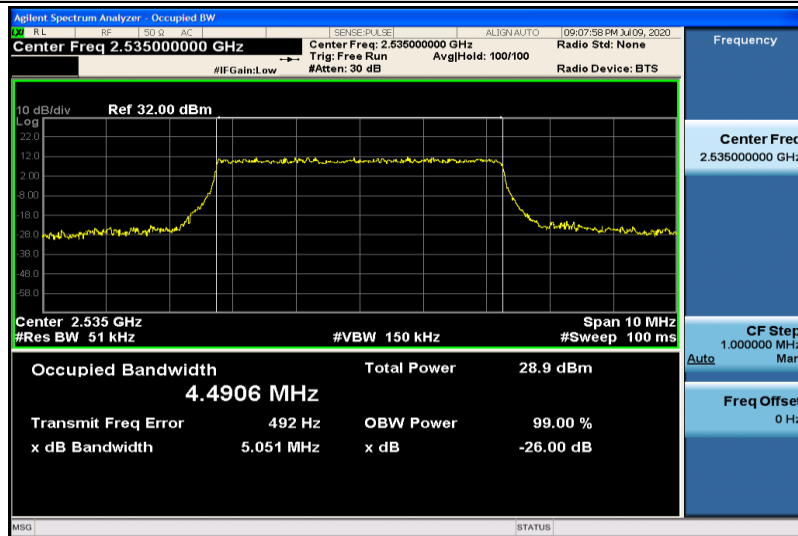
Band7-5MHz-QPSK-21100-25RB#0-4.4906
