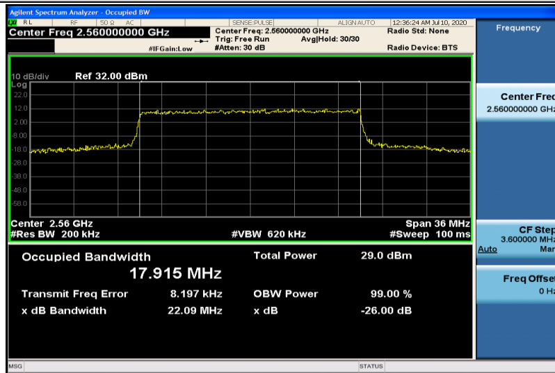
Band7-20MHz-16QAM-21350-100RB#0-17.915
