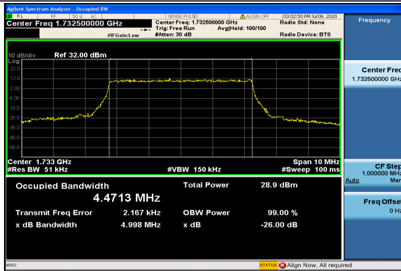
Band4-5MHz-QPSK-17325-25RB#0-4.4713
