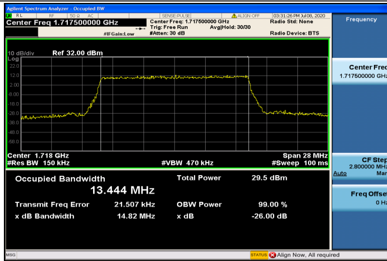
Band4-15MHz-QPSK-20025-75RB#0-13.444
