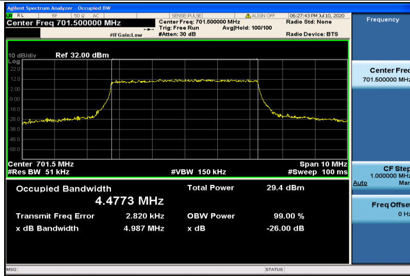
Band12-5MHz-QPSK-23035-25RB#0-4.4773
