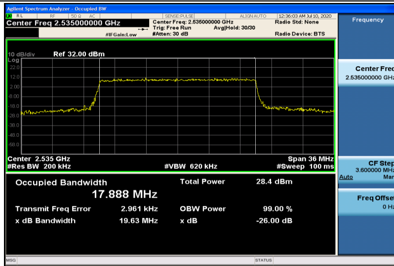
Band7-20MHz-16QAM-21100-100RB#0-17.888
