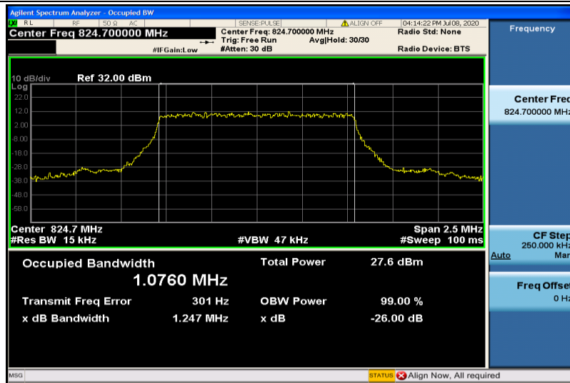
Band5-1.4MHz-QPSK-20407-6RB#0-1.0760
