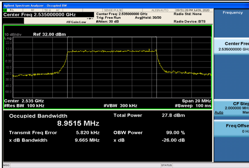
Band7-10MHz-16QAM-21100-50RB#0-8.9515
