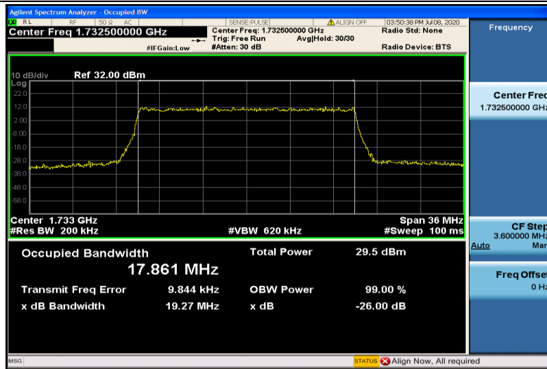
Band4-20MHz-QPSK-20175-100RB#0-17.861
