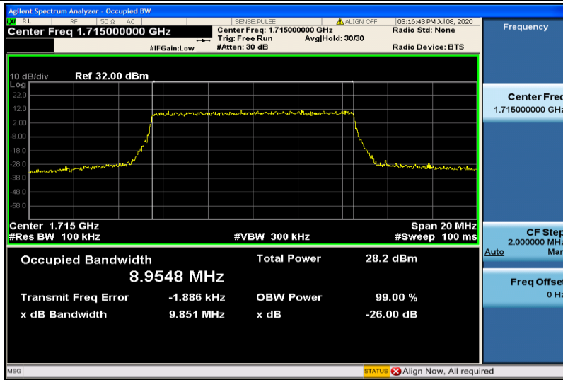
Band4-10MHz-16QAM-20000-50RB#0-8.9548
