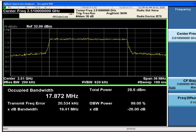
Band7-20MHz-16QAM-20850-100RB#0-17.872
