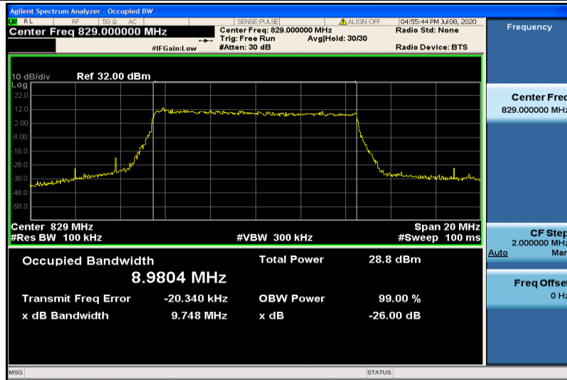
Band5-10MHz-QPSK-20450-50RB#0-8.9804
