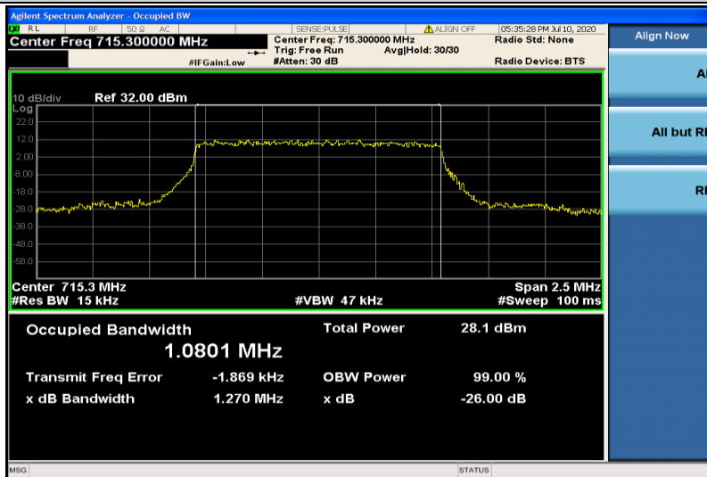
Band12-1.4MHz-QPSK-23173-6RB#0-1.0801
