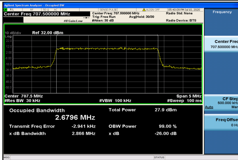
Band12-3MHz-16QAM-23095-15RB#0-2.6796
