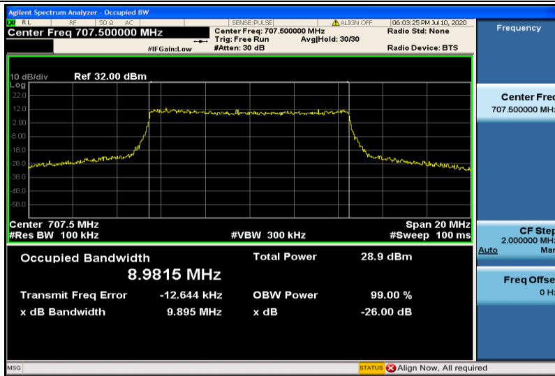
Band12-10MHz-16QAM-23095-50RB#0-8.9815
