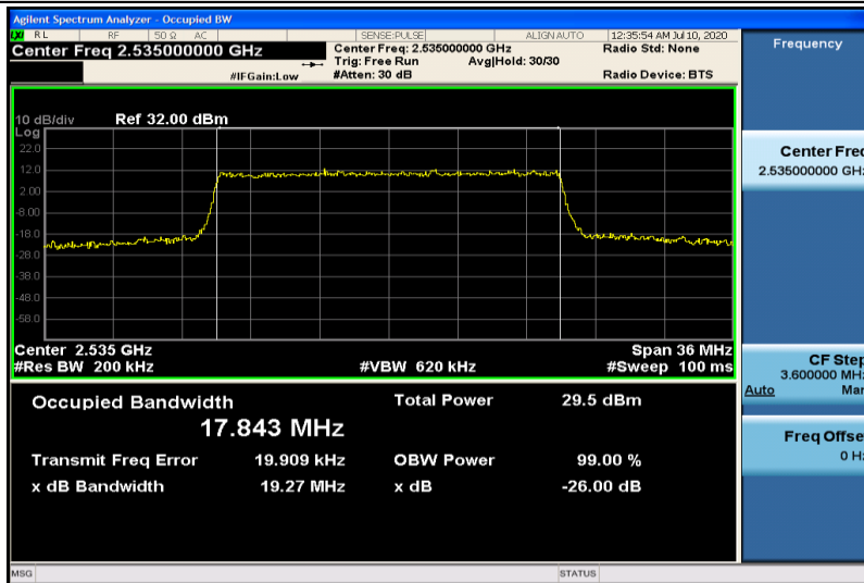
Band7-20MHz-QPSK-21100-100RB#0-17.843
