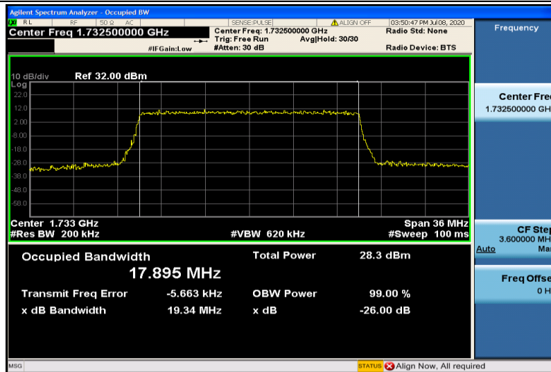
Band4-20MHz-16QAM-20175-100RB#0-17.895
