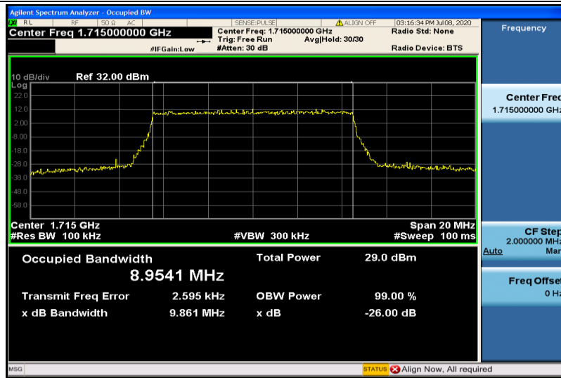
Band4-10MHz-QPSK-20000-50RB#0-8.9541
