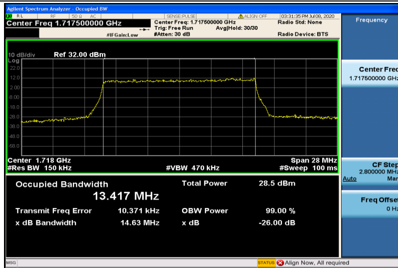
Band4-15MHz-16QAM-20025-75RB#0-13.417
