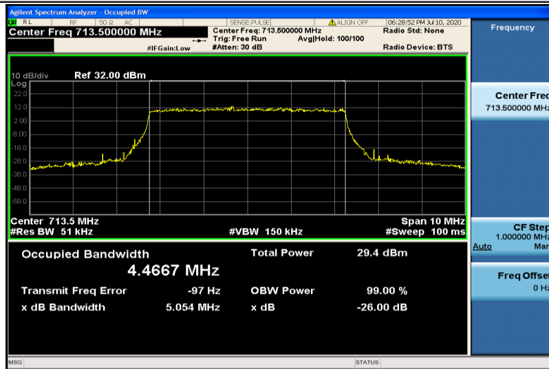
Band12-5MHz-QPSK-23155-25RB#0-4.4667
