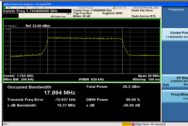
Band4-20MHz-16QAM-20300-100RB#0-17.894
