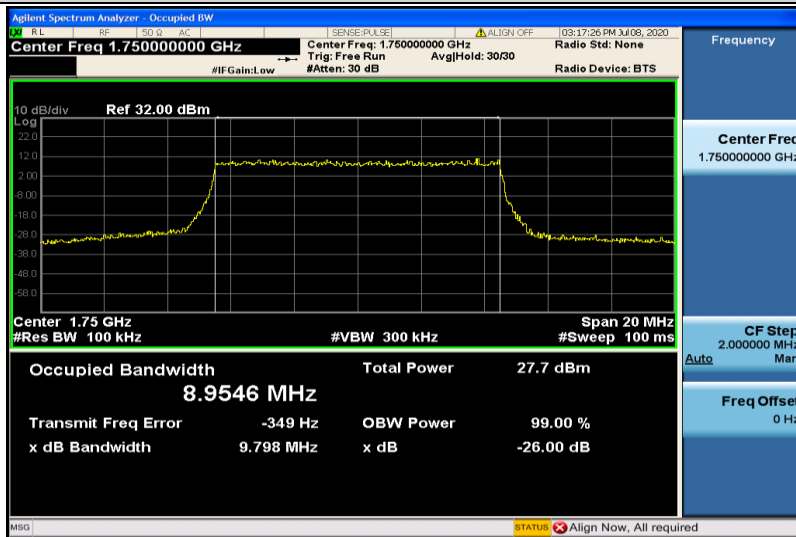
Band4-10MHz-16QAM-20350-50RB#0-8.9546
