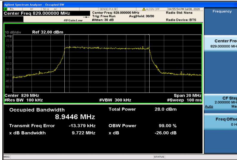
Band5-10MHz-16QAM-20450-50RB#0-8.9446
