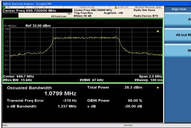
Band12-1.4MHz-QPSK-23017-6RB#0-1.0799
