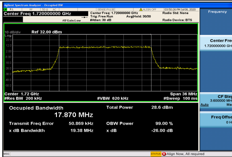
Band4-20MHz-16QAM-20050-100RB#0-17.870
