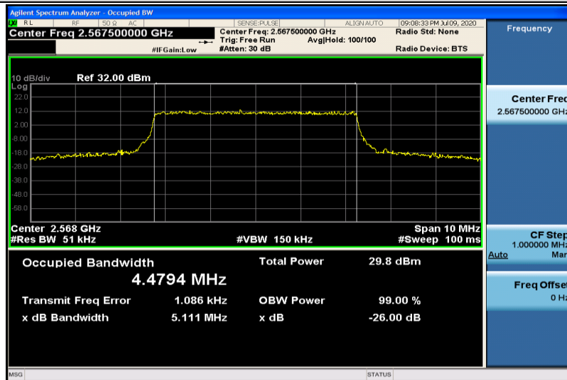
Band7-5MHz-QPSK-21425-25RB#0-4.4794
