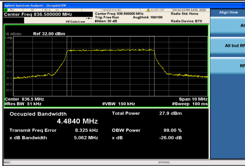
Band5-5MHz-16QAM-20525-25RB#0-4.4840
