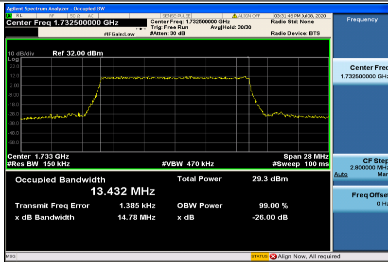
Band4-15MHz-QPSK-20175-75RB#0-13.432
