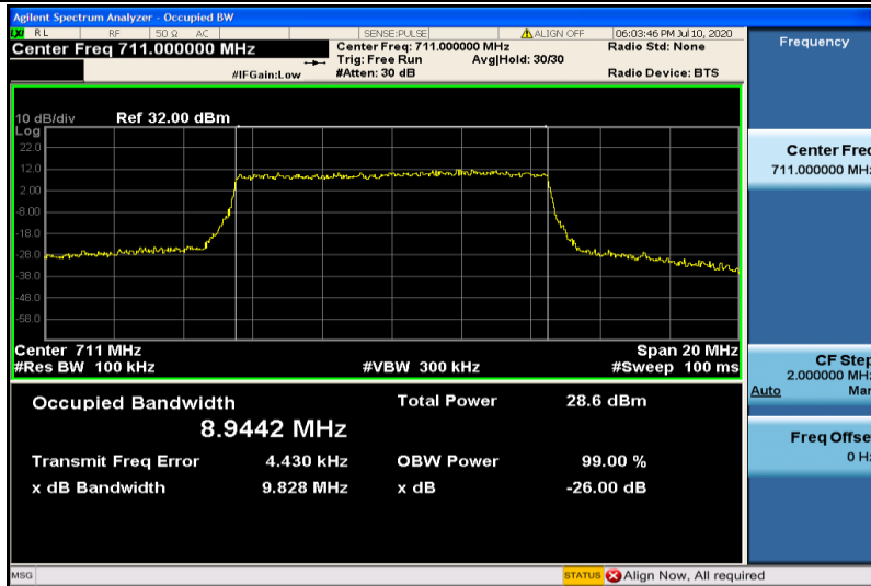
Band12-10MHz-16QAM-23130-50RB#0-8.9442
