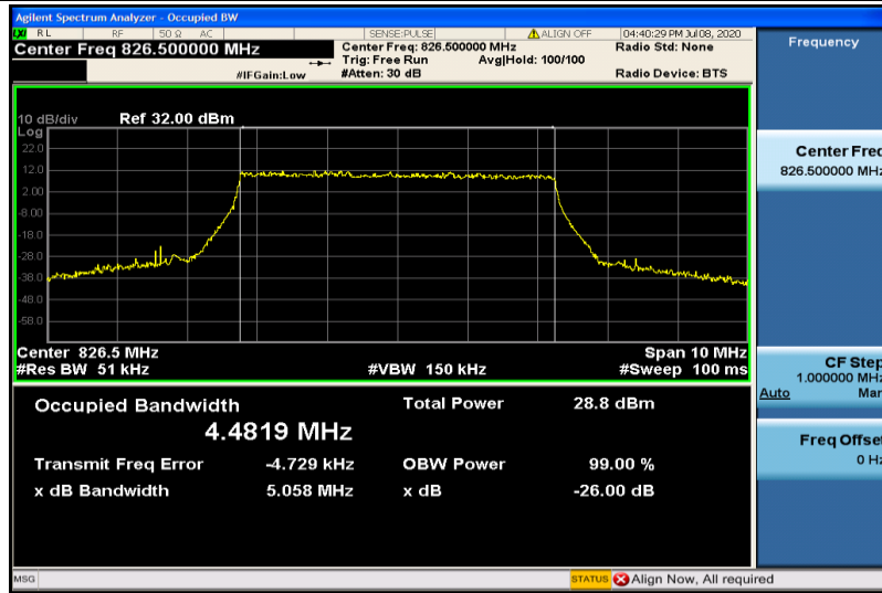
Band5-5MHz-QPSK-20425-25RB#0-4.4819
