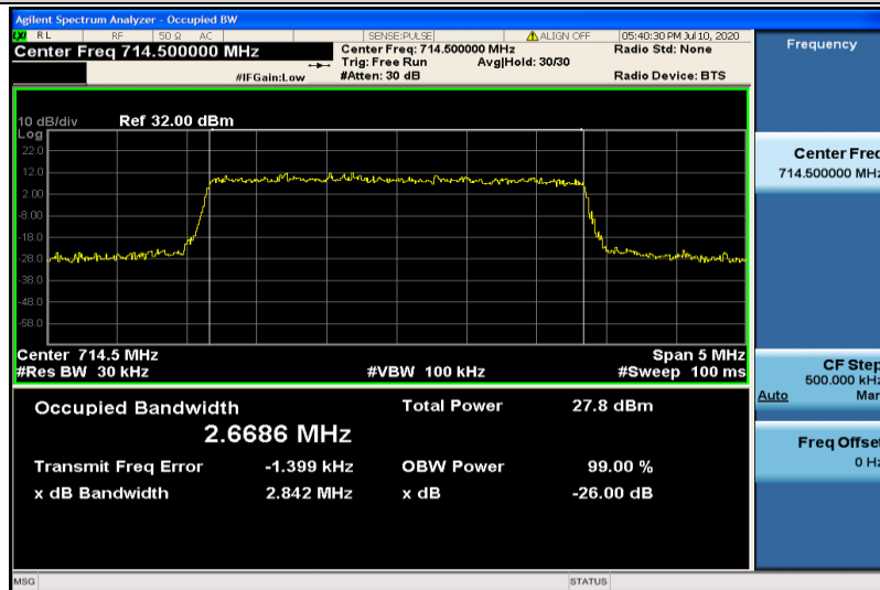
Band12-3MHz-16QAM-23165-15RB#0-2.6686
