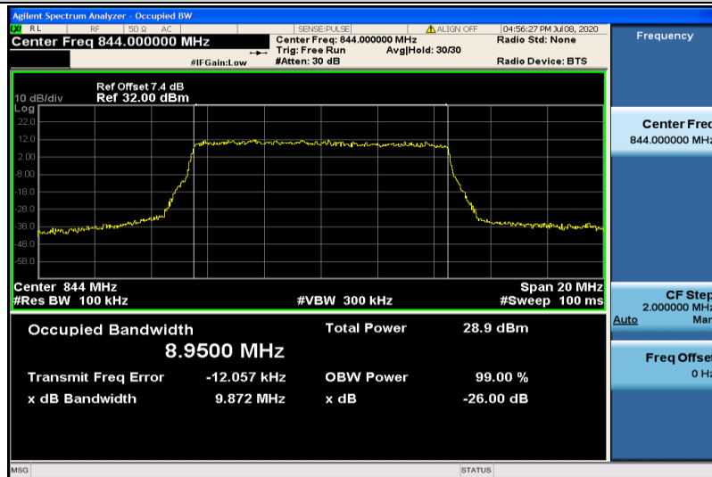
Band5-10MHz-QPSK-20600-50RB#0-8.9500
