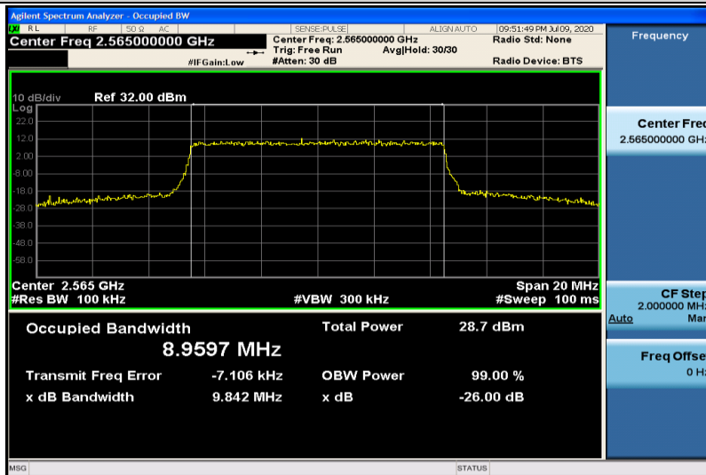
Band7-10MHz-16QAM-21400-50RB#0-8.9597
