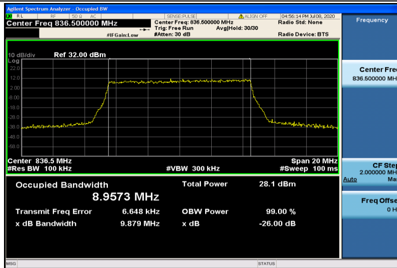
Band5-10MHz-16QAM-20525-50RB#0-8.9573
