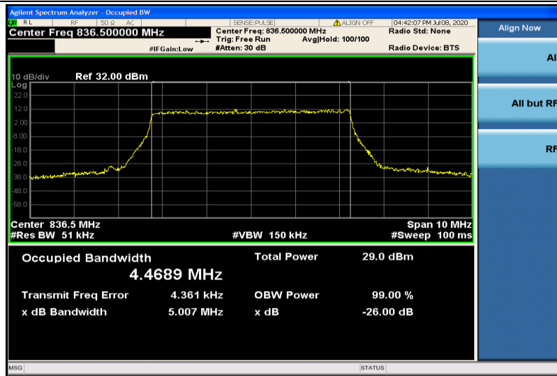
Band5-5MHz-QPSK-20525-25RB#0-4.4689
