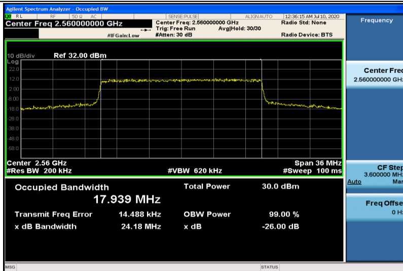
Band7-20MHz-QPSK-21350-100RB#0-17.939
