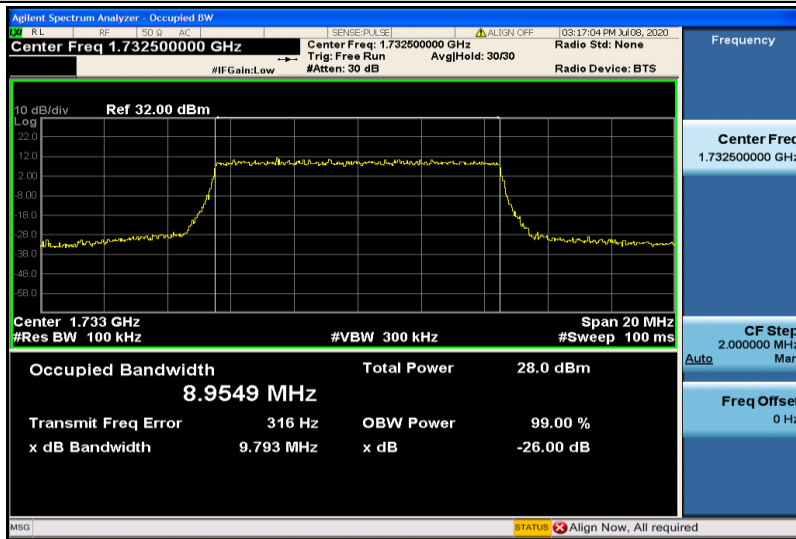
Band4-10MHz-16QAM-20175-50RB#0-8.9549
