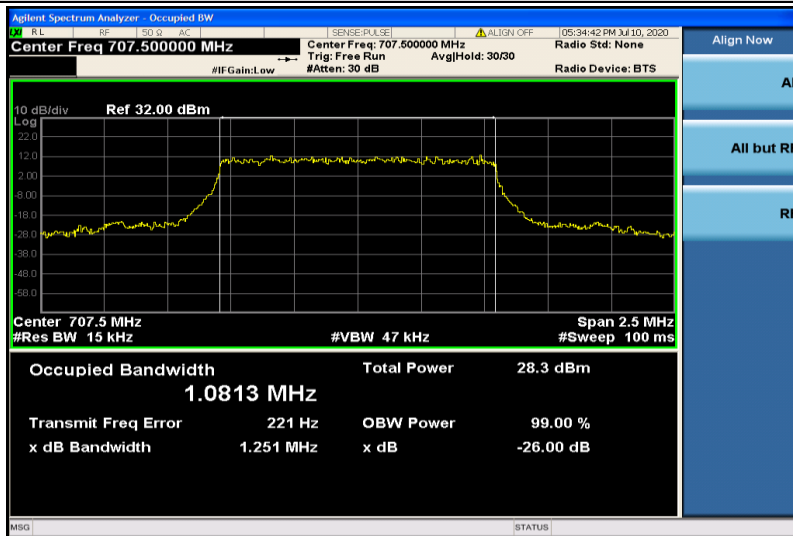
Band12-1.4MHz-QPSK-23095-6RB#0-1.0813
