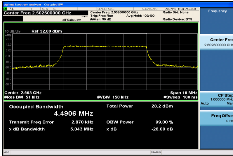
Band7-5MHz-16QAM-20775-25RB#0-4.4906
