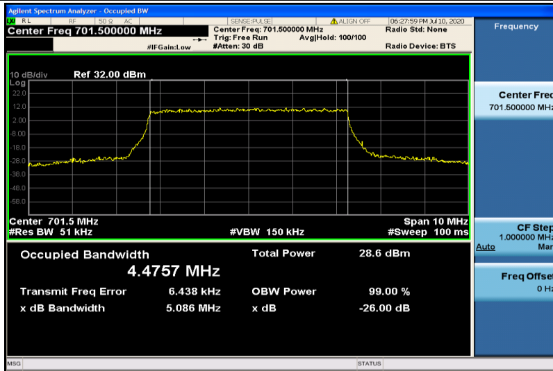
Band12-5MHz-16QAM-23035-25RB#0-4.4757
