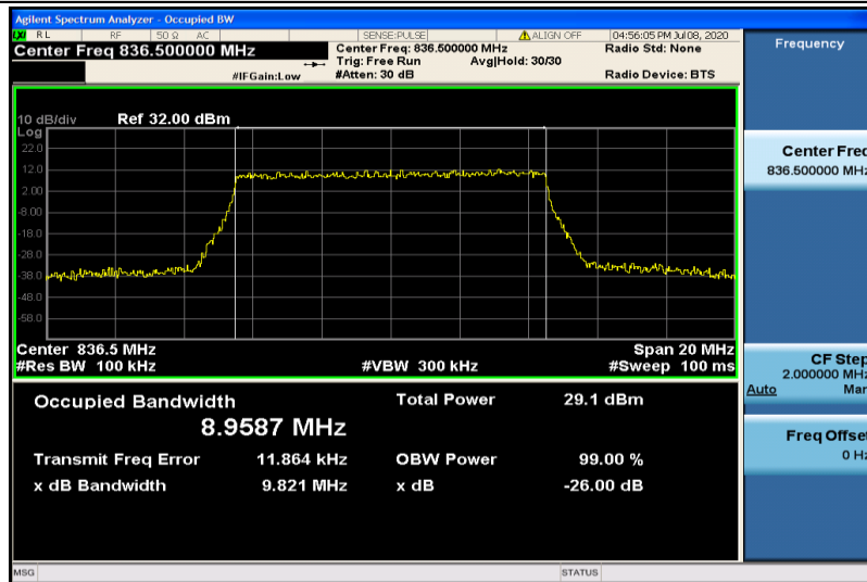
Band5-10MHz-QPSK-20525-50RB#0-8.9587
