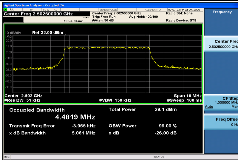
Band7-5MHz-QPSK-20775-25RB#0-4.4819
