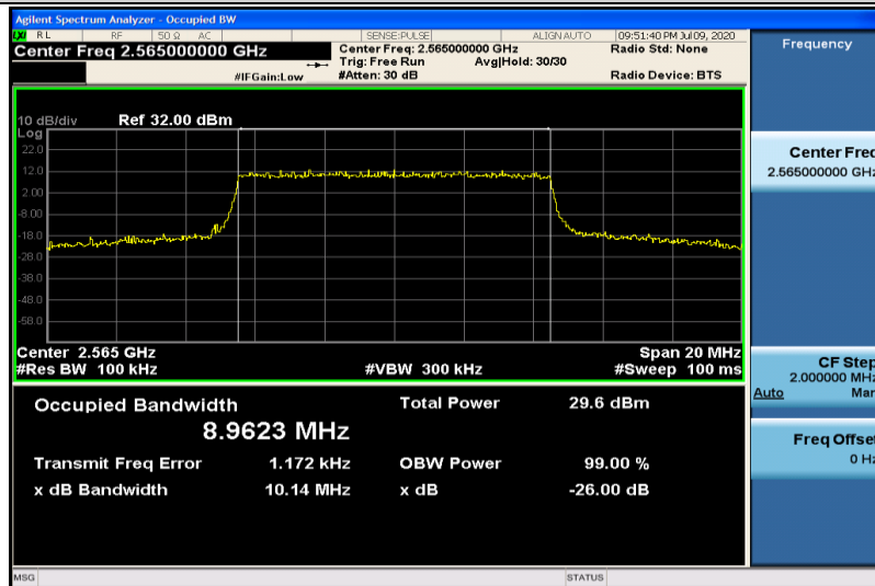
Band7-10MHz-QPSK-21400-50RB#0-8.9623
