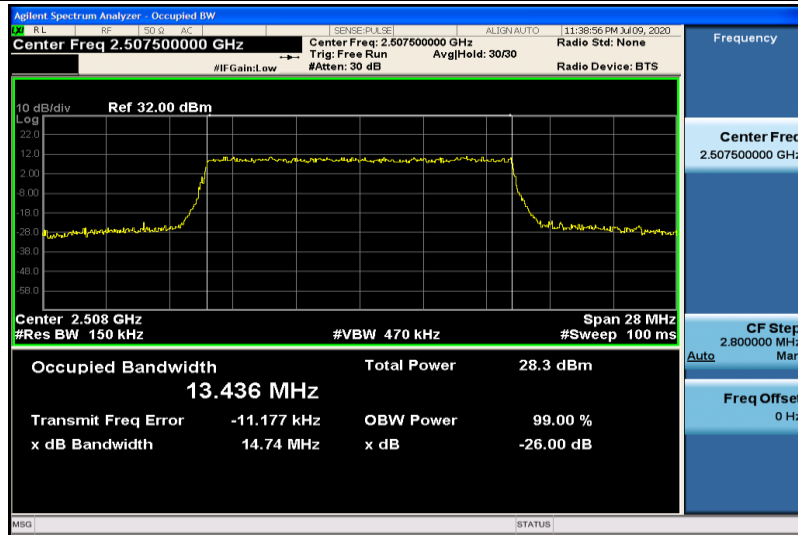
Band7-15MHz-16QAM-20825-75RB#0-13.436
